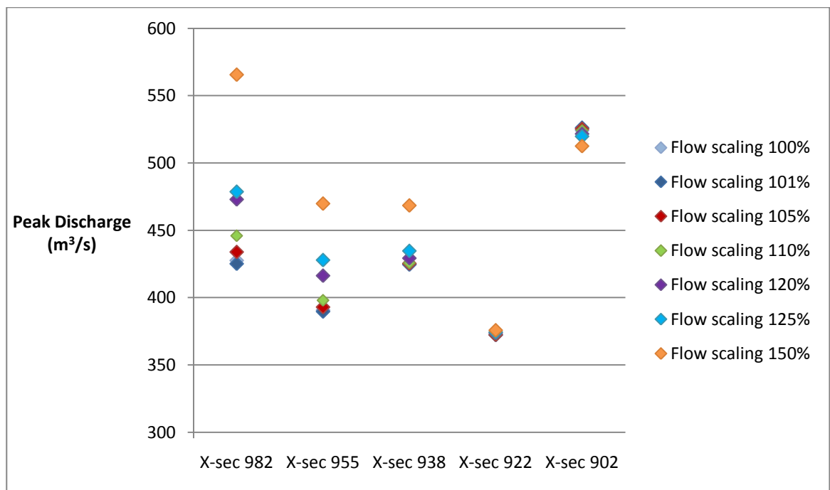
Figure 5.33 Peak discharge at selected cross section locations using the ‘with levées’ scenario for each of the scaled flows. The cross-section locations are from upstream to downstream in the reach (left to right on the graph). Cross-section locations are shown in Figure 5.2.
