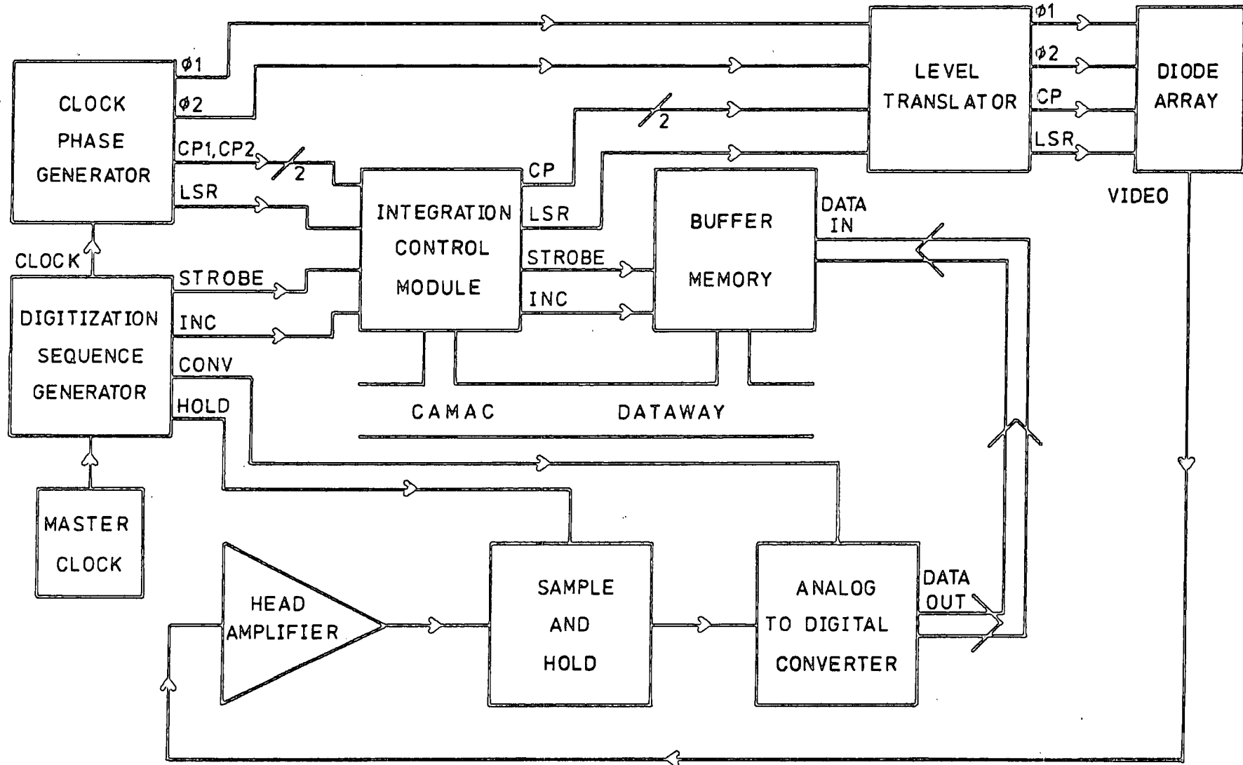
FIG. 3.21: DATA ACQUISITION AND CONTROL SYSTEM
