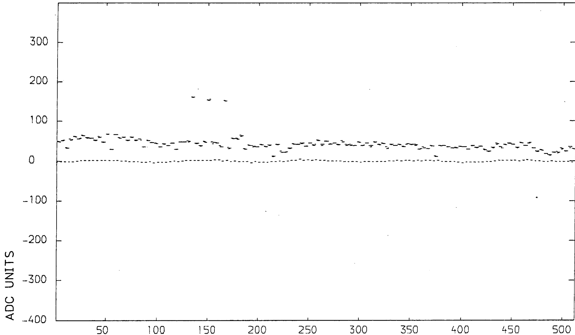
FIG.4.13: EXAMPLE OF FIXED PATTERN NOISE DIFFERENCE
