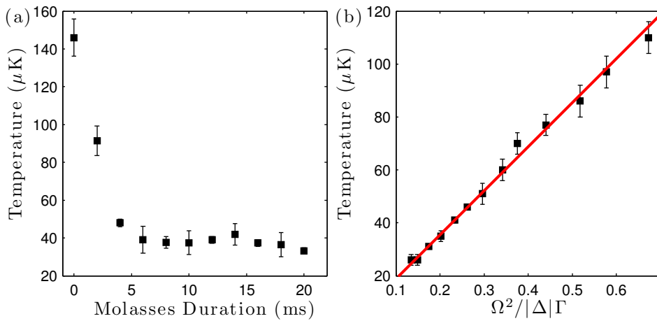
Figure 6.4: (a) Temperature vs. molasses duration for molasses temperature as a function of dimensionless light shift parameter \Omega^2/|\Delta|\Gamma . Fitting gives C_{\sigma+\sigma^-} = 0.58 \pm 0.02
