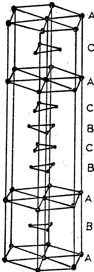
Samarium type
