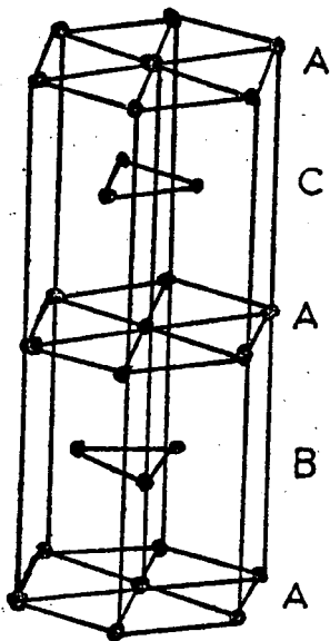
double hexagonal
