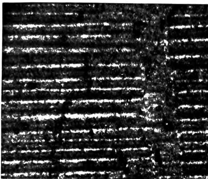
Fig. 7.31 (a) Domains in terbium at 215K Photograph shows a fine substructure (b) Domains in terbium at 95K Photograph shows light and dark contrast of domains due to vertical bias field (as discussed in text).
