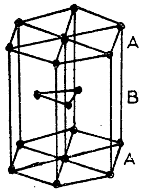
(e) hexagonal close - packed (h.c.p.)
