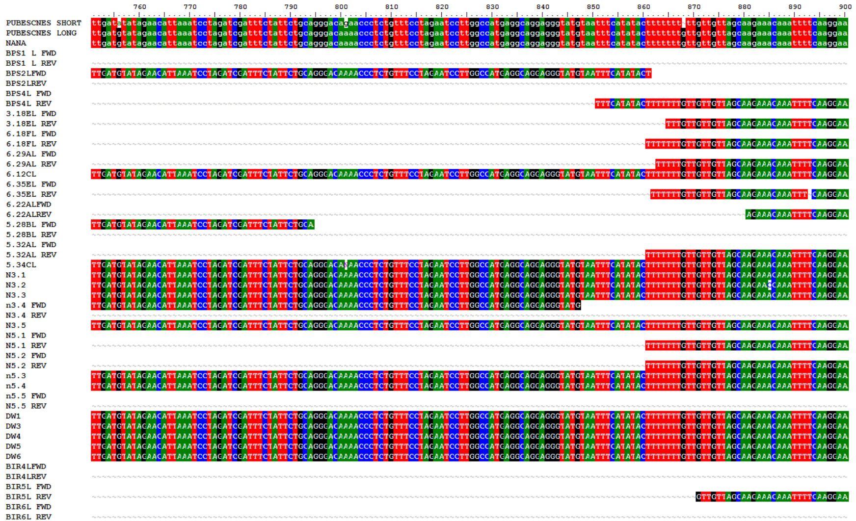
Fig. 3.2.3.19. Part 6. Full sequence of long alleles aligned with published long alleles and short allele.
