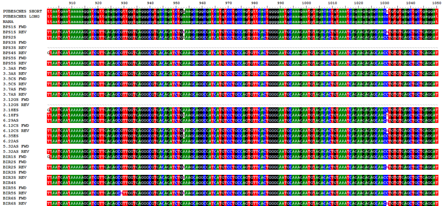
Fig. 3.2.3.9. Part 7. Full sequence of short alleles aligned with published long alleles and short allele.
