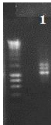
Fig. 3.2.2.7. TBE Gel image of PCR products using the ADH primer pair with DNA extracted from samples (1) BIR1.
