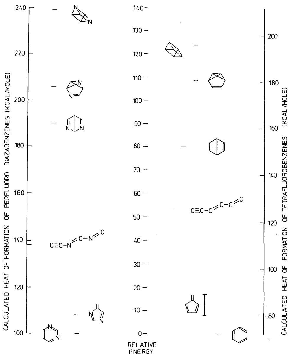
Figure 6.3 Heats of formation of the cations of the perfluoro 1,3-diazabenzene and some of the tetrafluorobenzene structural isomers.
