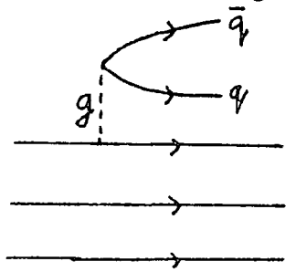
Figure 1.3 The Gluon-Induced Sea.
