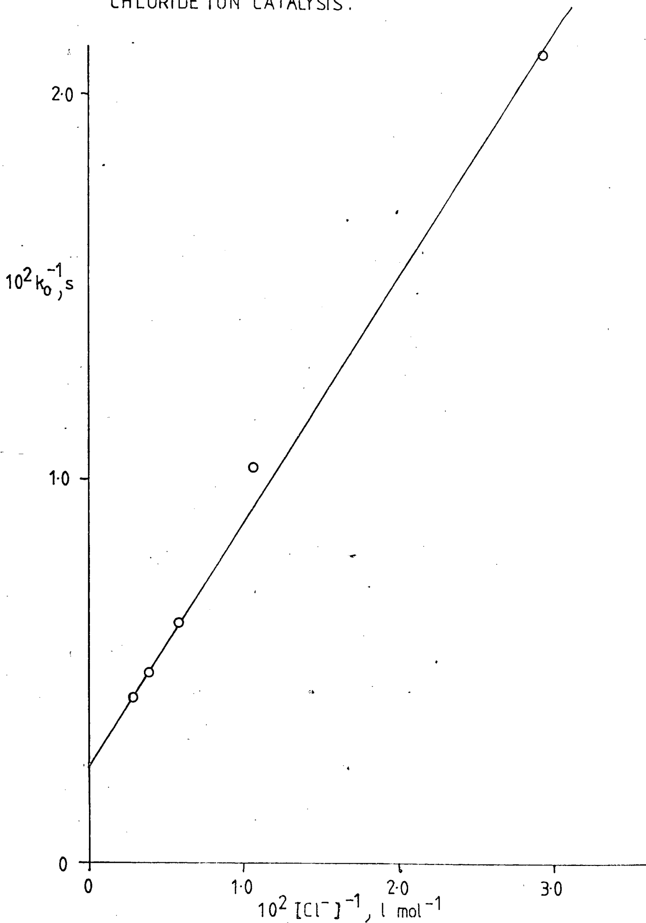
FIGURE 3 - NITROSATION OF NMA, CHLORIDE ION CATALYSIS.
