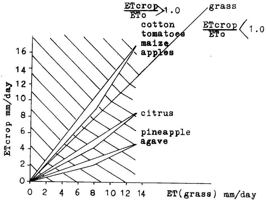
Figure 3.2 : ET_{crop} as compared to ET_o (After ref. 3.4)
