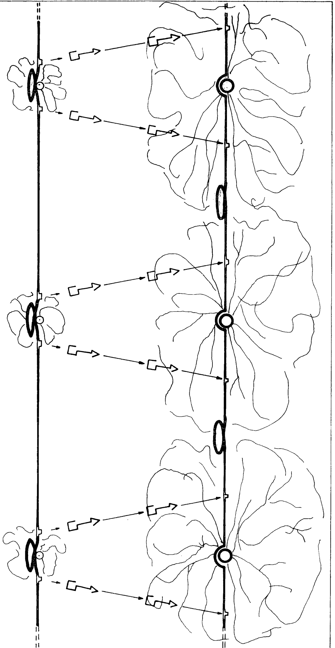
Figure 4.10: Emitter layout possibility and displacement from young to mature trees by forming loops.
