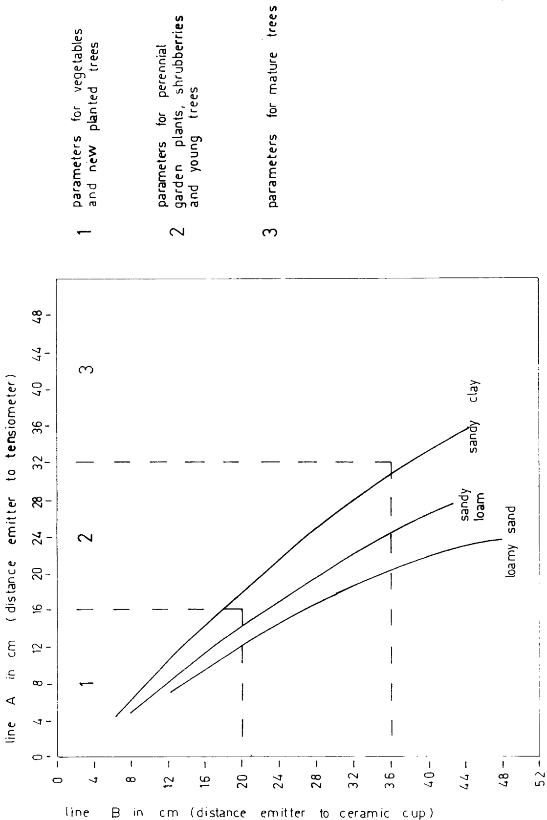
Figure 4.7: Guidelines for tensiometer placement for different kinds of soils and plants (Source: fieldwork)
