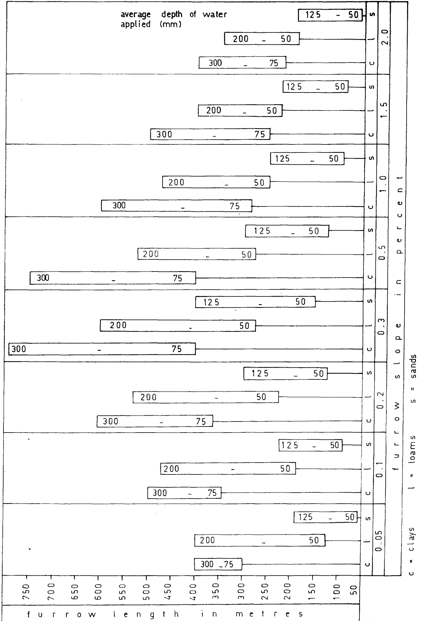
Figure 1.1: Suggested lengths of cultivated furrows for different soils, slopes and depths of water to be applied (After ref.1.3)
