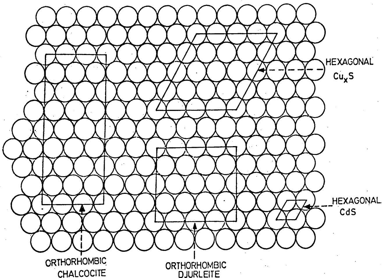
FIG.5-13(b) IDEALISED UNIT CELLS FOR THREE PHASES OF Cu_xS (FOR x \neq 2 ) SHOWING RELATIVE SIZE AND ORIENTATION IN THE BASAL PLANE OF HEXAGONAL CdS.
