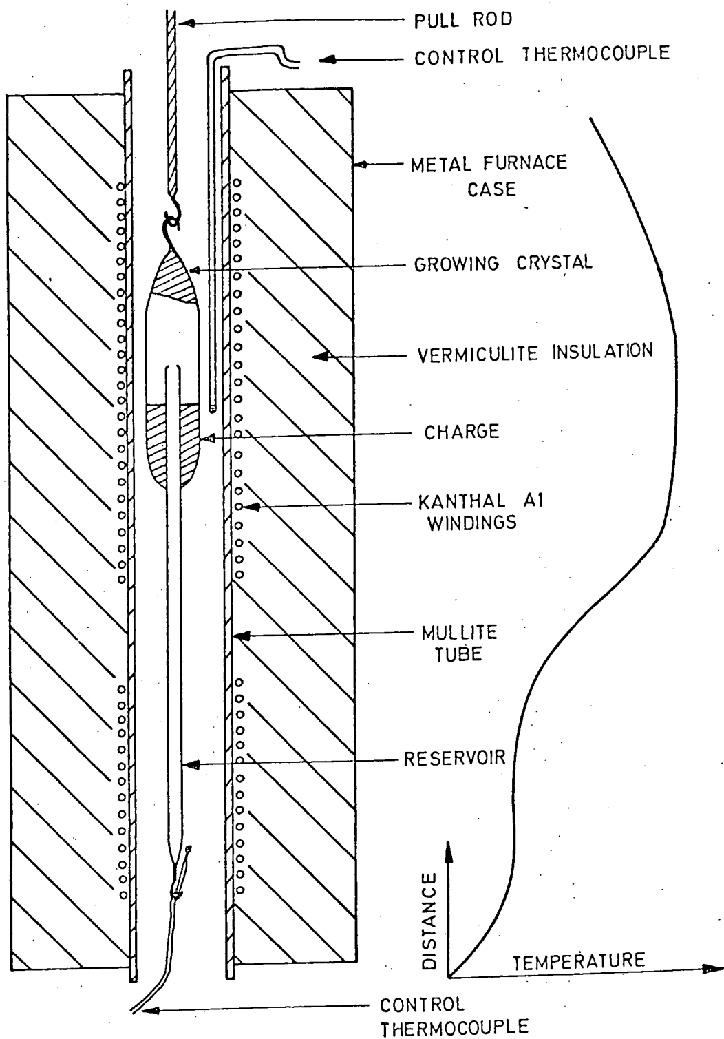
FIG. 4-1 EXPERIMENTAL ARRANGEMENT FOR THE GROWTH OF CdS AND (CdZn) 2 S SINGLE CRYSTALS FROM THE VAPOUR PHASE
