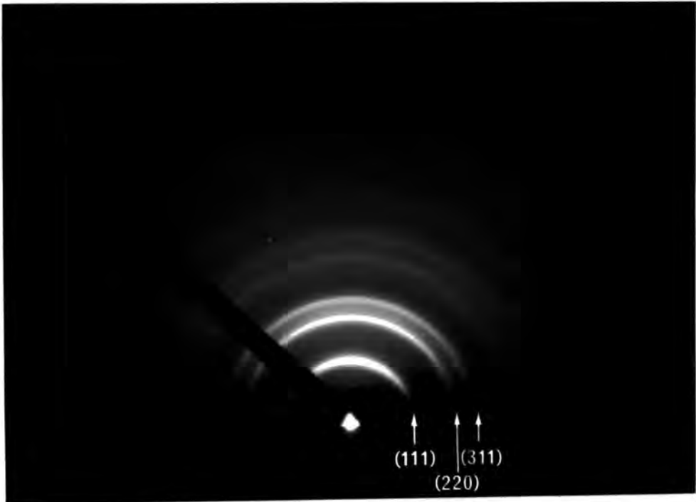
Figure 8.2 : Reflection electron diffraction pattern from the polished surface of a \text{Zn}_{0.3}\text{Cd}_{0.7}\text{S} crystal.
