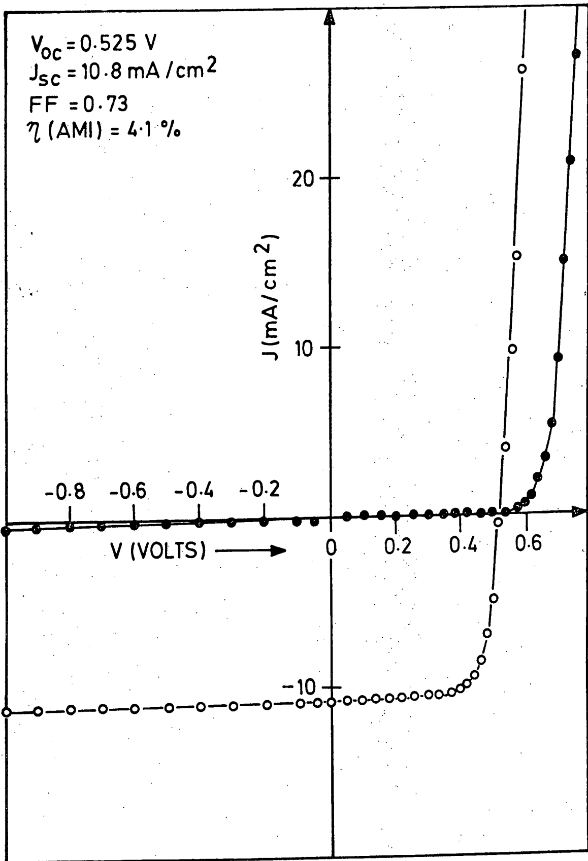
FIG.5-23. CURRENT VOLTAGE CHARACTERISTICS FOR TYPE A CELL AIR-BAKED AT 200^\circ\text{C} FOR 2 MIN, MEASURED IN THE DARK( \bullet )AND UNDER ILLUMINATION( \circ ).
