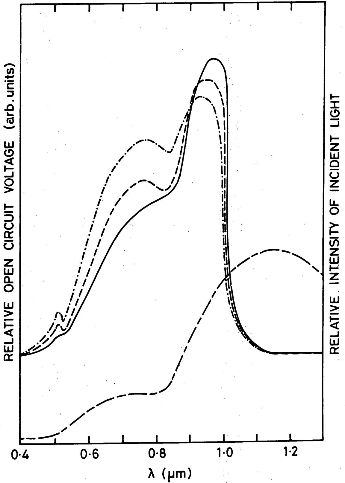
FIG.5-20. RELATIVE OPEN CIRCUIT VOLTAGES FOR AS-MADE \text{CdS}/\text{Cu}_x\text{S} CELLS CARRYING THE MIXTURE OF CHALCOCITE AND DJURLEITE
