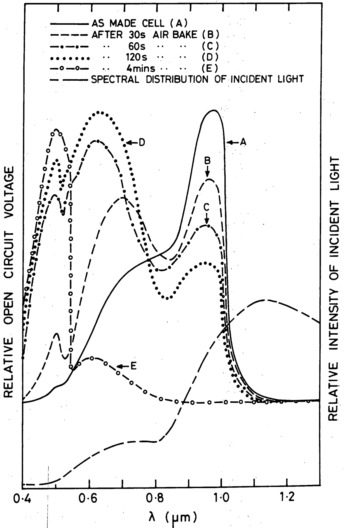
FIG.5.29. SPECTRAL DISTRIBUTION OF OPEN CIRCUIT VOLTAGE OF CdS/Cu x S CELL AS A FUNCTION OF HEAT TREATMENT
