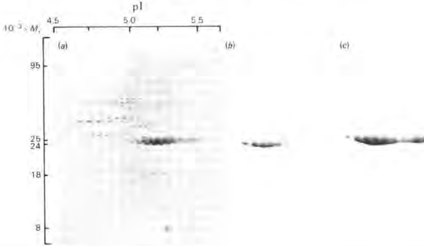
Fig. 4. Two-dimensional gel analyses of albumin proteins combining isoelectric focusing in urea gels in the first dimension and SDS/polyacrylamide-gel electrophoresis in the second dimension (a) Total seed albumin proteins; (b) small major albumin protein; (c) large major albumin protein.
