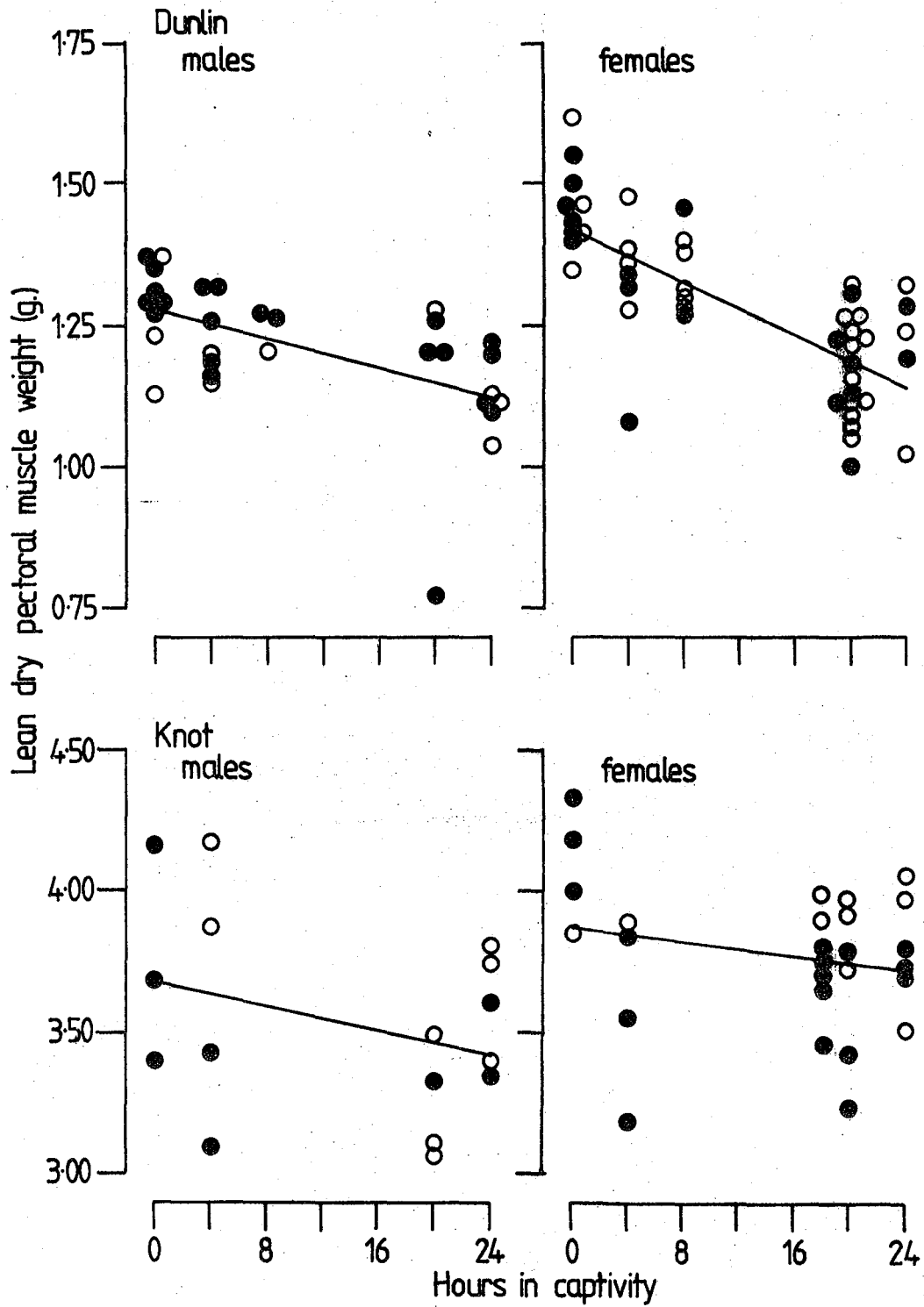
Figure 3: Loss of lean dry pectoral muscle weight by adult (●) and first-year (○) Dunlins and Knots from Teesmouth starved in captivity. Solid lines show least-squares regressions: Dunlin males r_{29} = -.56 , b = -.007 , P < .001 ; females r_{45} = -.75 , b = -.012 , P < .001 ; Knot males r_{14} = -.33 , b = -.011 , P > .10 ; females r_{25} = -.22 , b = -.006 , P > .10 .
