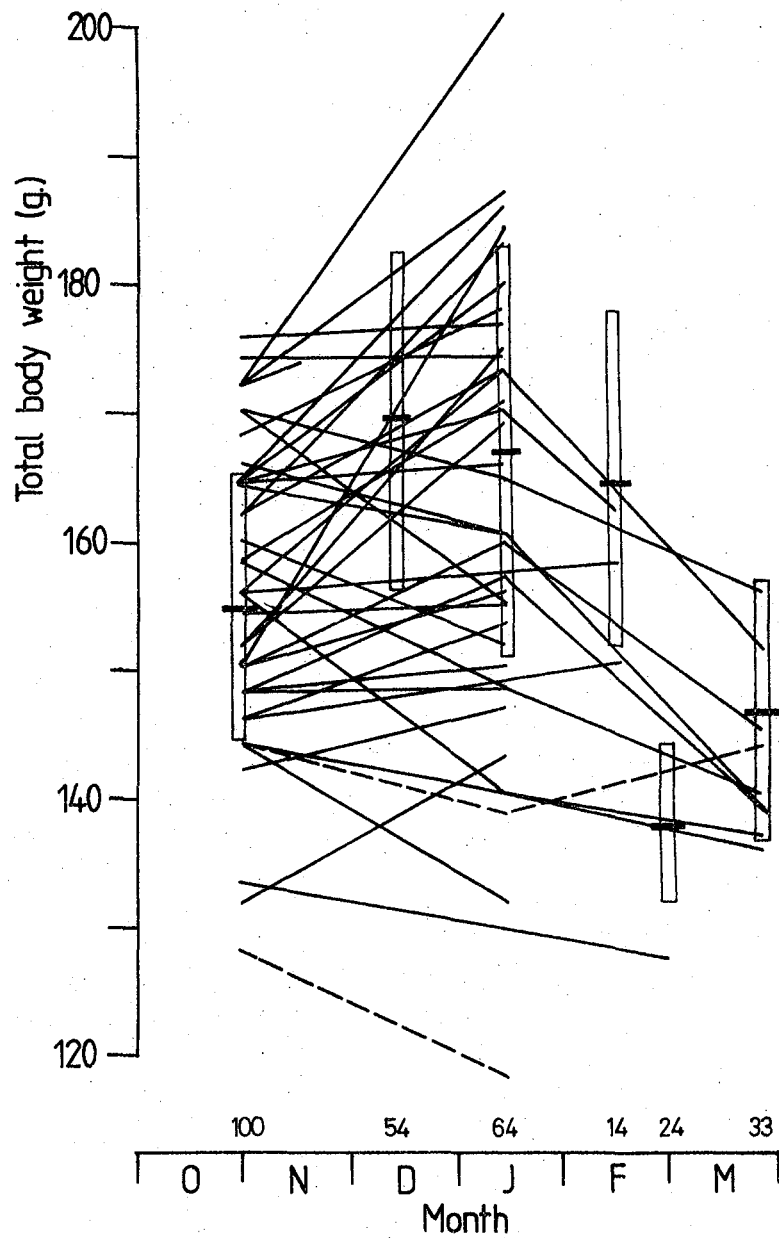
Figure 6: Total body weight changes of Redshanks caught more than once on the Firth of Forth during the 1979/80 winter. Solid lines join weights of each adult and dashed lines join weights of each first-year. For clarity, 20 adults and 6 first-years caught in October and March only are omitted. Open boxes show the mean \pm 1 standard deviation of all adult Redshanks weighed during the 1979/80 winter. Numbers indicate sample sizes.
