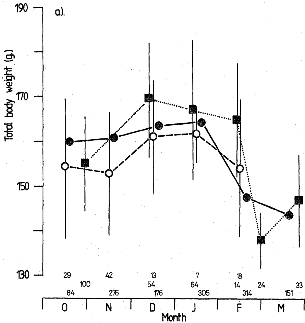
Figure 7: Total body weights of adult Redshanks wintering on various estuaries. a) on the Wash ( \text{---}\bullet\text{---} ) from Branson (1979), on the Firth of Forth in 1979/80 ( \text{.....}\blacksquare\text{.....} ) and at Teesmouth ( \text{---}\circ\text{---} ). Weights from the Wash and Teesmouth are grouped by month; weights from the Forth are plotted on date of capture, and b) presumed Icelandic ( \text{---}\blacktriangle\text{---} ) and Continental ( \text{---}\triangle\text{---} ) Redshanks on the Dutch Waddensee, from Smit and Wolff (1981). Each point is the mean \pm 1 standard deviation. Means only are shown for the Wash. Numbers indicate sample sizes.
