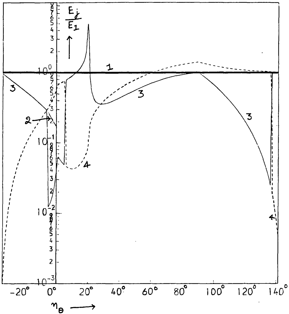
Figure 5.14(a) The normalised energy densities of the incident and reflected waves as functions of \eta_\theta for the case of the reflection from a conducting rigid boundary. \omega = 1.21 units for all these waves and n_\phi = -3.15^\circ .
