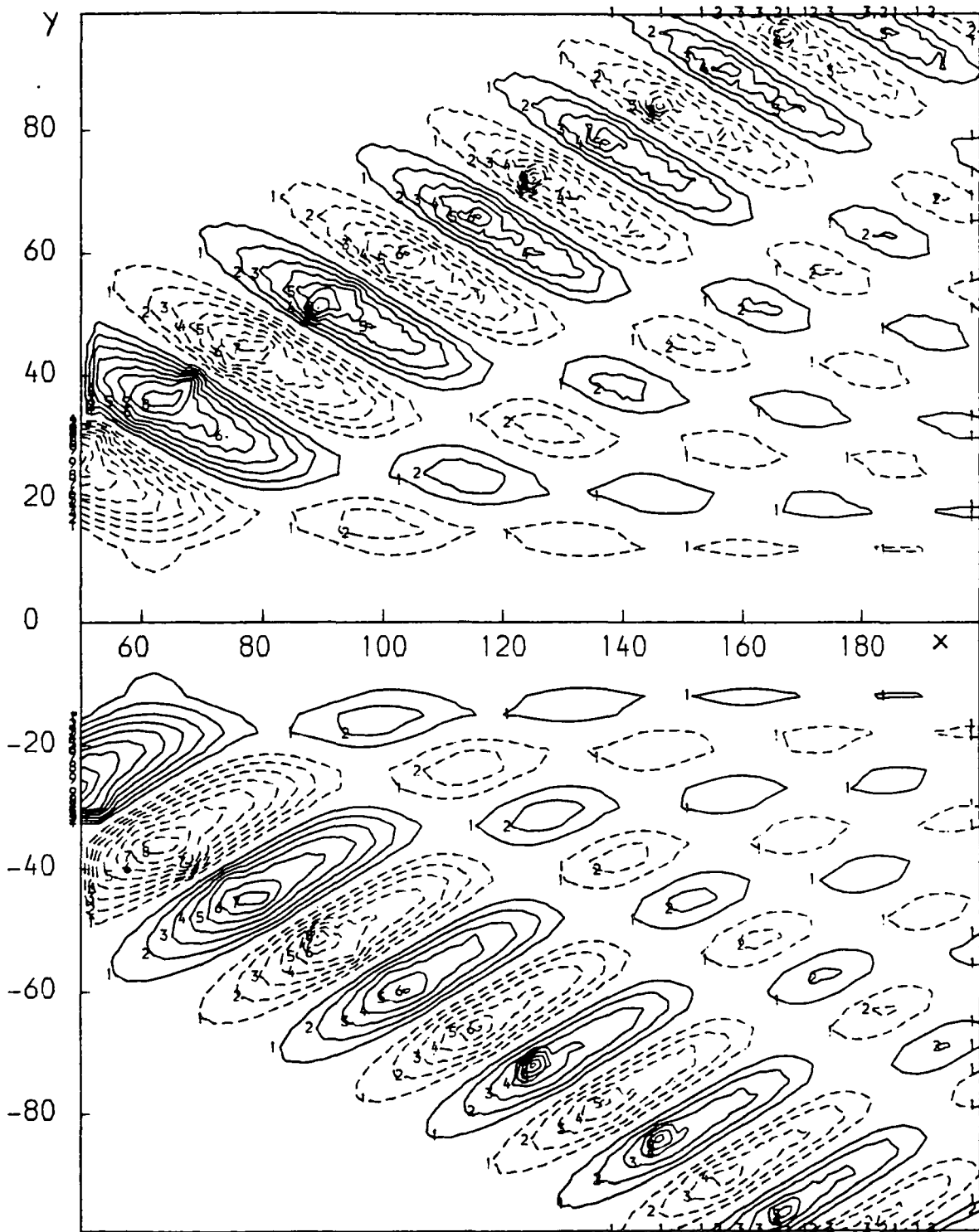
Figure 3.5 u(x,y,t) , the x-component of fluid velocity associated with the propagating disturbance. For other details see figure 3.4. Contour interval arbitrary.
