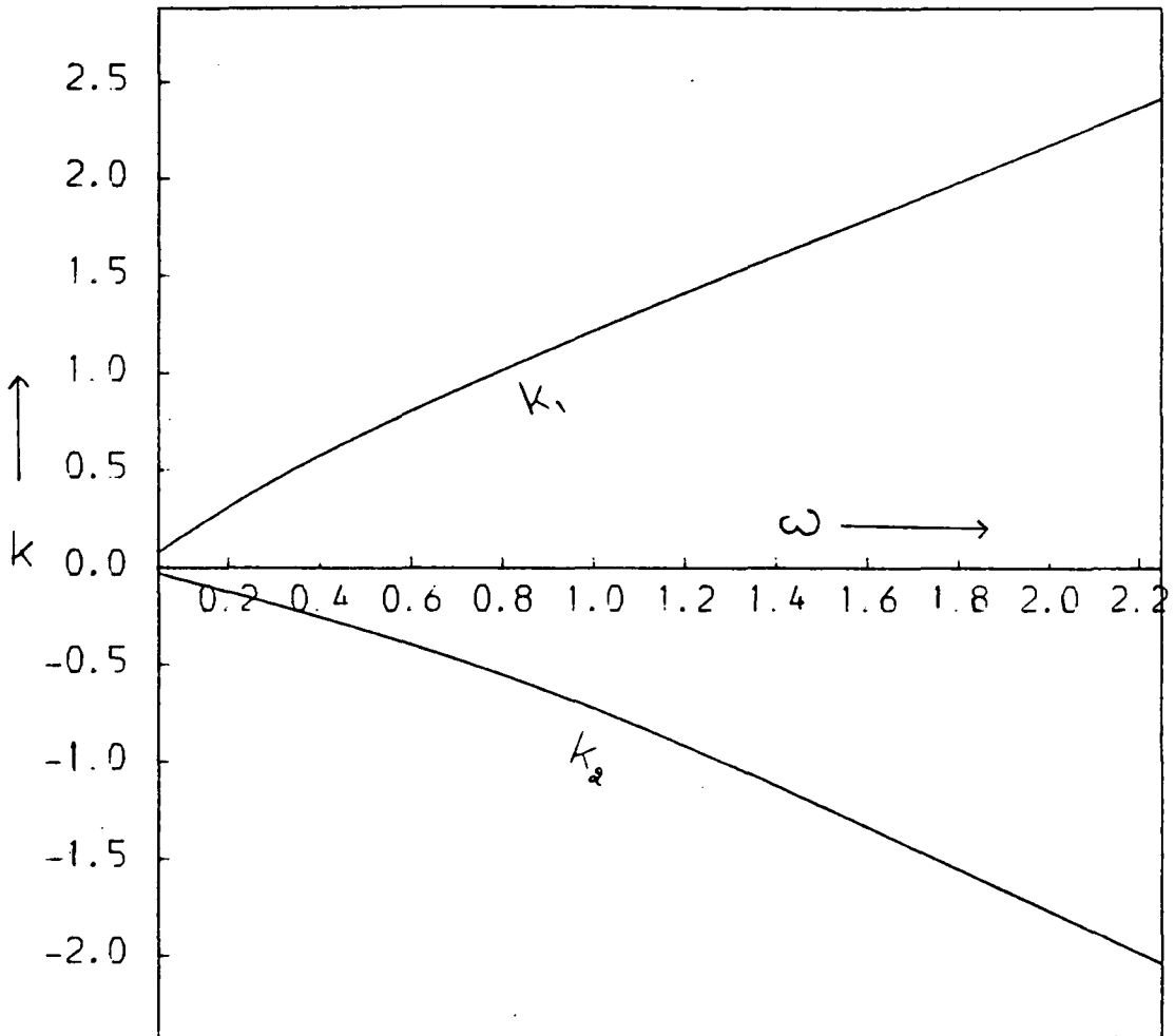
FIGURE 4.3(b) The incident and reflected wave numbers as functions of frequency. l = 1.0 . k_3 and k_4 are imaginary for all \omega .
