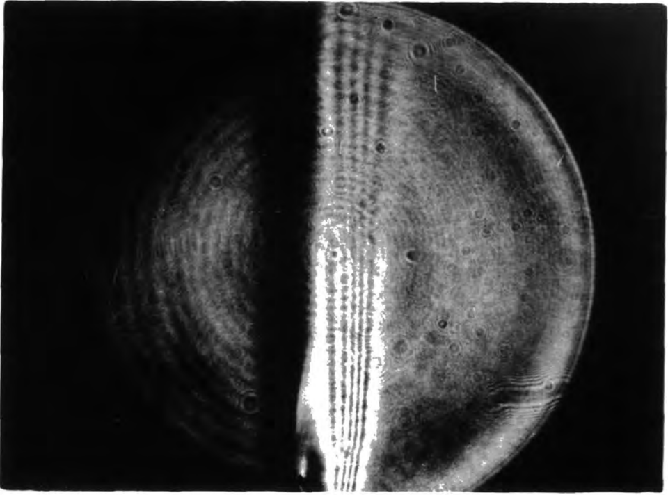
PLATE 2: Schlieren using razor blade cut-off
