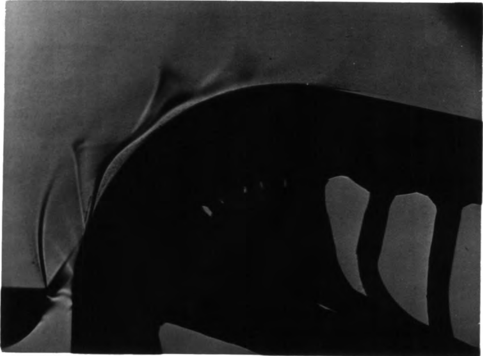
PLATE 10: Shadowgraph, Pa/Po = 0.267 Slot = 4 mm
