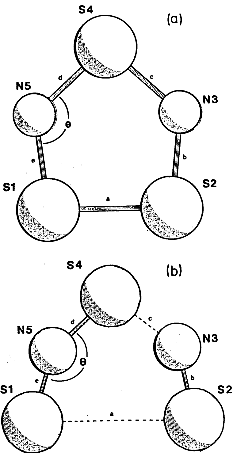
Figure 6.2. MNDO optimised geometry of the S_3N_2^+ ring. a) equilibrium geometry; b) calculated geometry for d \text{ S-S} = 3.3 \text{ \AA} .
