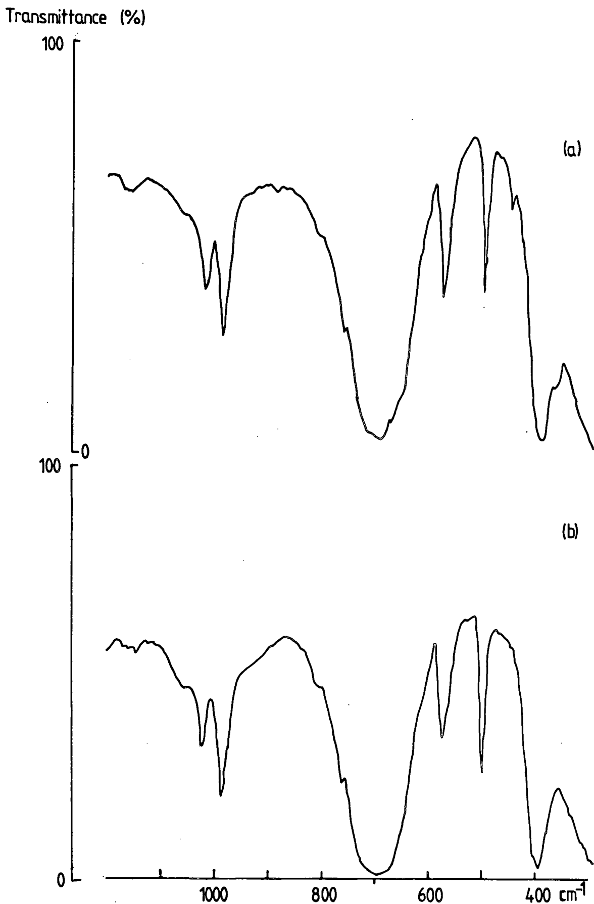
Figure 6.1a. Infrared spectra of \text{S}_3\text{N}_2\text{F}^+\text{AsF}_6^- , a) prepared from \text{S}_2\text{N}^+\text{AsF}_6^- and \text{CsF} ; b) prepared from \text{S}_3\text{N}_2^{2+}(\text{AsF}_6^-)_2 and \text{CsF} .
