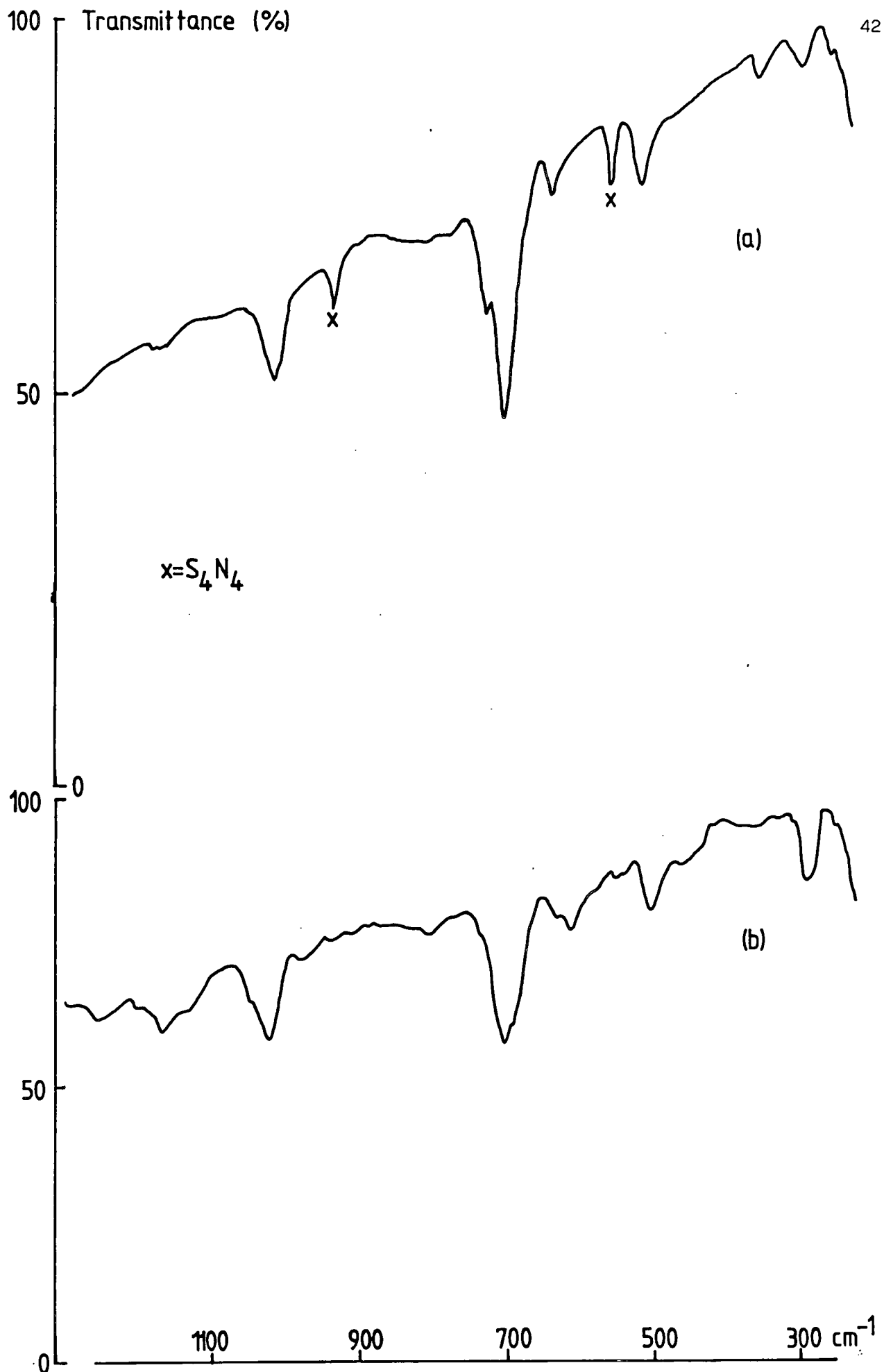
Figure 3.1. Infrared spectra of (SN)_x (nujol mull, CsI plates). a) Classical (SN)_x contaminated with a little S_4N_4 (supplied by Dr Z.V. Hauptmänn) b) Product from the reaction between S_5N_5Cl and K_2CS_3
