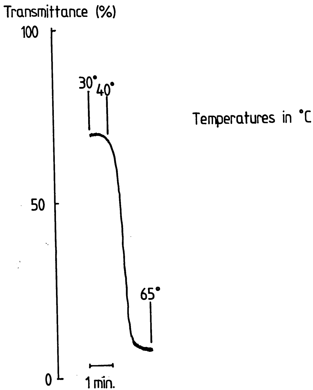
Figure 5.2. Evolution of NSF with increasing temperature.
