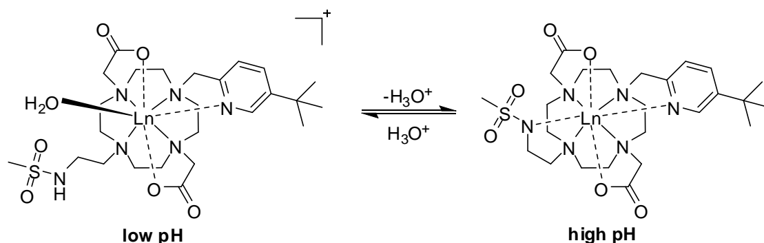
Scheme 5.7 Design of the pH-responsive probe, [Ln.L 11 ].
