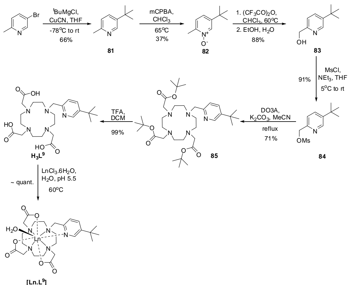
Scheme 5.3 General procedure for the synthesis of [\text{Ln}.L^9] .
