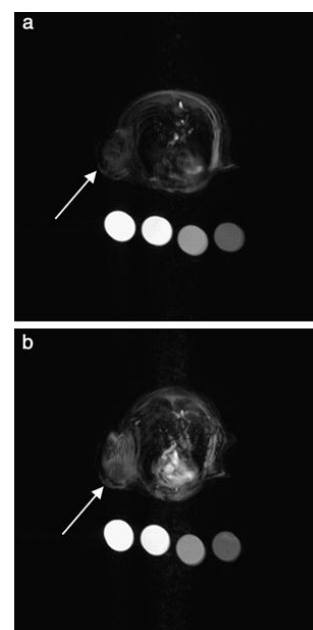
Figure 1.18 Chemical structure of anionic block copolymer reported by Yokoyama and co-workers and T_1 -weighted MR images of axial slices (a) before and (b) 24 h after injection at dose of 0.05 mmol Gd/kg. Arrow indicates the tumour and circles are stock solutions of (left to right) 1.0 mM, 0.5 mM, 0.1 mM, and 0 mM Gd(III) ion in agarose gel. 106
