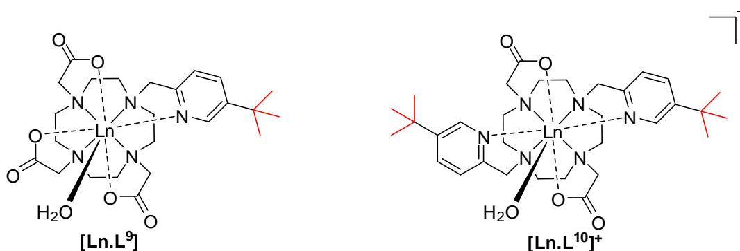
Scheme 5.4 Comparison between the chemical structure of [\text{Ln.L}^9] , and [\text{Ln.L}^{10}]^+ .
