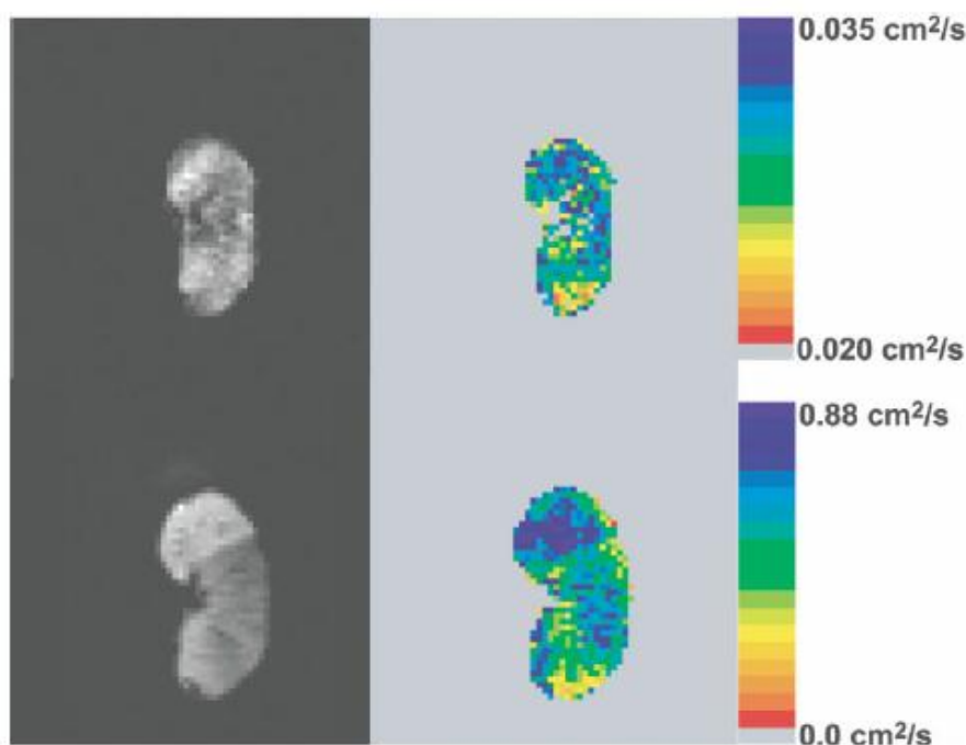
Figure 1.6 Comparison of C_2F_6 (top row) and hyperpolarised ^3He (bottom row) gradient-echo spin density images (left) and apparent diffusion coefficient maps (right) of a formalin-fixed emphysematous lung. 45
