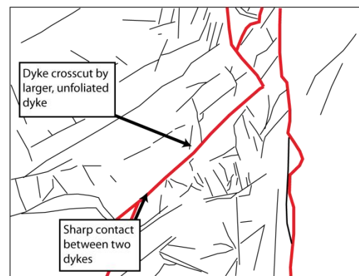
Figure 5.66C (top, right) The dyke is cut by a larger, NNE-SSW trending dyke. Could the foliated dyke represent a much older magmatic event than the other syn-rift dykes? seen
