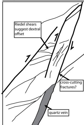
Figure 5.61C. Apparent dextral kinematics of fractures in the granite at F1a, away from the dyke. A quartz vein trends parallel to one of these structures, suggesting they may have been formed during a hydrothermal event. The sense of deformation on these structures has been derived from their geometry, and that of the smaller conjugate fractures between them.
