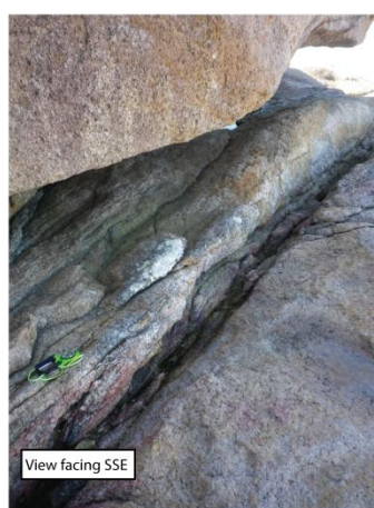
Figure 5.61A. NNE-SSW trending en-echelon fractures within the granite at Praia Galhetas. These individual fractures do not accommodate any apparent offset, but their geometry suggests dextral kinematics.
