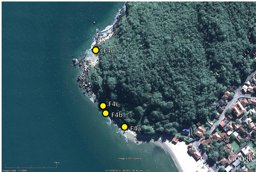
Figure 5.69. A Google earth aerial image of the outcrop at Ponta das Canas, showing localities visited (yellow circles).
