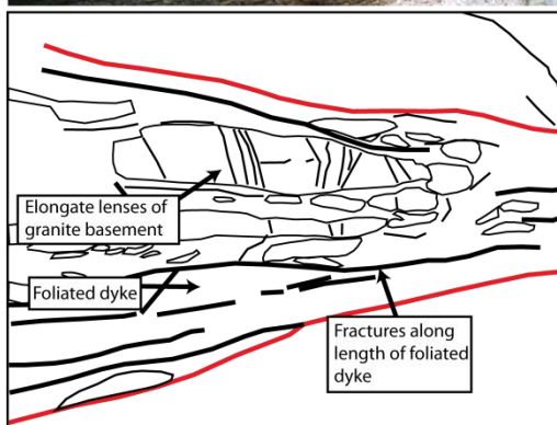
Figure 5.66A (top, middle). The sheared dyke locality at Praia Joaquina, showing the large amounts of fracturing in the granite.
