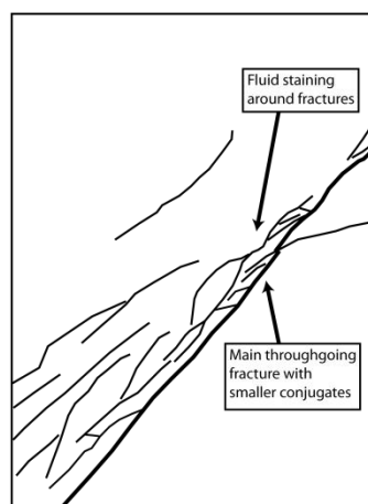
Figure 5.61B. This fault consists of a series of lenses of granite within a larger structure. The fractures within the fault are stained red, and trend at a high angle to the dyke margin. No evidence can be seen of this particular fault cutting the dyke.
