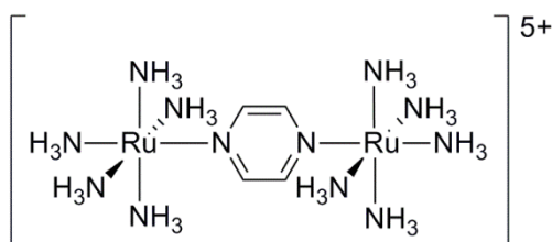
Figure 1.9. The Cruetz Taube ion.
