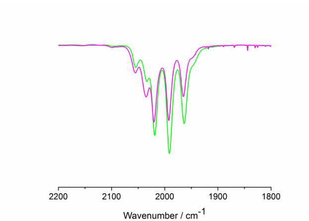
Figure 5.18. The IR \nu(\text{C}\equiv\text{O}) spectra [41c]PF 6 (green), [41c][PF 6 ] 2 (purple) obtained by stoichiometric oxidation of 41c with two equivalent of [FcAc]PF 6 in CH 2 Cl 2 at -40 °C.
