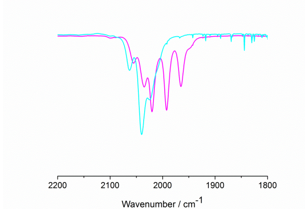
Figure 5.19. The IR \nu(\text{C}\equiv\text{O}) spectra of [41c][PF 6 ] 2 (purple) and [41c][PF 6 ] 3 (blue) obtained by stoichiometric oxidation of 41c with three equivalents of [FcAc]PF 6 in CH 2 Cl 2 at -40 °C.
