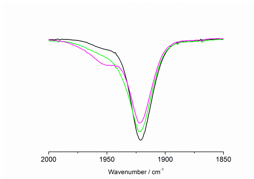
Figure 4.11. IR spectra for 20 (black), [\mathbf{20}]^+ (green) and [\mathbf{20}]^{2+} (purple) collected during an in situ oxidation in an IR spectroelectrochemical cell in 0.1 M \text{NBu}_4\text{PF}_6 / \text{CH}_2\text{Cl}_2 .
