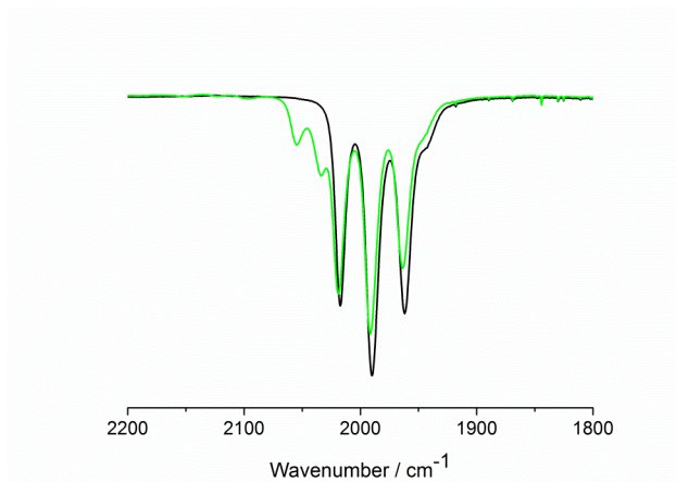
Figure 5.17. The IR \nu(\text{C}\equiv\text{O}) spectra of 41c (black), [41c]PF 6 (green) obtained by stoichiometric oxidation of 41c with one equivalent of [FcAc]PF 6 in CH 2 Cl 2 at -40 °C.
