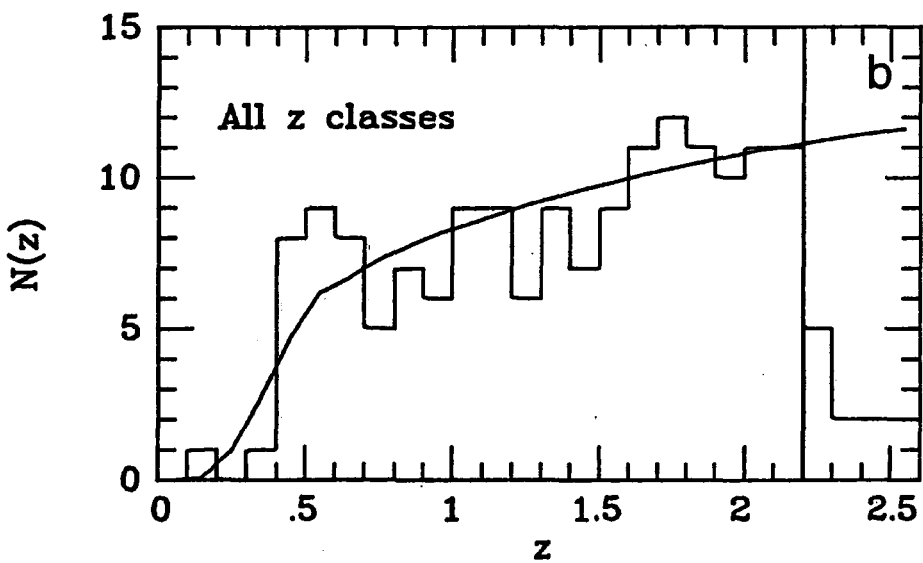
Figure 4.7 Number redshift relation for a) redshift class 1 and 2 and b) all redshift class QSOs discovered in the faint spectroscopic survey. Solid line indicates prediction of the standard evolution model (see text).
