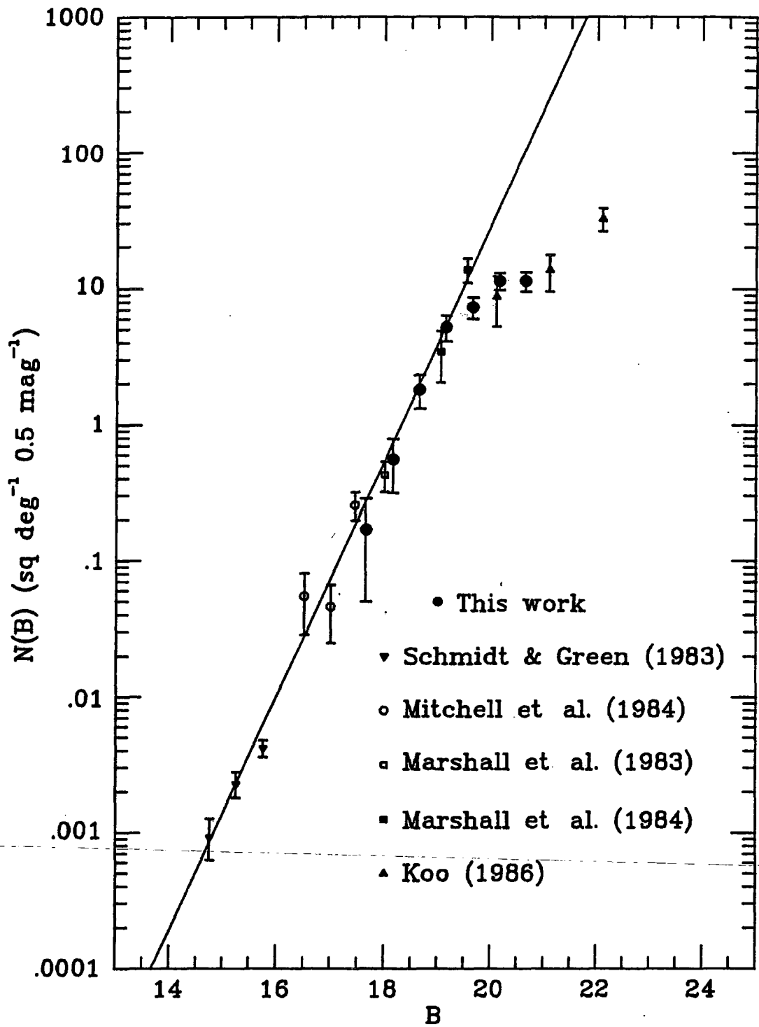
Figure 4.3 Differential number magnitude counts for z < 2.2 QSOs. Solid line indicates Braccési et al. (1980) power law relation.
