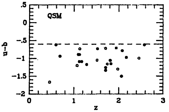
Figure 3.8 u-b vs z for redshift class 1 and 2 QSOs discovered in the faint UVX survey. Dashed lines denote the UVX limits applied on each field. • denote b < 20 mag QSOs, ○ b > 20 mag QSOs, ■ b < 20 mag BAL QSOs, ◻ b > 20 mag BAL QSOs.
