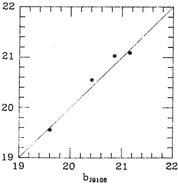
Figure 2.7 Galaxy Calibration a) QNA field b) QSN field (see text for details).
