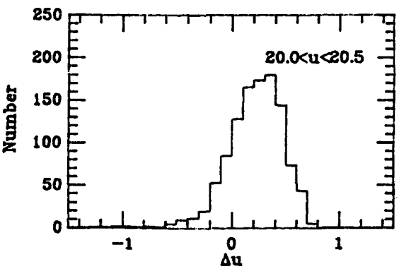
Figure 2.9 c) Number \nu \Delta u ( u_{5707} - u_{9218} ): QNY field.
