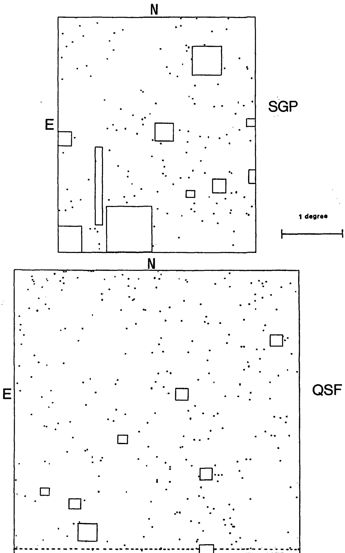
Figure 6.1 Distribution of UVX objects ( 18 \text{ mag} < b < 20 \text{ mag} ) on all fields used in the correlation analysis. Dashed lines indicate the areas over which clustering analysis took place.
