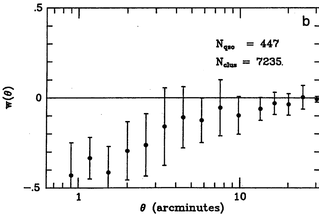
Figure 6.6 Cluster galaxy/emission line object cross-correlation function. a) Individual field cross-correlation function. b) Pair-weighted average cross-correlation function. See figure 6.5 for key to symbols
