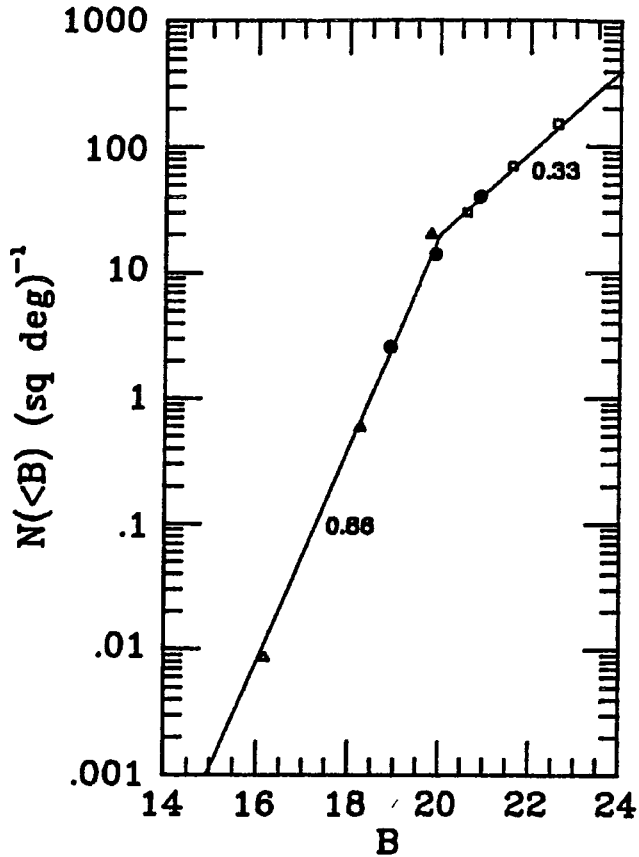
Figure 6.14 Integral n(<B) relation for spectroscopically confirmed QSOs. \triangle Schmidt and Green (1983), \blacktriangle Marshall et al. (1984), \square Koo (1986), \bullet this work.
