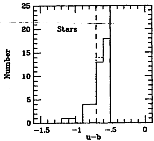
Figure 4.2 continued b) QNY, QNA and QSM fields.
