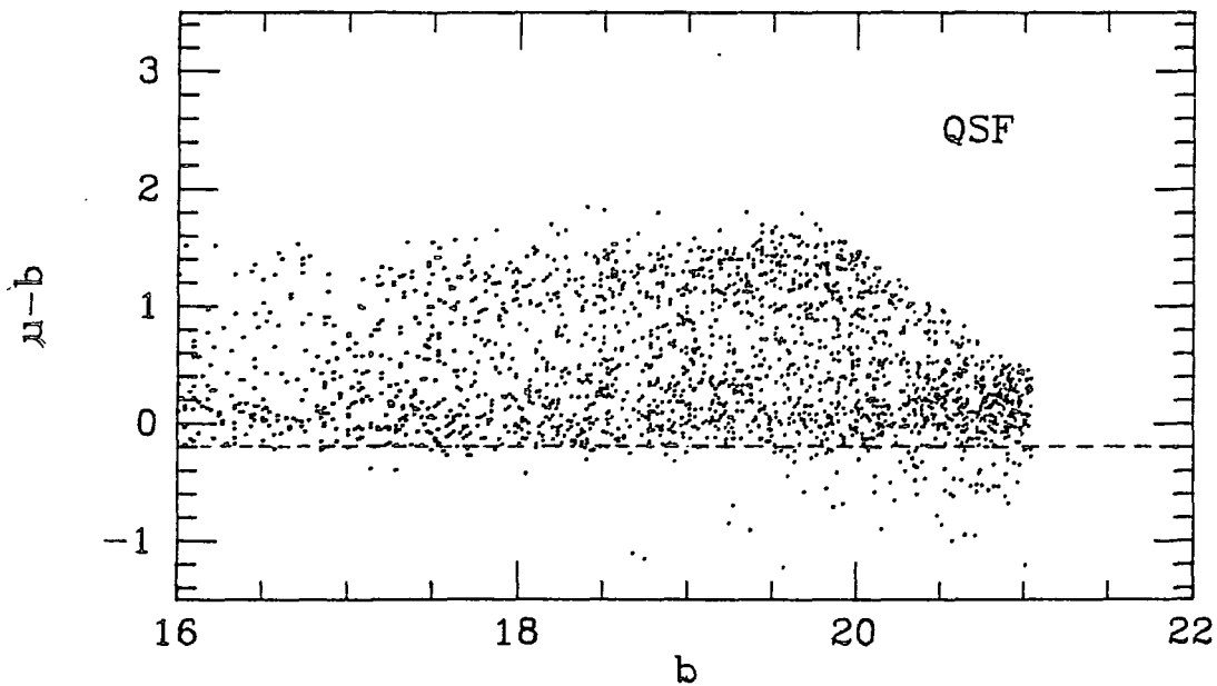
Figure 2.5 u-b vs b diagrams for stellar images in central 1 square degree areas on each field observed in the faint spectroscopic survey. Dashed lines indicate UVX limits used for the faint spectroscopic survey. a) SGP and QSF fields.
