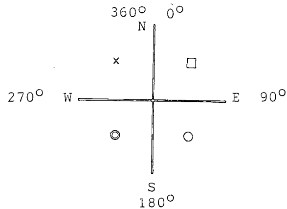
Fig A5ii Teesmouth average daily wind speed (knots) 0000 - 2400 hrs, showing daily maximum gust - when this exceeded 34 knots (gale force 8 or greater) - and principle wind direction (courtesy of the Meteorological Office, Newcastle-upon-Tyne)
