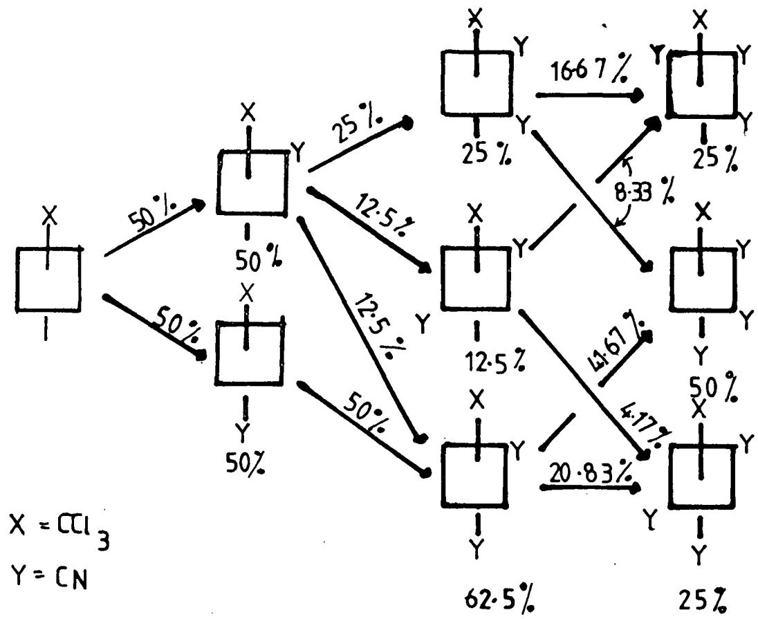
Fig. 6.7 STATISTICAL PATTERN OF SUBSTITUTION IN THE [\text{CCl}_3\text{PCl}_{5-n}(\text{CN})_n]^- DERIVED FROM EXPERIMENTAL DATA.
