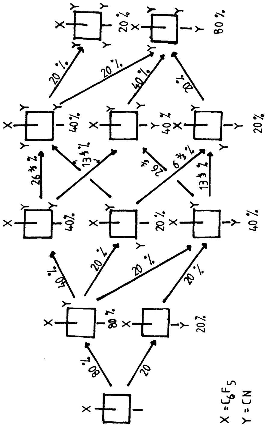
Fig. 6.4 : STATISTICAL PATTERN OF SUBSTITUTION IN THE C_6F_5PCl_5/CN^- SYSTEM
