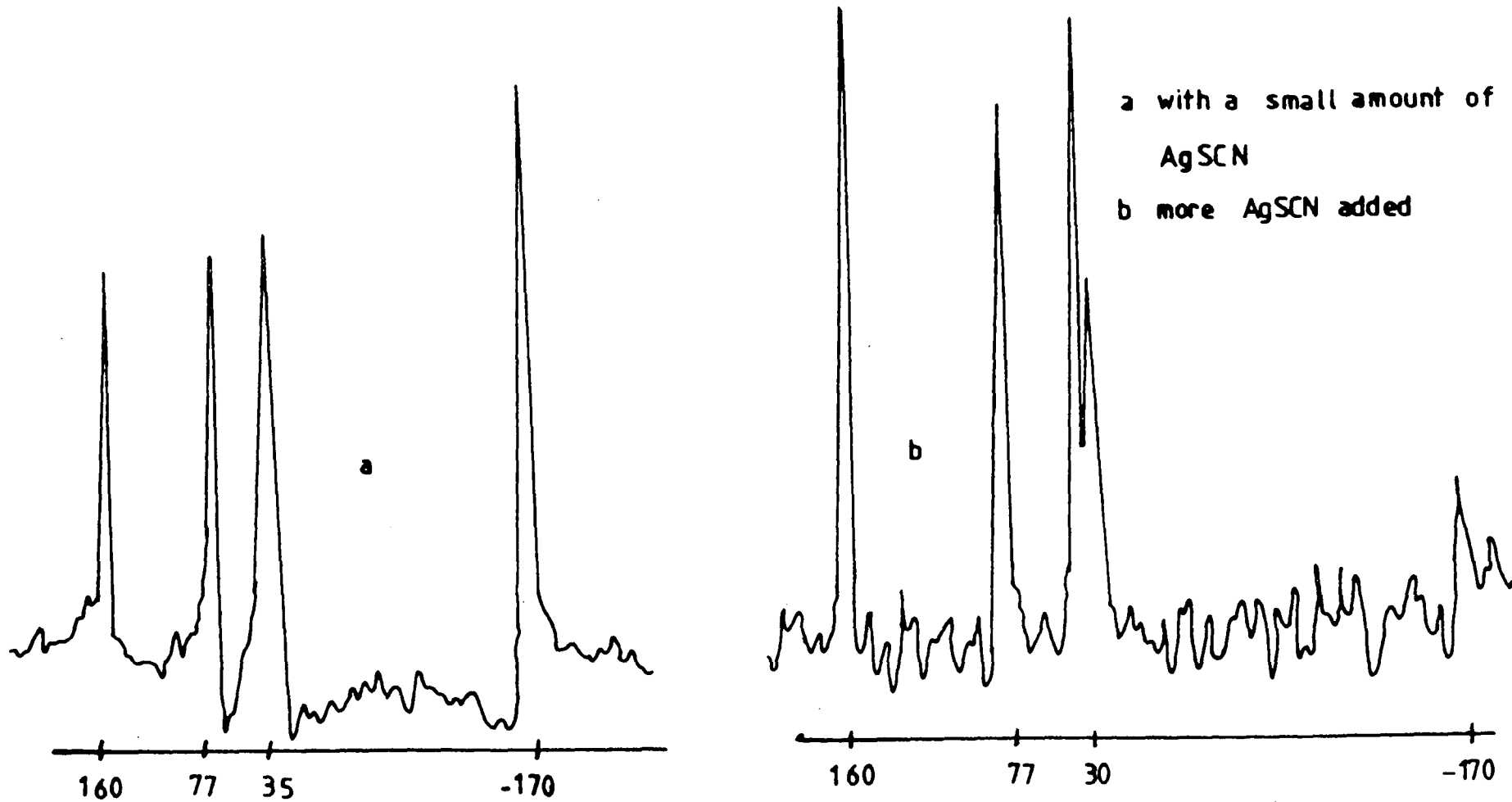
Fig. 6.3: ^{31}\text{P} NMR SPECTRA FOR \text{Et}_3\text{NPhPCL}_2 / \text{SCN}^- SYSTEM
