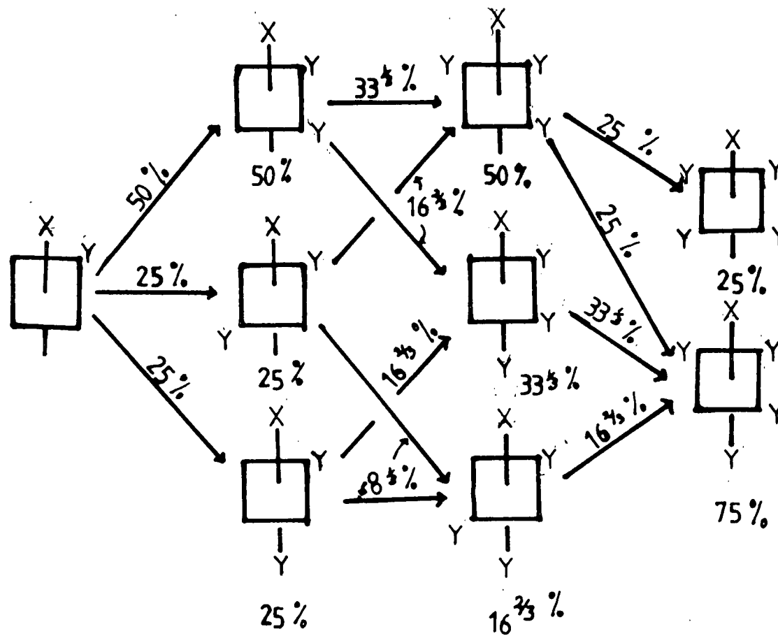
Fig. 6.5: STATISTICAL PATTERN DERIVED FROM EXPERIMENTAL DATA FOR [C_6F_5PCl_4(CN)]^- .
