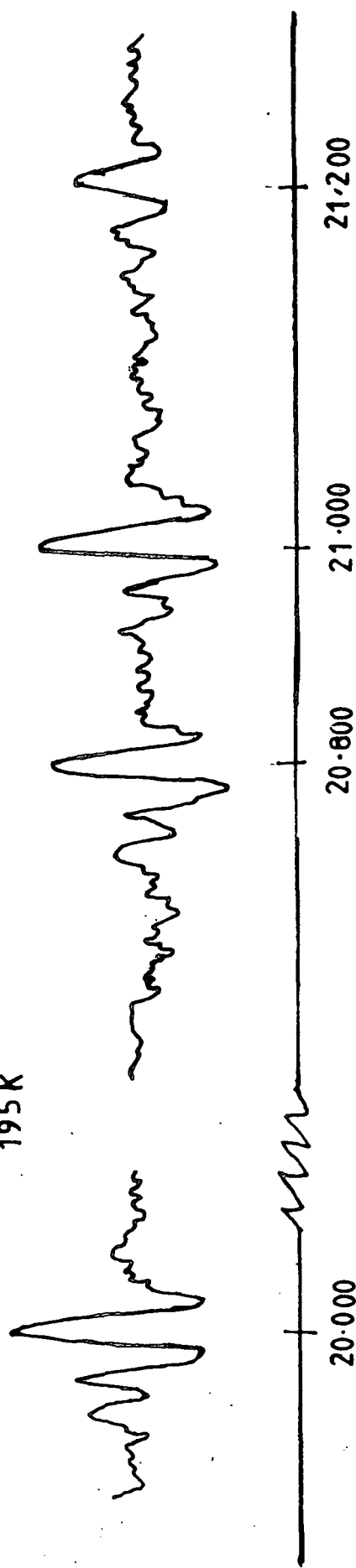
Fig. 34: ^{35}\text{Cl} n.q.r. spectra for \text{BCl}_4^- in \text{C}_6\text{F}_5\text{PCl}_3\text{BCl}_4
