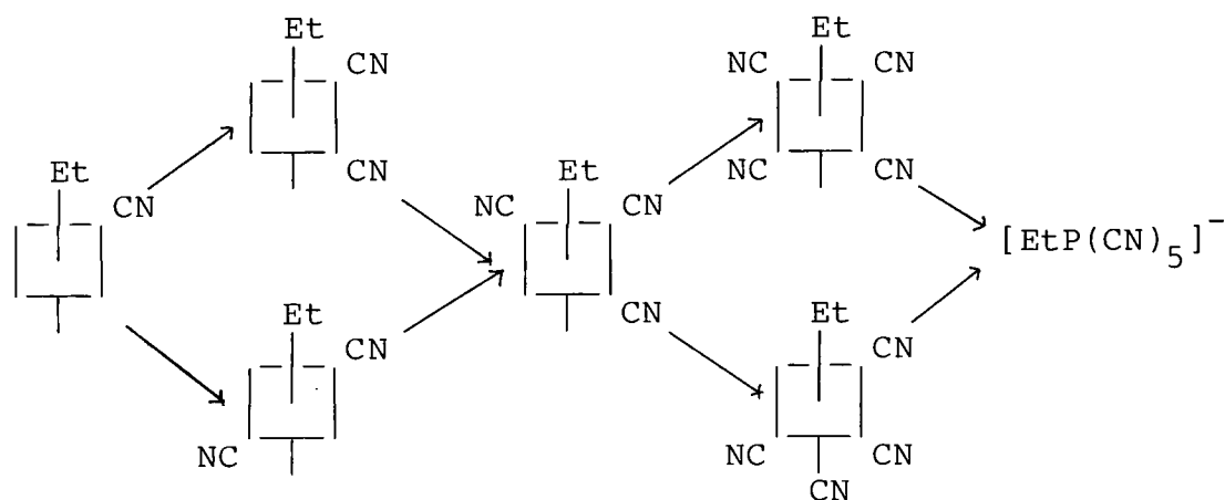
Fig.6.6: Pattern of substitution in the [\text{EtPCl}_{5-n}(\text{CN})_n]^- system derived from experimental data.
