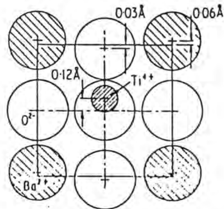
Figure 4 : The Atomic Positions in Tetragonal \text{BaTiO}_3
