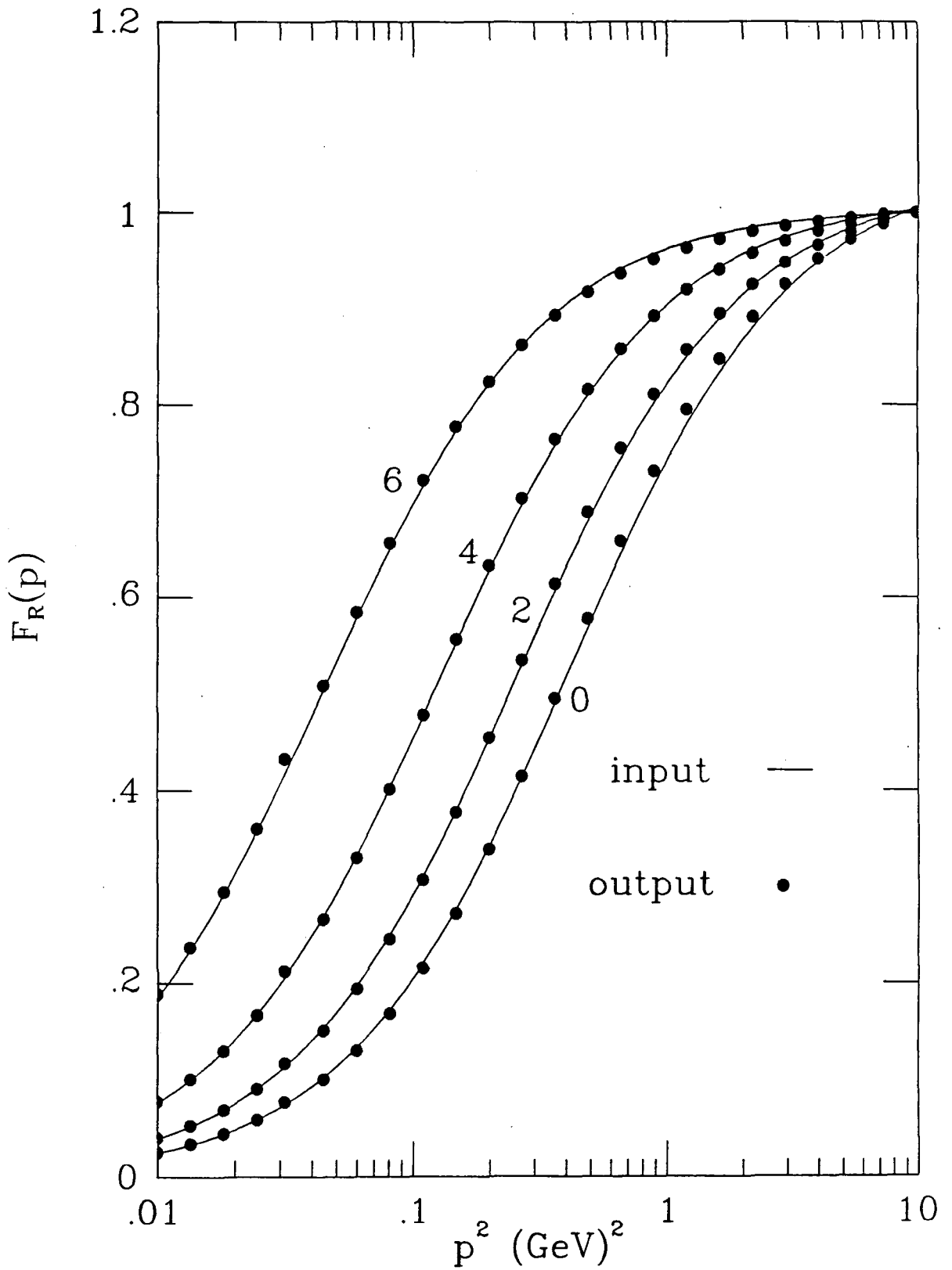
fig. 6.9: The quark renormalisation function \mathcal{F}_R(p) as a function of p^2 for \alpha(\mu) = 0.3 , with n_f = 0, 2, 4, 6 .
