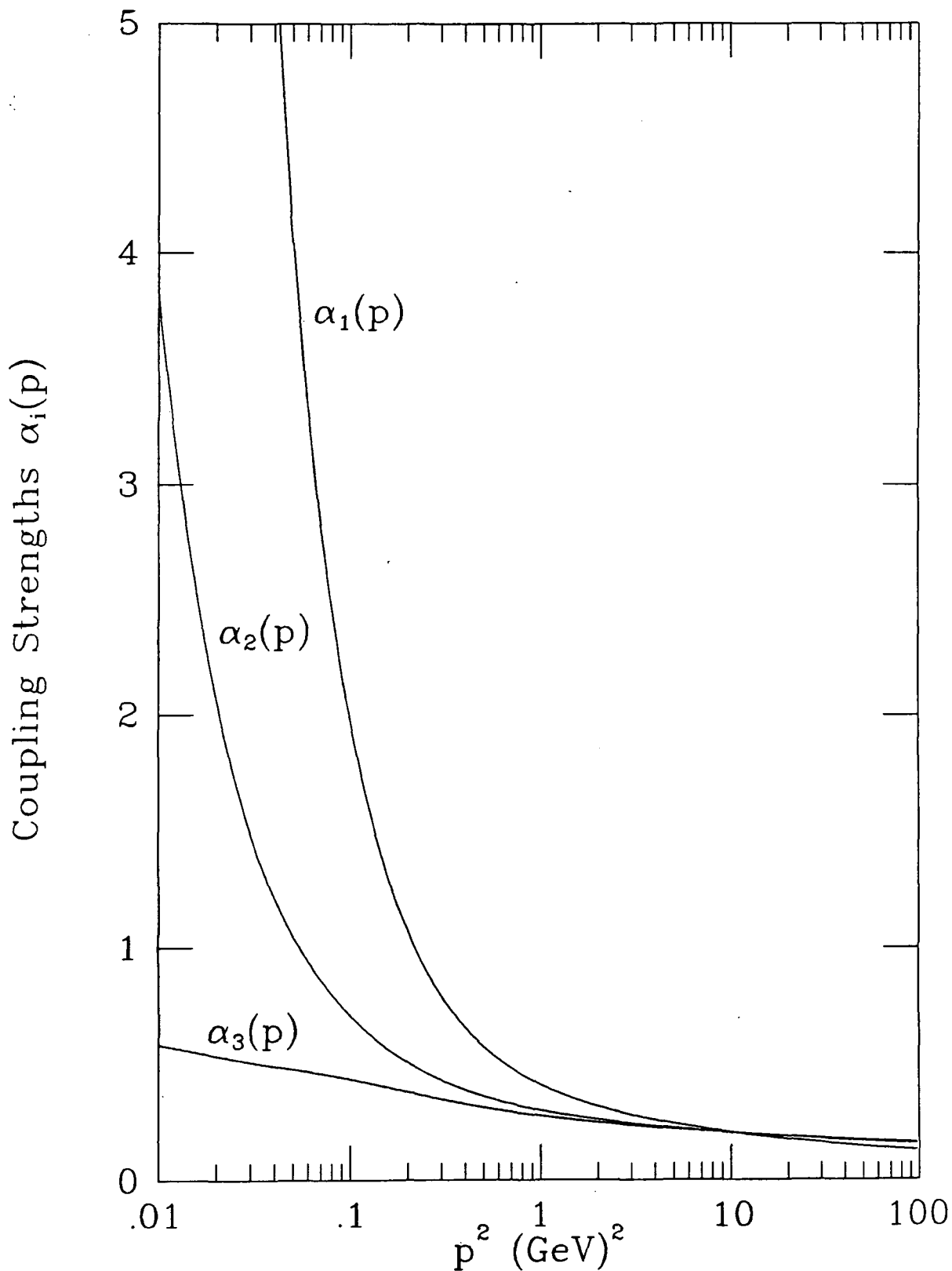
fig. 7.1: The three running couplings \alpha_i(\mu) , with i = 1, 2, 3 , as a function of p^2 , with \alpha_i(\mu) = 0.2 , i = 1, 2, 3 .
