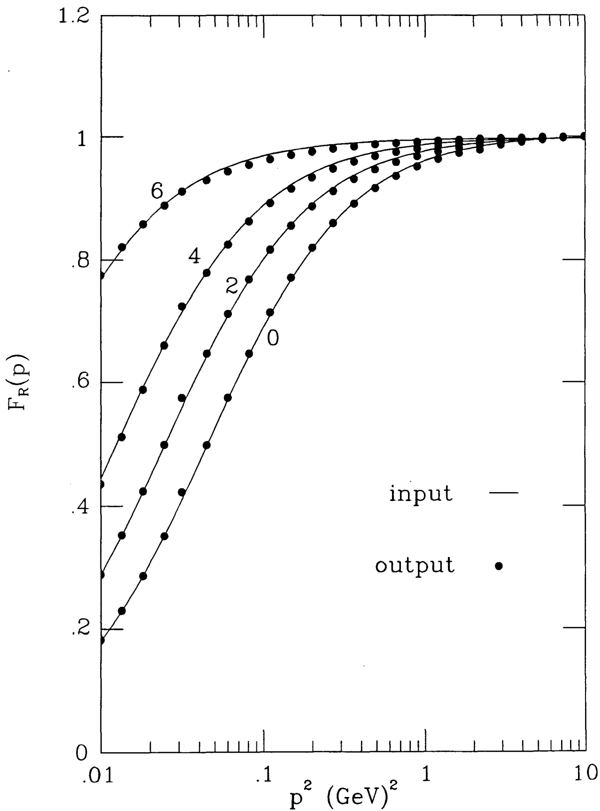
fig. 6.5: The quark renormalisation function \mathcal{F}_R(p) as a function of p^2 for \alpha(\mu) = 0.2 , with n_f = 0, 2, 4, 6 .
