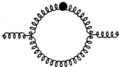
fig. 4.1: The gluon loop diagram in the Mandelstam approximation.
