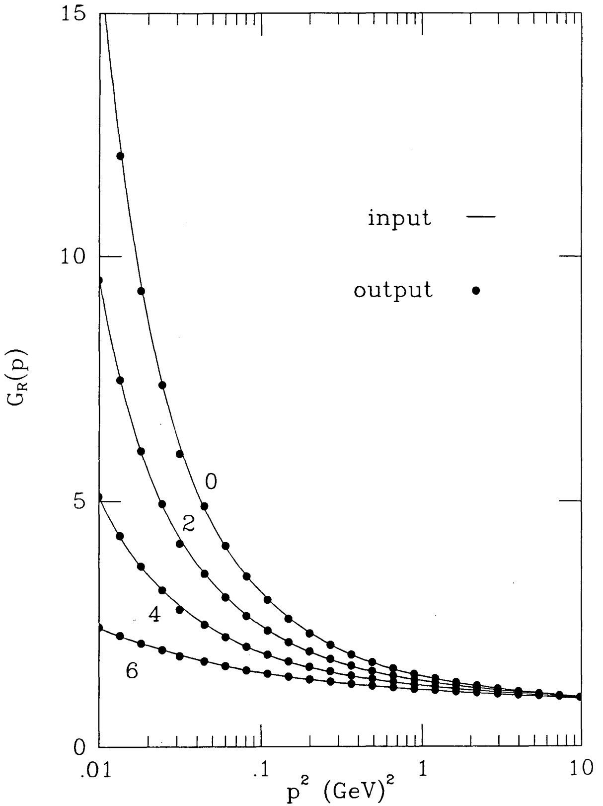
fig. 6.4: The gluon renormalisation function \mathcal{G}_R(p) as a function of p^2 for \alpha(\mu) = 0.2 , with n_f = 0, 2, 4, 6 .
