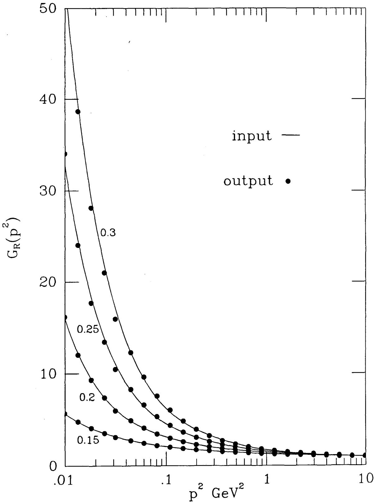
fig 4.3: The gluon renormalisation function \mathcal{G}_R(p) in the Mandelstam approximation, as a function of p^2 , for \alpha_1(\mu) = 0.15, 0.2, 0.25, 0.3 .
