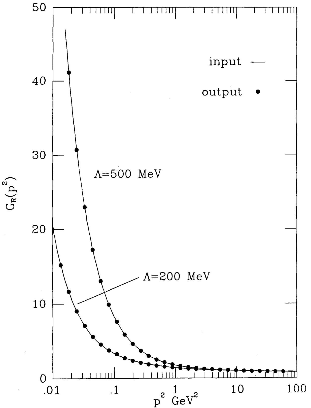
fig. 3.2: The gluon renormalisation function \mathcal{G}_R(p) as a function of p^2 for \Lambda = 200, 500 \text{ MeV} .
