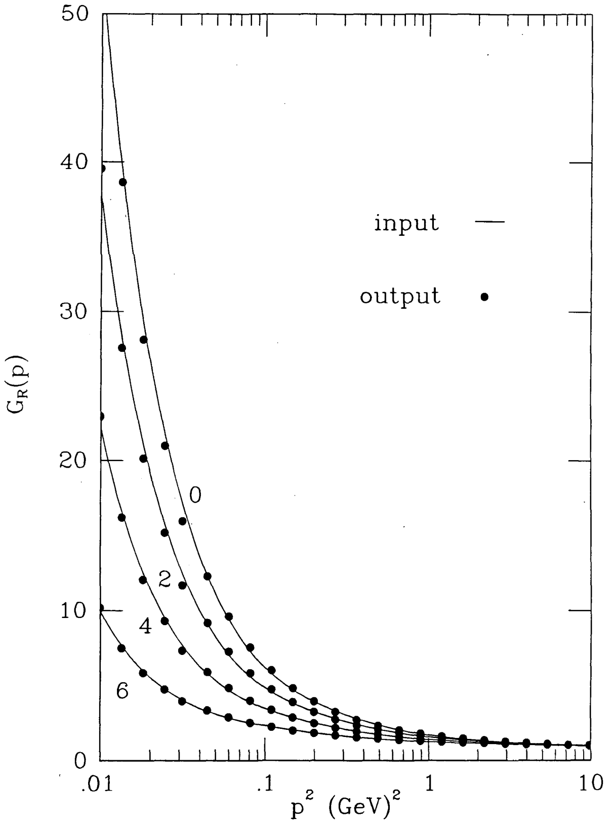
fig. 6.8: The gluon renormalisation function \mathcal{G}_R(p) as a function of p^2 for \alpha(\mu) = 0.3 , with n_f = 0, 2, 4, 6 .
