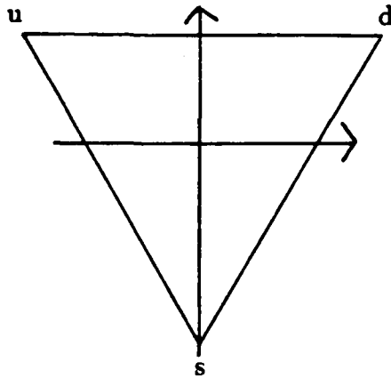
Fig 1.2: fundamental quark triplet of SU(3).
