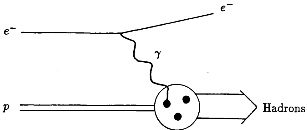
Fig 1.3: Deep Inelastic Scattering. A high energy virtual photon scatters off a parton inside the proton.
