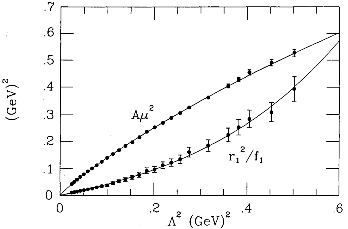
fig. 7.3: The gluon enhancement scale A\mu^2 , and the quark suppression scale r_1^2/f_1 , as a function of \Lambda_1^2 . Also plotted are the curves described in Eq. 7.6. The error bars were determined from an input-output analysis of our solutions to the Schwinger-Dyson equations.
