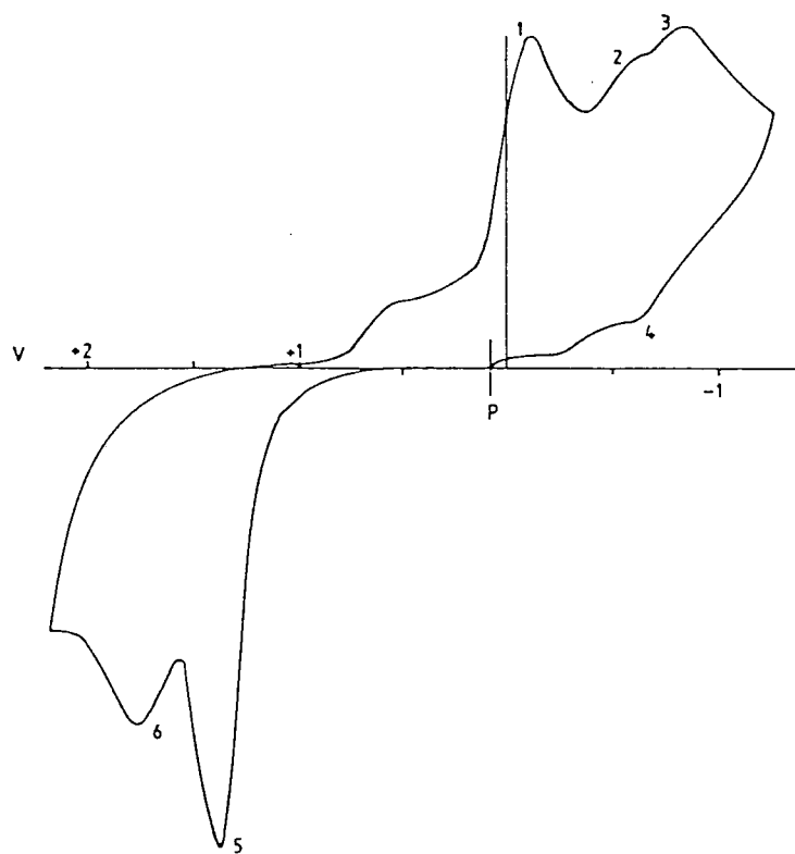
b) Cyclic voltammogram of S_5N_5AsF_6 in CH_3CN at -30^\circ C after holding at potential P for 3 minutes followed by scanning in the positive direction.
