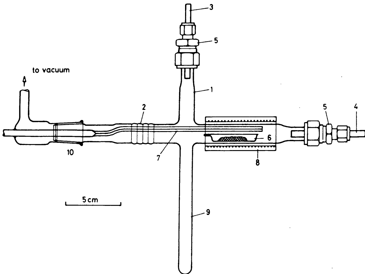
Figure 2.3 The plasma tube used for small scale reactions.
