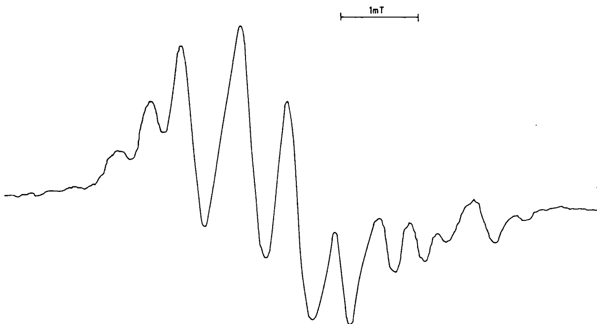
b) The e.s.r. spectrum taken at 90^\circ to a) showing the orientation dependence of the crystal.
