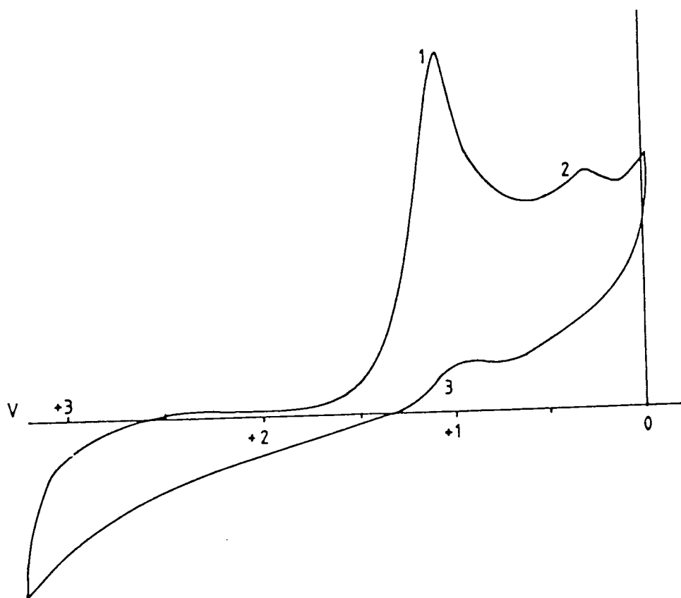
Figure 4.5 Cyclic voltammogram of [\text{SN}]\text{AsF}_6 in \text{CH}_3\text{CN} at -30^\circ\text{C} .
