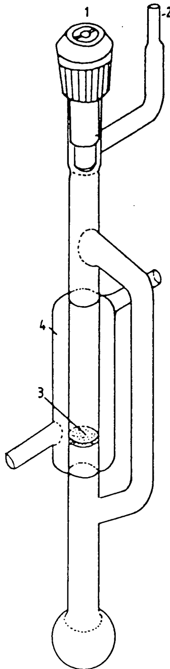
Figure 2.2 The "closed extractor".
