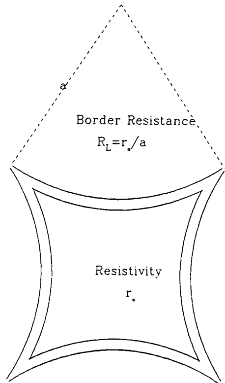
Figure 4.13: Schematic diagram of the design of the IPD detector head.
