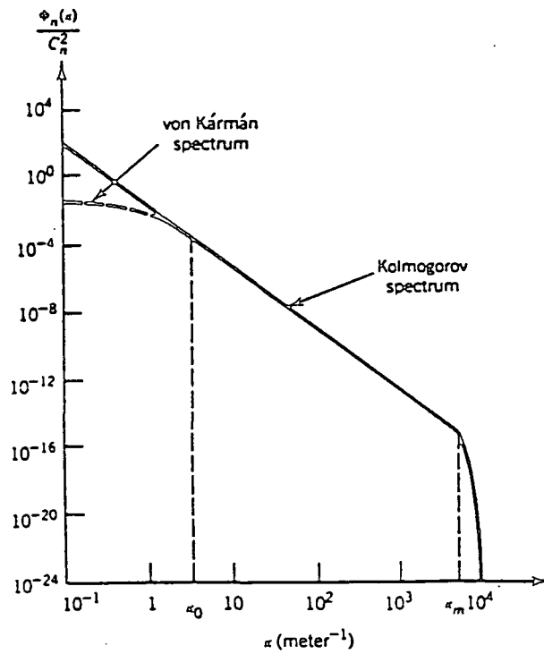
Figure 2.2: Power spectrum of refractive index fluctuations (from Goodman [3]).
