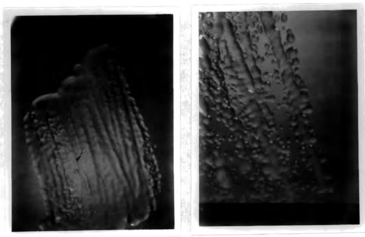
Fig.3.1. Growth patterns of 316NCIB11767 on L-Strep. To test for plasmid presence samples were taken from the L-Strep plates, or in the case of the non growers, from the L-agar. DNA was extracted, restricted with different restriction enzymes and run on a 0.7% agarose mini-gel in tris-borate buffer containing ethidium bromide. The gel was photographed under U.V. light using a polaroid 545 land film type 52.
