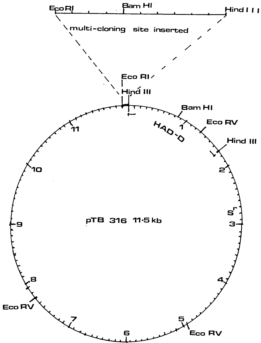
Fig. A.1. Restriction map of plasmid pTB316 showing HAD-D insert and appropriate restriction sites used in the project.
