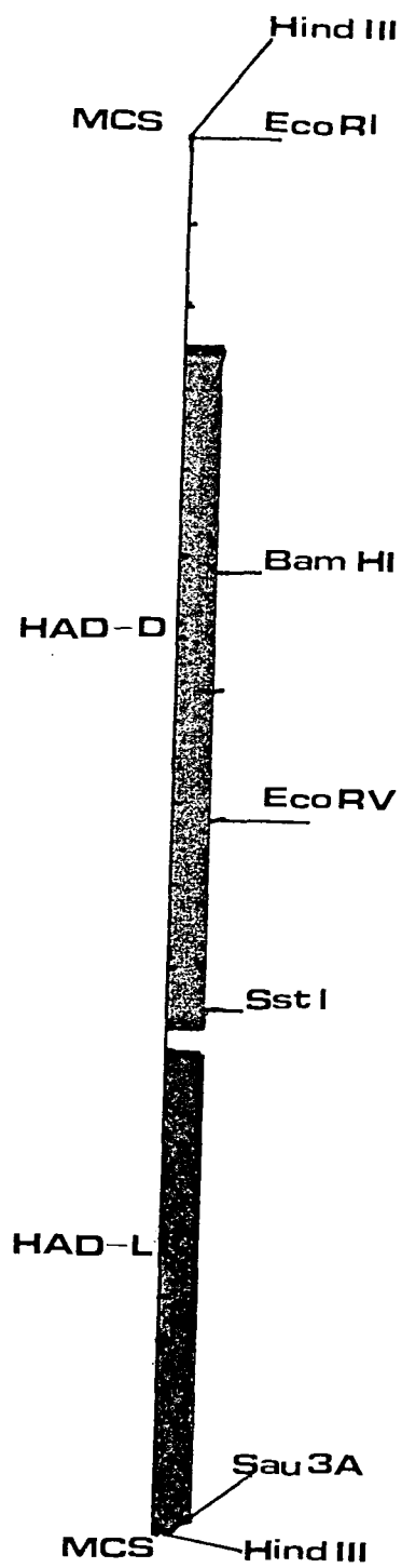
Fig. A.2 Restriction map of the HAD-D/HAD-L insert showing restriction sites of the enzymes used in the project.
