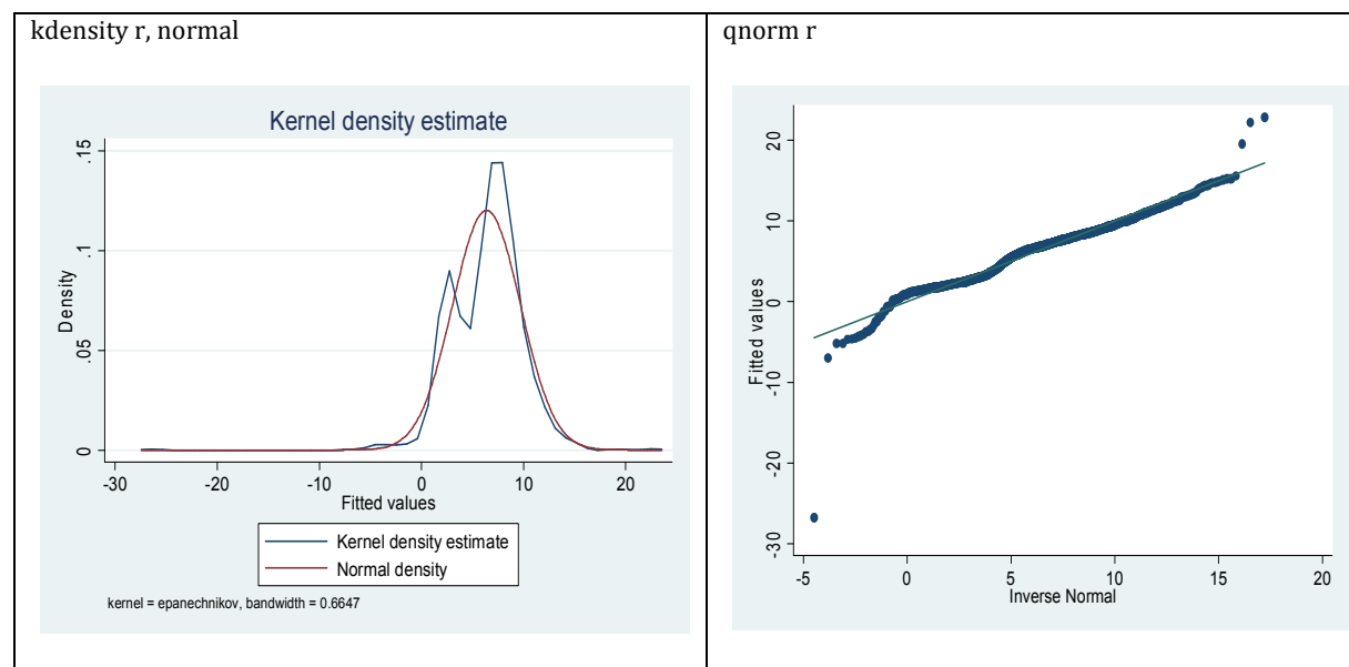
Fig. 5.3: Graphical tests for normality
