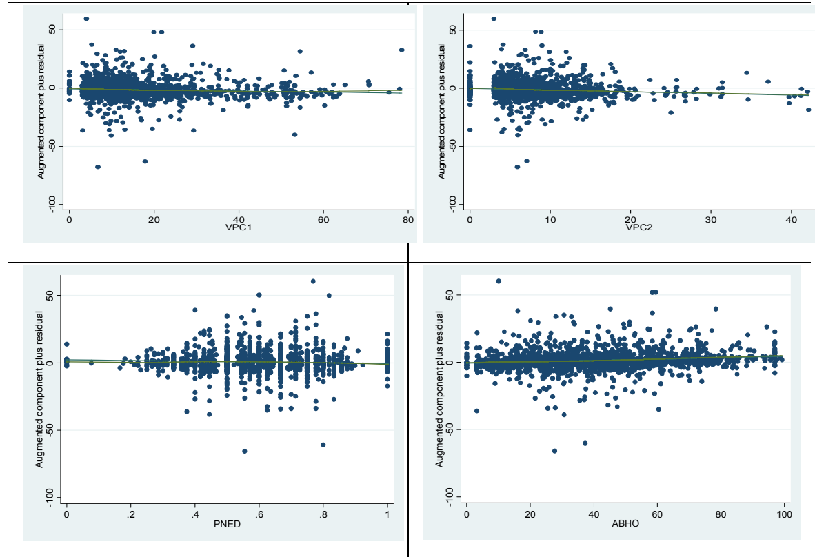
Fig.5.6: Tests for linearity on VPC1, VPC2, PNED and ABHO
