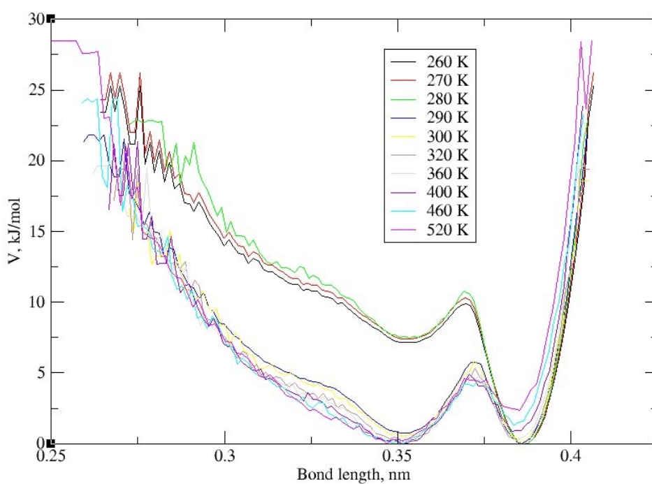
(b) Bond length potential
