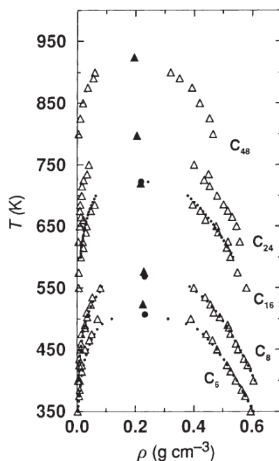
(c) SKS-longer alkanes
