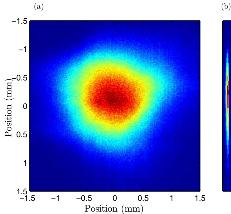
Figure 5.17: (a) A false colour fluorescence image of the MOT taken with the CCD camera used for atom number/density measurements, corresponding to the spatial distribution of the ground state. (b) A false colour image of the Rydberg state spatial distribution made up of 12 vertical translation measurements. The spatial proportions are the same for both images.
