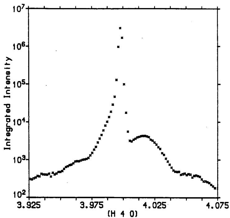
Figure 7.2: The intensity distribution along [100] , the face normal direction, through the \text{InP} (440) Bragg peak from sample INP2.
