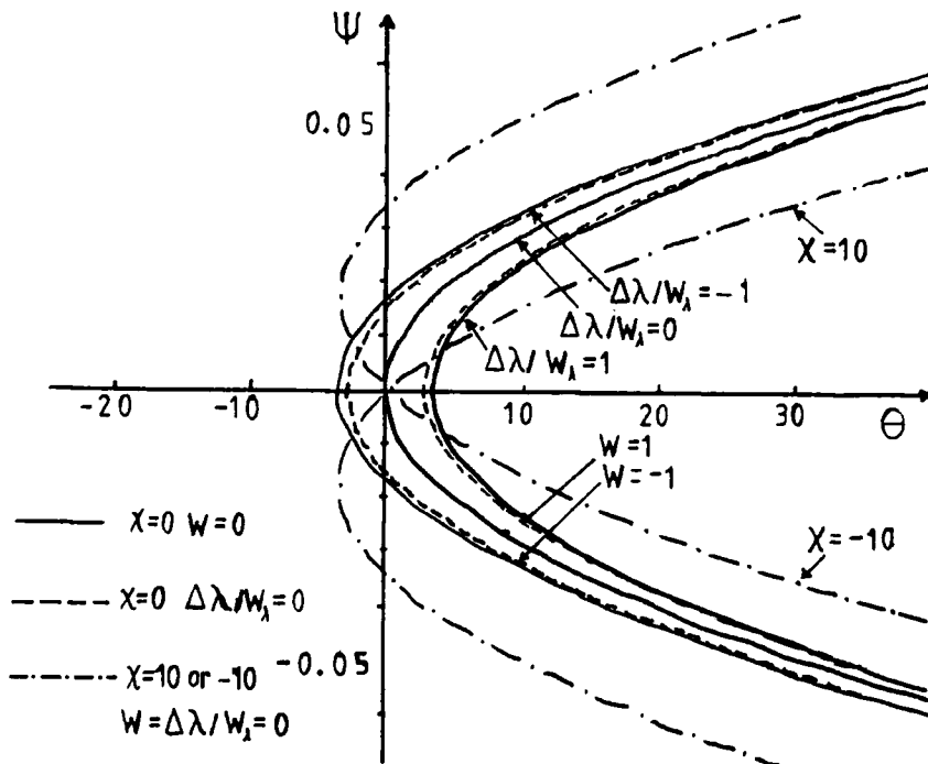
Figure 2.10: Curve of \psi vs ( \theta ) for a non-parallel (+, -) setting with \text{Si}(111) and \text{Si}(220) reflections. \text{CuK}\alpha_1 radiation with the abscissa scaled in units of 1.55 arc seconds. After Yoshimura (1984).
