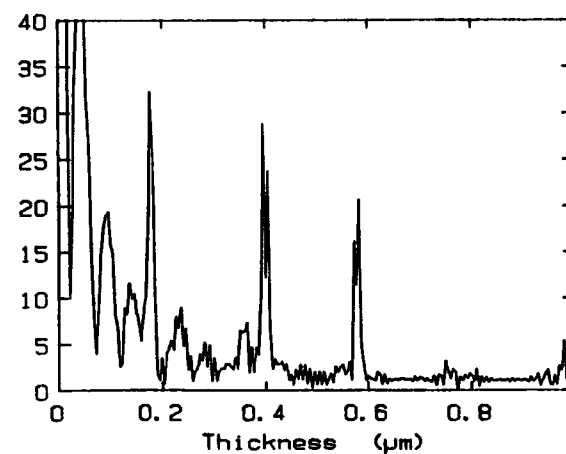
Figure 6.8: 004 rocking curves and Fourier Transforms of a structure comprising of a 0.18\mu\text{m} active layer with mismatch of (a) -200\text{ppm} , (b) -500\text{ppm} , (c) -1000\text{ppm} and (d) -1500\text{ppm} , with a 0.4\mu\text{m} cap.
