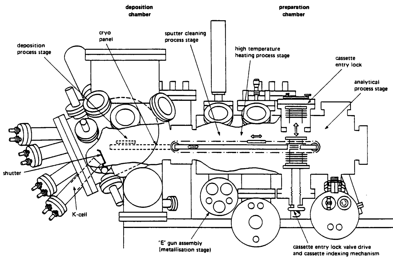
Figure 1.11: Cross-sectional view of an MBE system illustrating the configuration of the major components. After Davies and Andrews (1985).
