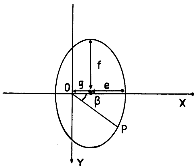
Figure 5.8(b): General form of an ellipse.
