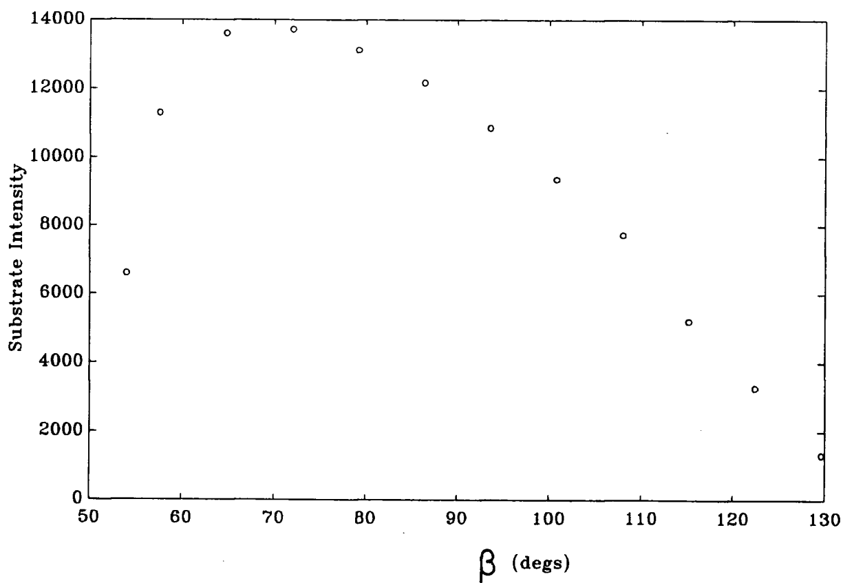
Figure 5.17(b): Substrate peak height found experimentally for the 133 reflection.
