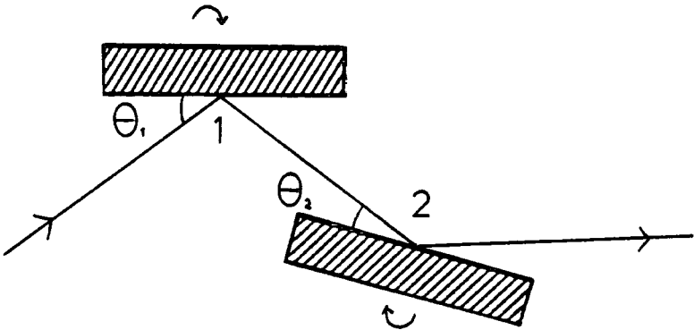
(a) (n, -n) \theta_1 = \theta_2 , non-dispersive
