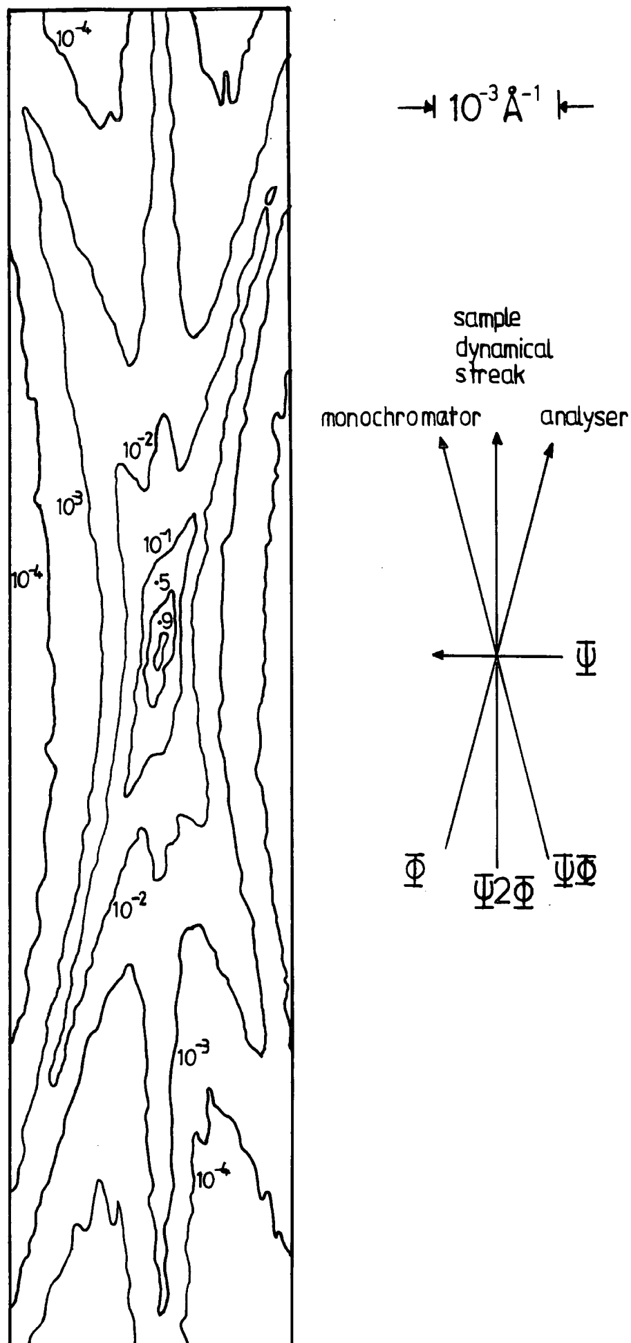
Figure 2.14: Triple crystal diffractometer contour map in reciprocal space with Si(111) monochromator, sample and analyser crystals and a focussing (+1, -1, +1) configuration. CuK\alpha_1 , \theta_m = \theta_s = \theta_a = 14.22^\circ . After Ryan (1986).
