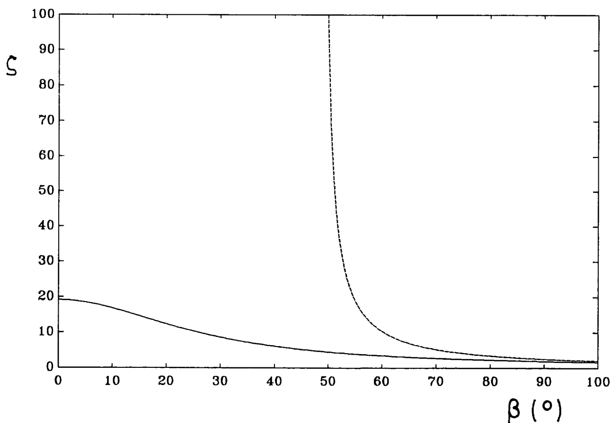
Figure 5.5: Relationship between the path length ratio and rotation angle for 044 (solid), 333 (dashed) and 133 (dotted) reflections.
