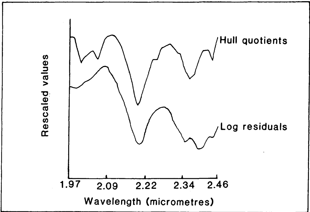
Figure 4.15 The upper plot is the hull quotients output over an area rich in sericite. That below is the log residuals output of the same area. The major absorptions are clearly visible in both spectra, with the added atmospheric CO_2 absorptions in the hull quotients spectra around 2.00\mu m .
