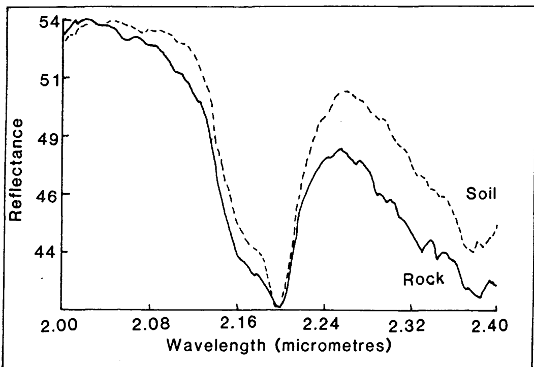
Figure 5.31 Laboratory spectra from Plateau, location 3. Both rock and soil show the diagnostic doublet of kaolinite (2.16 \mu\text{m} shoulder, 2.2 \mu\text{m} minima).
