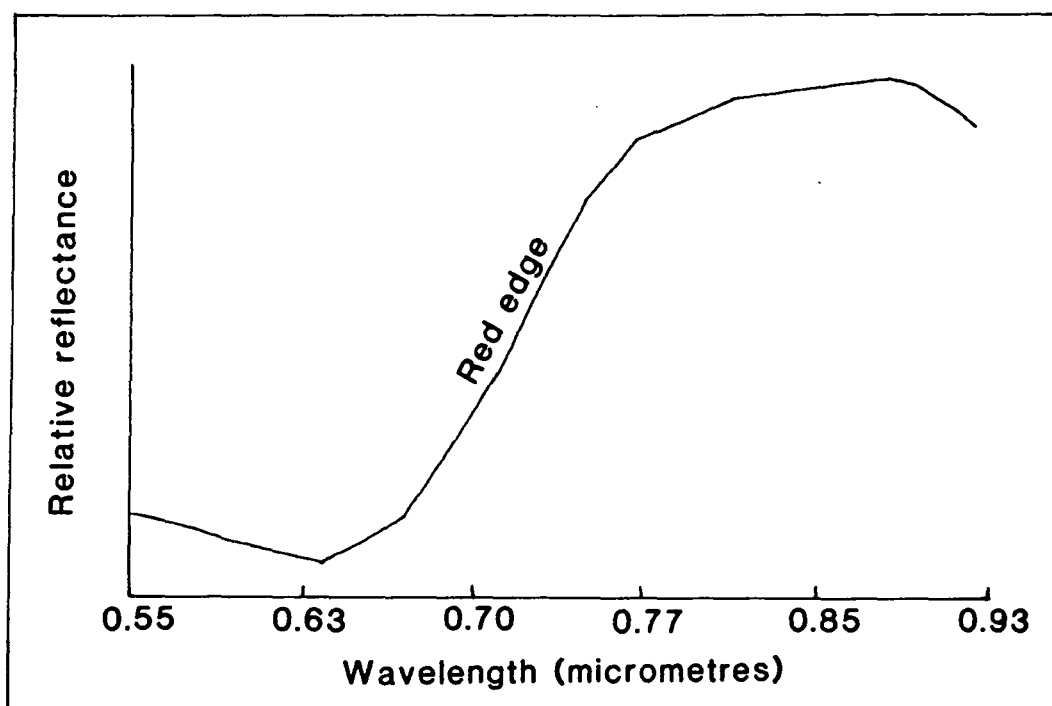
Figure 6.15 The corresponding VNIR spectra of green vegetation, from the area covered above. Note the step rise in reflectance at the red edge.
