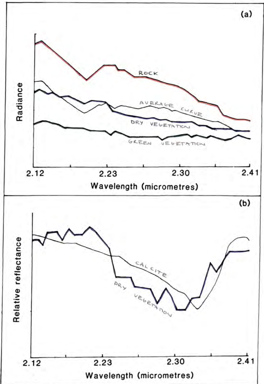
Figure 4.12 (a) The spectral curves of three materials are shown, with their average curve (black). (b) After performing the second step of log residuals, the curve averaging step (using the black curve). The dry vegetation residual curve is compared with a reflectance spectrum of calcite.
