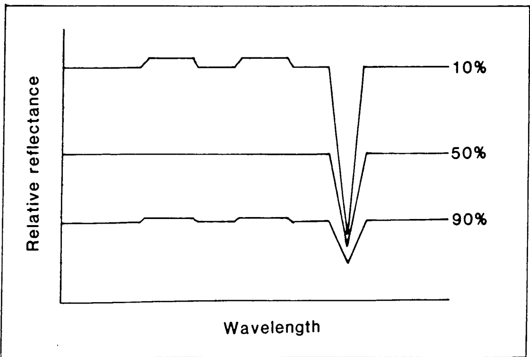
Figure 4.11 Varying the percentage of a scene component in the scene average will affect the output curves. The curves shown are the log residuals output of the data from figure 4.10, for percentages of 10%, 50% and 90% of the material with the extra absorption.
