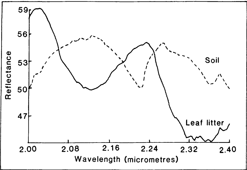
Figure 5.21 Laboratory spectra from Arsenopyrite, location 4. The anomaly is centred on a tree with no outcrop. The soil shows a small unidentifiable clay feature. A spectrum of the dry leaf litter present at the location is also shown.
