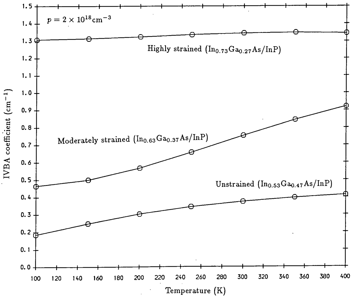
Temperature variation of bound-unbound IVBA in 1.3\mu\text{m} laser devices.
