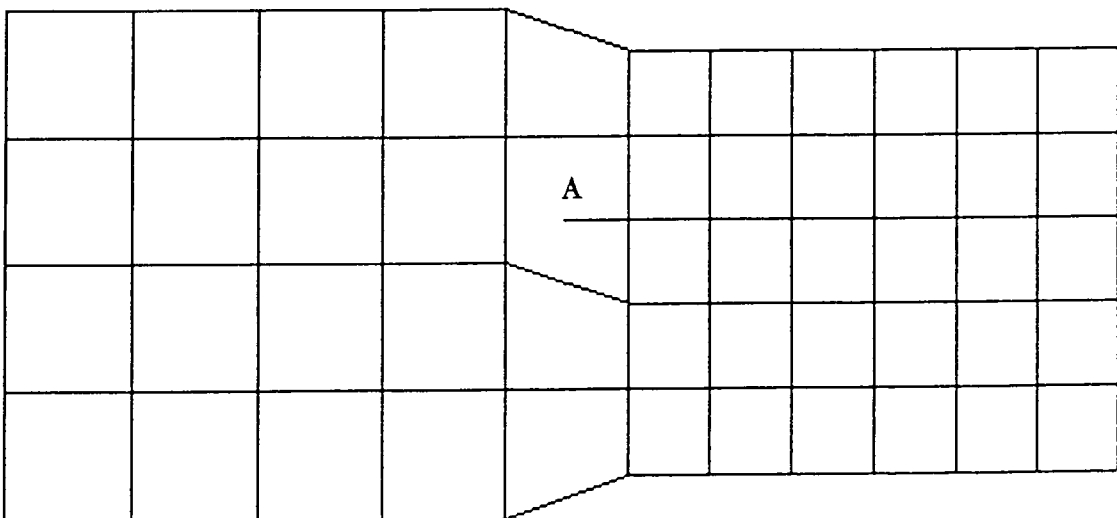
c) Relaxed regime, showing dangling bond (A).
