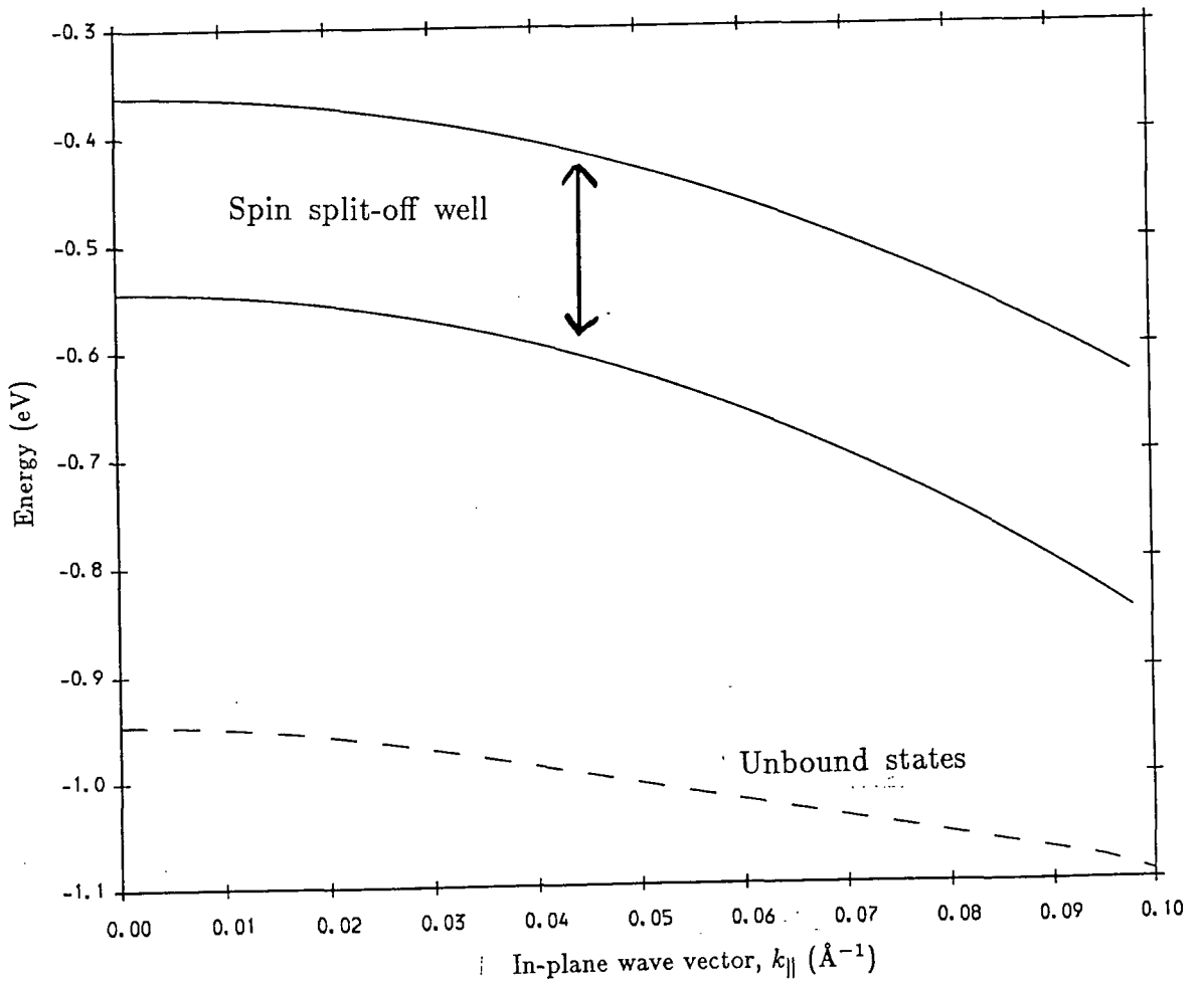
Variation of spin split-off well with in-plane wave vector.
