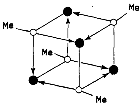
Figure 3.2: Crystal Structure of Thallium(I) Methoxide 72
