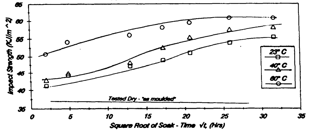
5.34(b) Impact Strength against √ Soak - Time Soak - Temperatures : 23, 40 & 60° C Charpy Impact Samples - (Notched)
