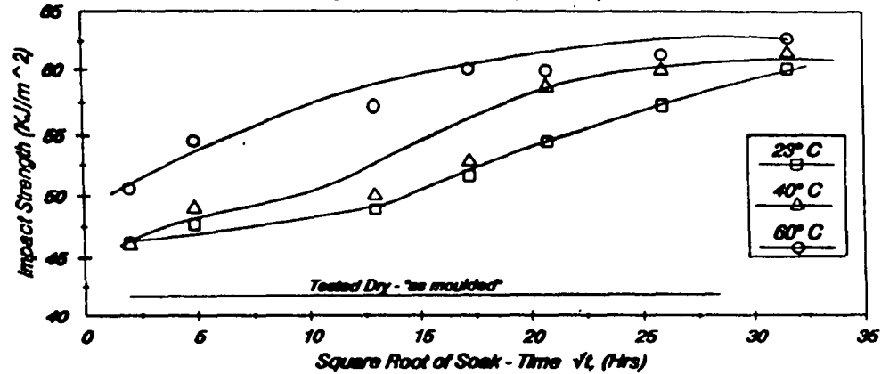
5.33(b) Impact Strength against √ Soak - Time Soak - Temperatures : 23, 40 & 60° C Charpy Impact Samples - (Notched)
