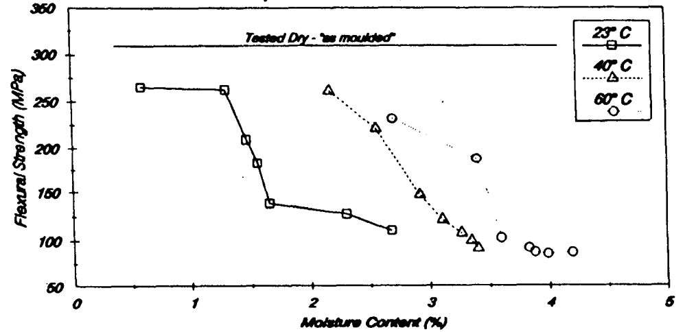
5.17(a) Flexural Strength against Moisture Content Soak - Temperatures : 23, 40 & 60° C
