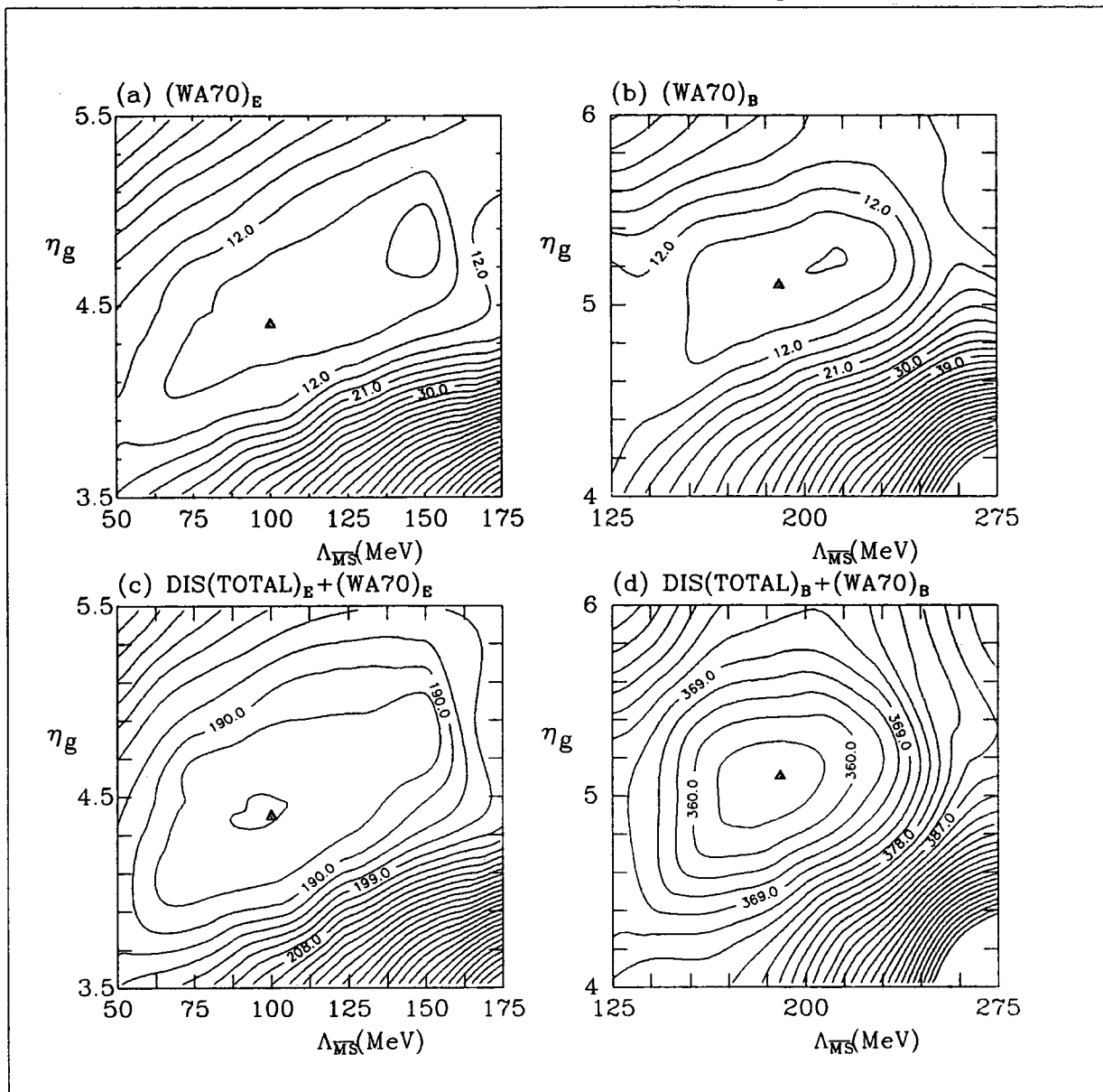
Figure 6.4 (a) and (b) show contours of constant \chi^2 (with an interval of three units) in the \Lambda_{\overline{MS}} - \eta_g plane where \chi^2 is a measure of the quality of the theoretical prediction for the WA70 prompt photon data [66] in the range -0.35 < x_F < 0.45 (corrected to y = 0 ) using the various sets of parton distributions obtained by fitting to the deep-inelastic scattering data of ((a))[32], ((b))[16] ( F_2^{\mu p} ), [36] ( F_2^{\nu N} and x F_3^{\nu N} ) and [40], [42], [43] ( F_2^{\mu n} / F_2^{\mu p} ). The statistical and systematic errors of all data have been combined in quadrature. (c) and (d) show the corresponding total \chi^2 when the \chi^2 to all the deep-inelastic data is added and indicates the quality of the simultaneous description of the deep-inelastic and prompt photon data. The optimum overall description is obtained for the values of \Lambda_{\overline{MS}} and \eta_g shown by the triangles.
