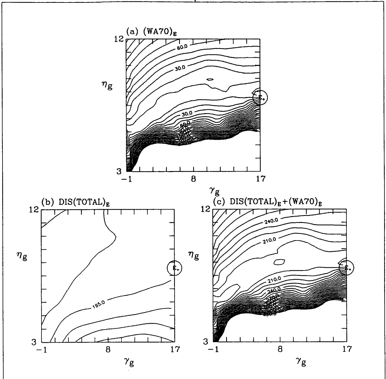
Figure 9.3 (a) shows contours of constant \chi^2 in the \gamma_g - \eta_g plane where \chi^2 is a measure of the quality of the theoretical prediction for the WA70 prompt photon data [66] in the range -0.35 < x_F < 0.45 (corrected to y = 0 ) using the various sets of parton distributions obtained by re-evolving the HMRS(E) set with the gluon momentum redistributed in the form xg(x, Q_0^2) = A_g x^{\delta_g} (1-x)^{\eta_g} (1 + \gamma_g x) with \delta_g = +1/2 . (b) shows the total \chi^2 to the deep-inelastic scattering data of [32] (EMC F_2^{\mu p} ), [36] ( F_2^{\nu N} and x F_3^{\nu N} ) and [40], [42], [43] ( F_2^{\mu n} / F_2^{\mu p} ). (c) is the total of (a) and (b). 'E + ' signifies the position of the gluon chosen for illustrative purposes (see text). The statistical and systematic errors of all data have been combined in quadrature. The contour interval is 10 units of \chi^2 for all three contour plots.
