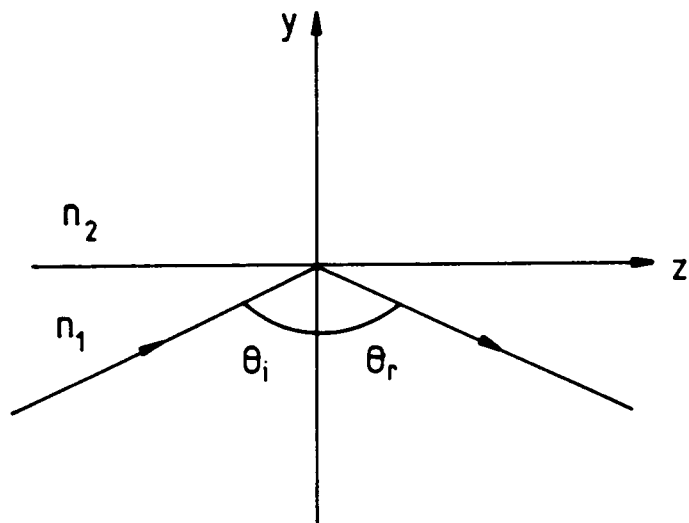
Figure 3.1. a) When an electromagnetic wave is incident upon the boundary between two dielectric media whose refractive indices are n_1 and n_2 , with n_1 > n_2 , then in general a portion of the wave is reflected and the remainder is transmitted. b) Total internal reflection is produced when \theta_i > \theta_c .
