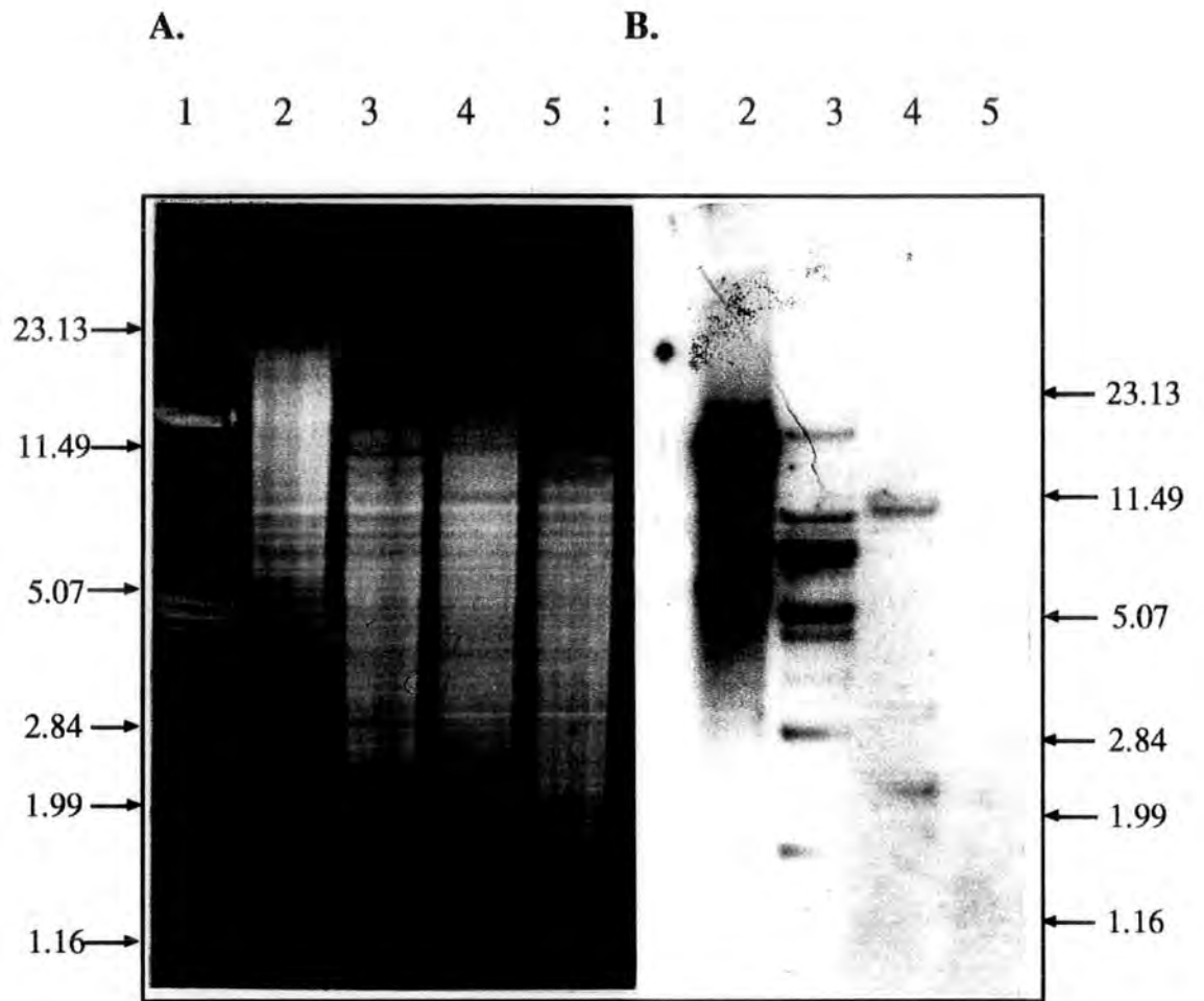
Figure 4.3 : Southern blot analysis of bacterial chromosomal DNA digests with oligonucleotide probe A.
