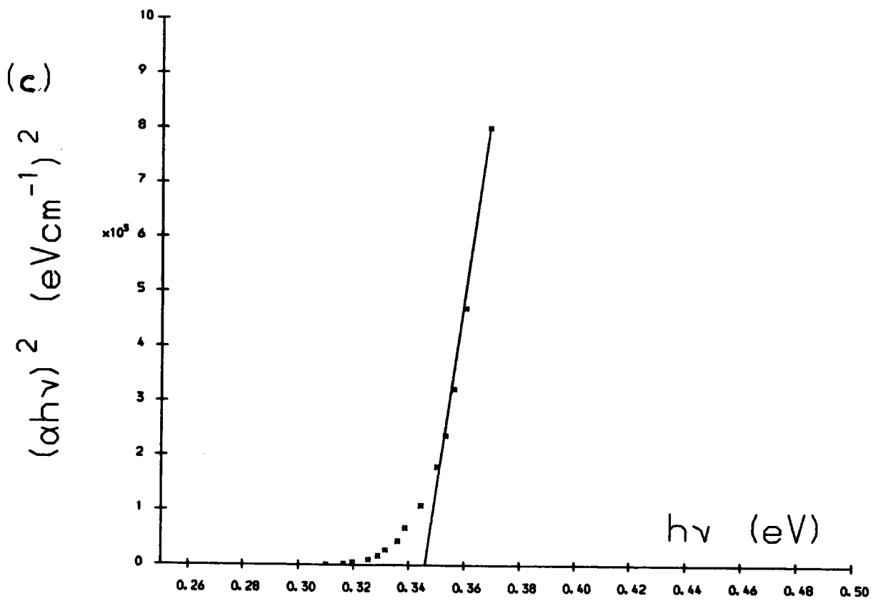
Fig. 5.4(b) Absorption coefficient ( \alpha ) versus photon energy ( h\nu ) and (c) (\alpha h\nu)^2 versus ( h\nu ) for MCT78.
