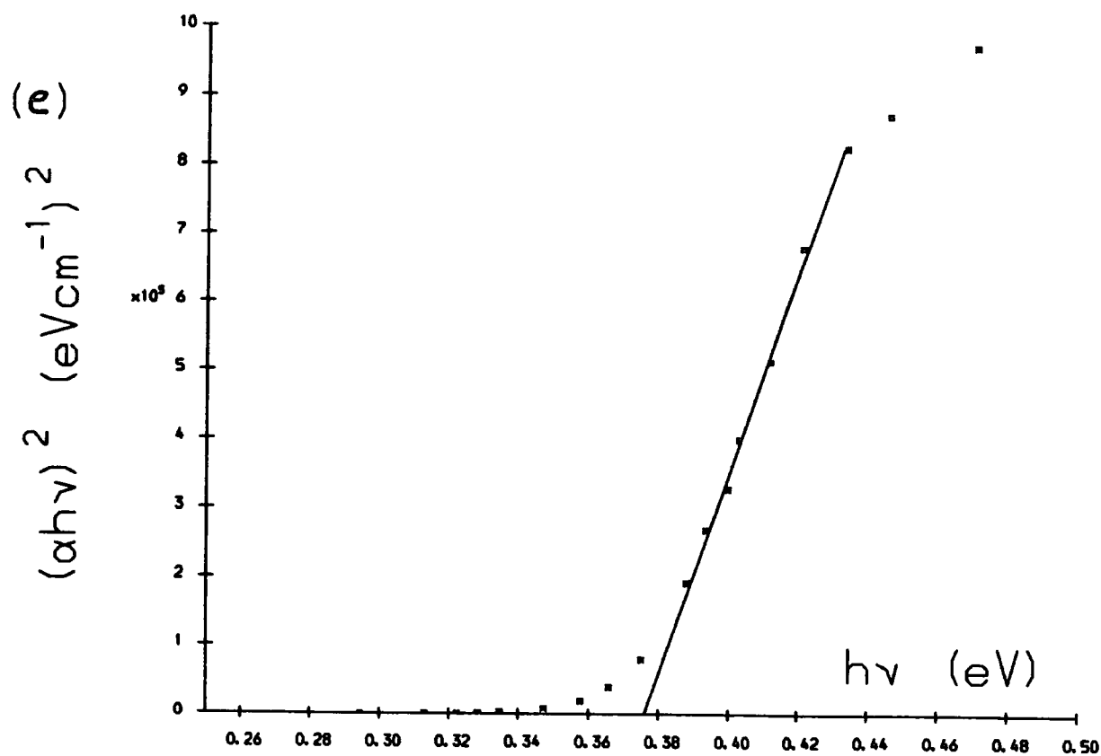
Fig. 5.2(d) Absorption coefficient ( \alpha ) versus photon energy ( h\nu ) and (e) (\alpha h\nu)^2 versus ( h\nu ) for a second region of MCT37.
