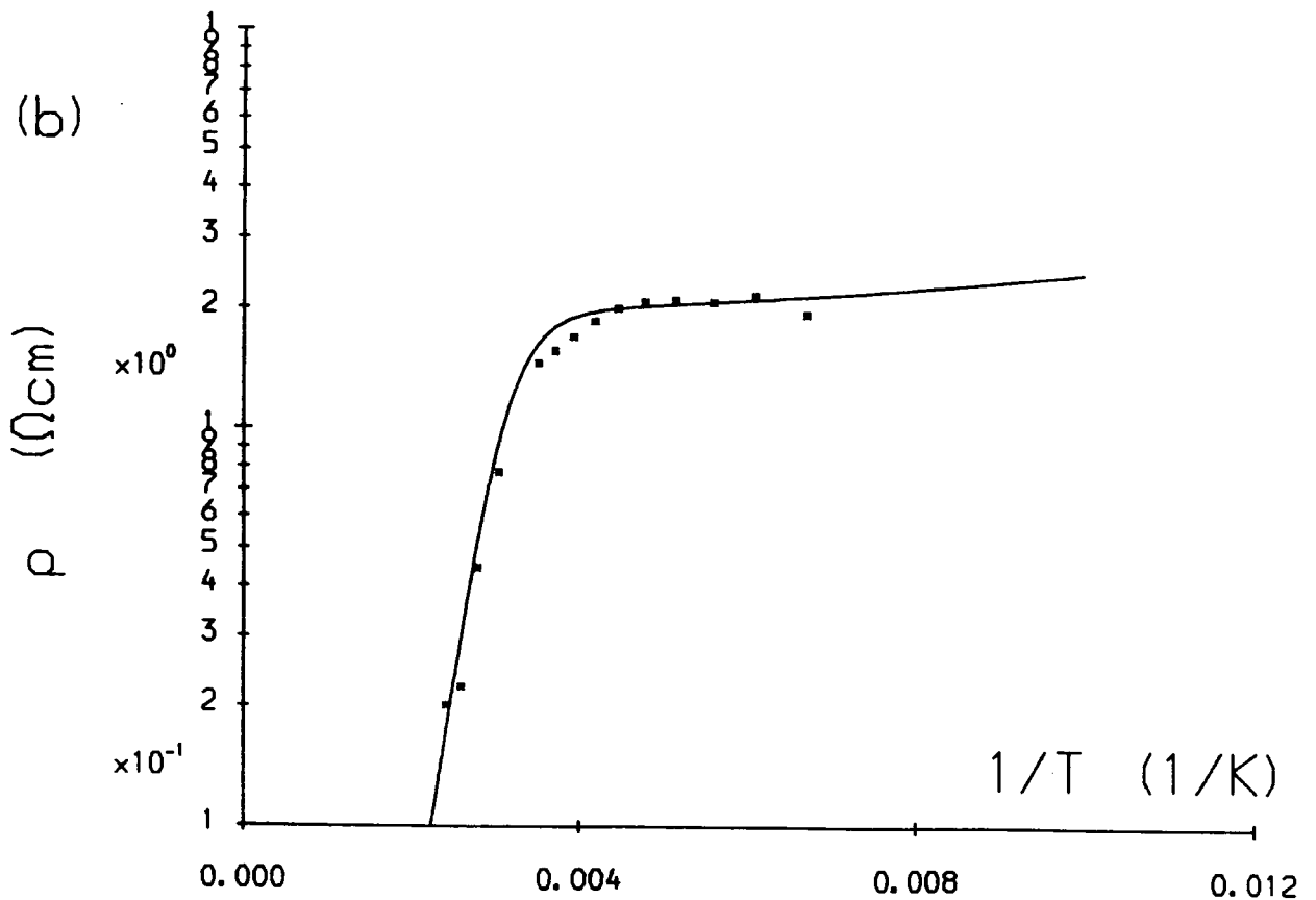
Fig. 5.9(a) Hall coefficient ( R_H ) versus inverse temperature ( 1/T ) and (b) resistivity ( \rho ) versus ( 1/T ) for GEC630.
