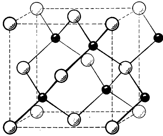
Fig.1.1. The Sphalerite Structure.
