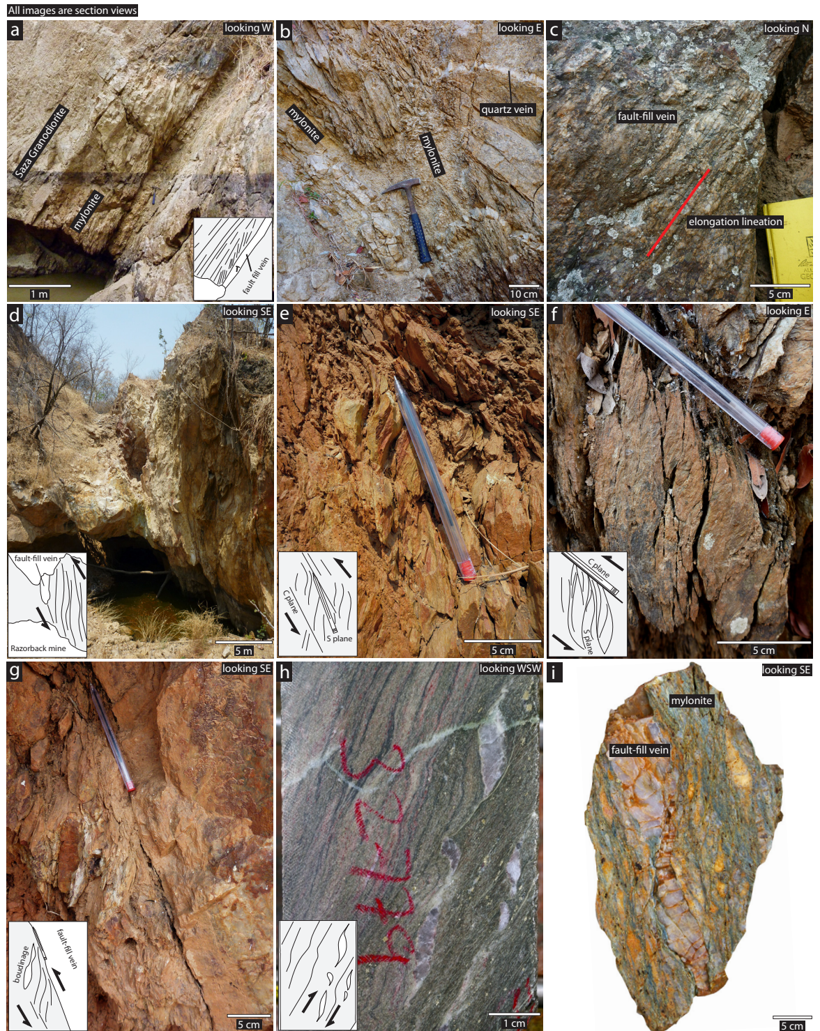
Figure 5.5 – (a) Photo of E-W trending shear zone from artisanal working. The complete transition from hydrothermally altered Saza granodiorite to mylonitic shear zone is exposed; (b) photo of quartz veins pre-dating E-W trending shear zone at artisanal working; (c) quartz rods on fault-fill vein and mylonitic shear zone contact; (d) photo from the Kenge ore body looking SE (standing in what was formerly known as Razorback mine). The mylonitic foliation possesses a steeper dip relative to the shear zone boundary (ca. 70^\circ ; not shown); (e) photo from artisanal working at the Kenge SE zone showing S/C fabrics indicative of south-side up movement; (f) photo from E-W trending artisanal working showing S/C fabrics indicative of south-side up movement; (g) photo from artisanal working at the Kenge main zone showing S/C fabrics indicative of south-side up movement; (h) photo of partially oriented core from Porcupine showing asymmetric porphyroclasts and the mylonitic foliation wrapping quartz-feldspar micro-lithons; (i) oriented sample from NW trending shear zone showing deformed fault-fill vein.
