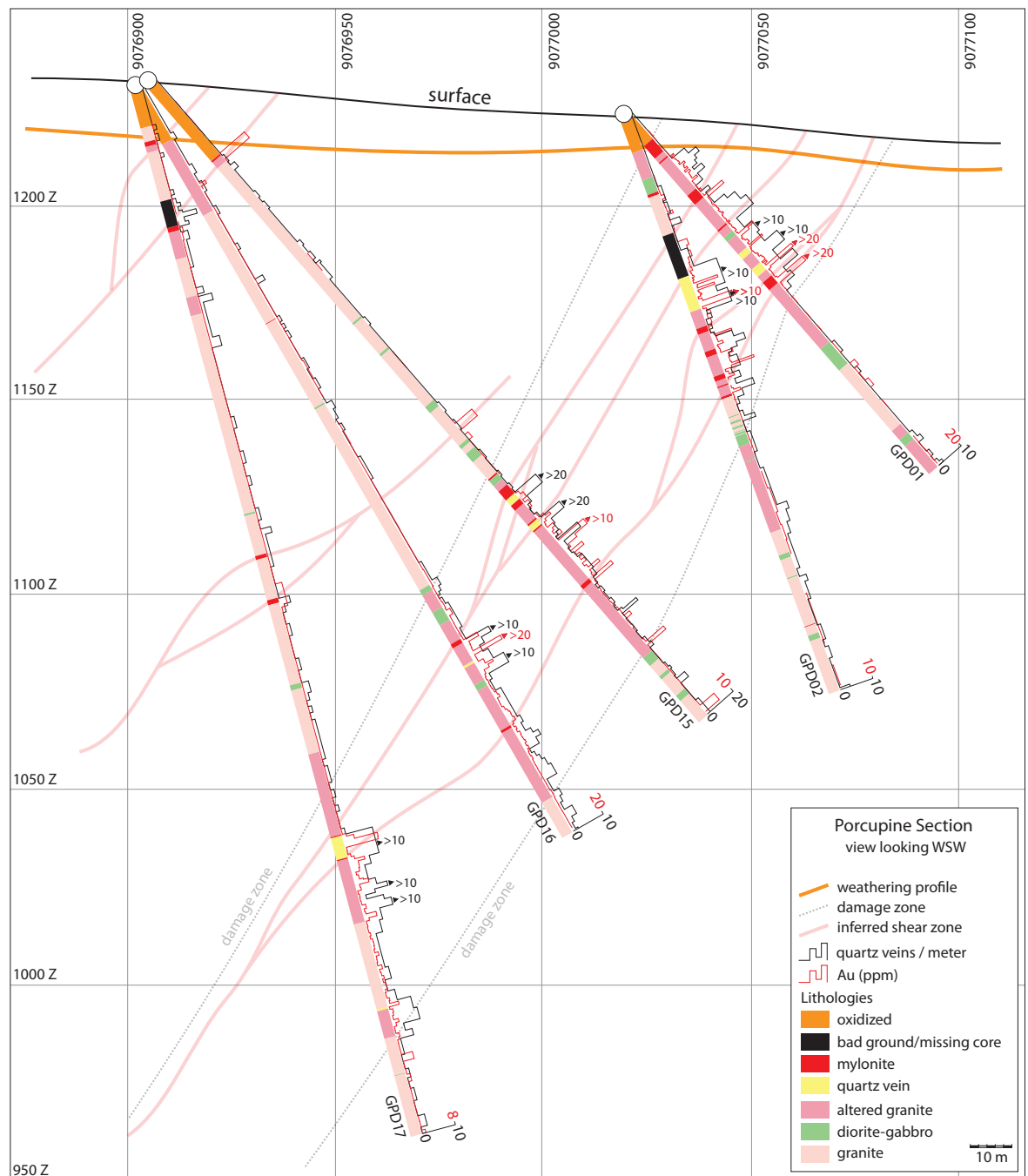
Figure 5.14 – Cross section of Porcupine with lithology logs parallel to diamond drill hole traces. Note correlation between quartz vein intensity (measured as quartz veins / meter) and Au grade. The extent of the damage zone is inferred from the increase in quartz vein density near the interpreted shear zone boundaries.
