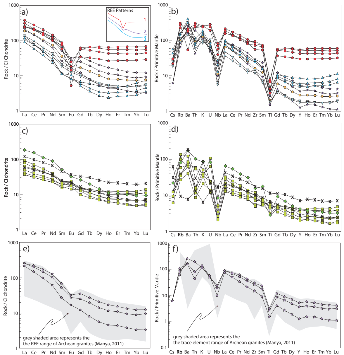
Figure 2.8 – (a–b) REE and trace element plots plot of felsic phases normalized to CL chondrite and primitive mantle, respectively (Sun and McDonough, 1989); (c–d) REE and trace element plots of intermediate-mafic phases normalized to CL chondrite and primitive mantle, respectively (Sun and McDonough, 1989); (e–f) REE and trace element plots of foliated Archean granitoids normalized to CI chondrite and primitive mantle, respectively (Sun and McDonough, 1989). Grey shadings area represents the range of Archean granitoid compositions from the Tanzanian Craton (Manya, 2011). Sample symbols are the same as Fig. 2.6.
