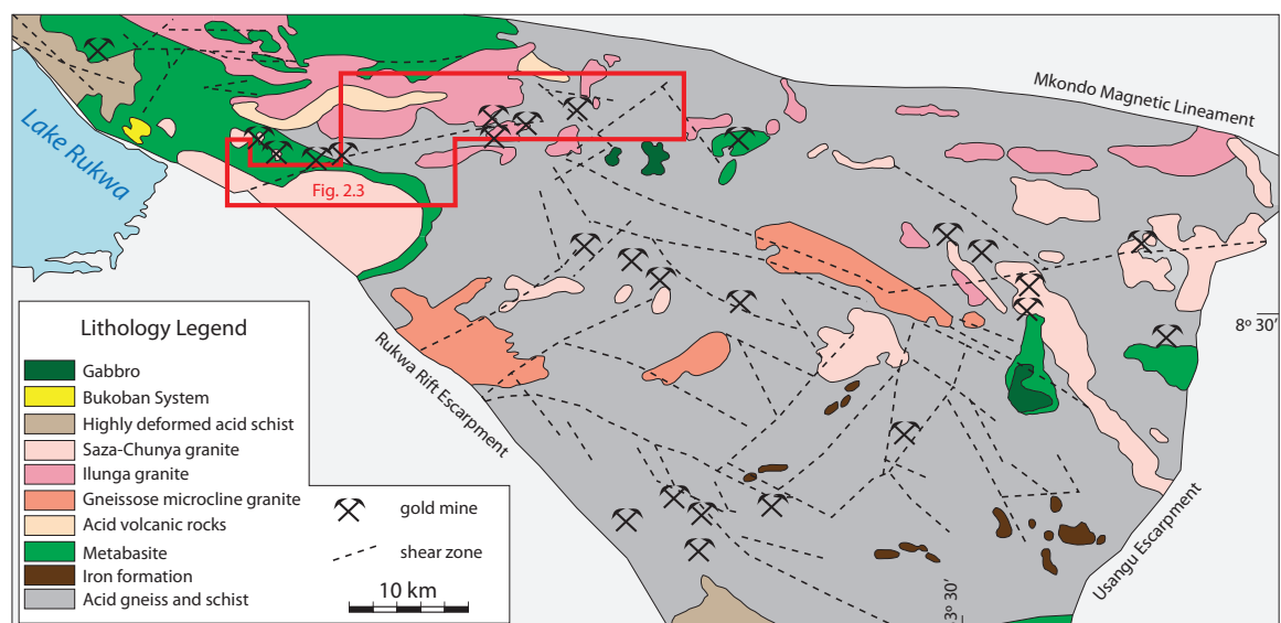
Figure 2.2 – Simplified geology of the Lupa goldfield (modified from Kimambo, 1984).
