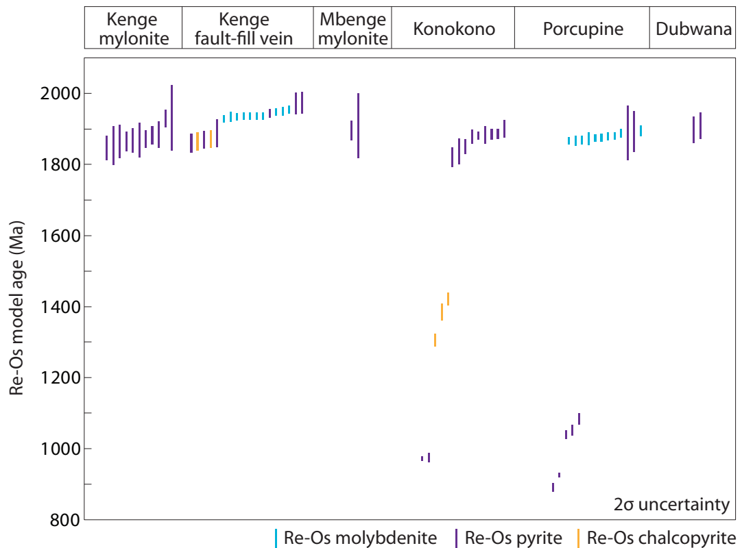
Figure 4.9 – Summary diagram showing all Re-Os model ages at 2\sigma uncertainty level (Re-Os molybdenite model ages are in blue; Re-Os chalcopyrite ages in yellow; Re-Os pyrite ages in purple).
