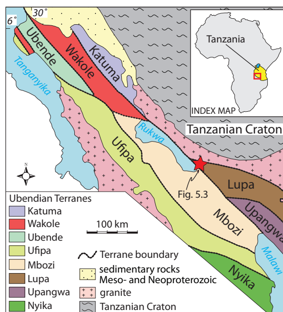
Figure 5.2 – Regional geologic map showing Ubendian Terranes and Tanzanian Craton. The star shows the location of the field area for the current study (modified from Daly, 1988).
