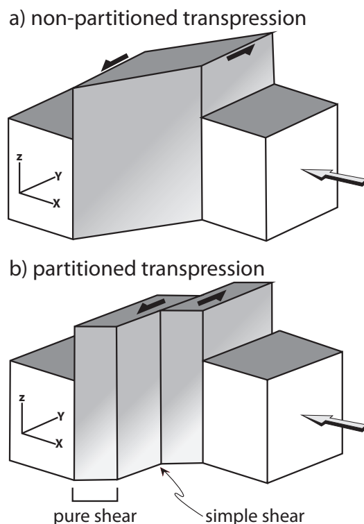
Figure 5.1 – (a) Schematic block model of homogeneous, or non-partitioned transpression; (b) schematic block mode of partitioned transpression where the wrench component of the transpressional strain is compartmentalized into a discrete strike-slip fault (modified from Dewey et al., 1998).
