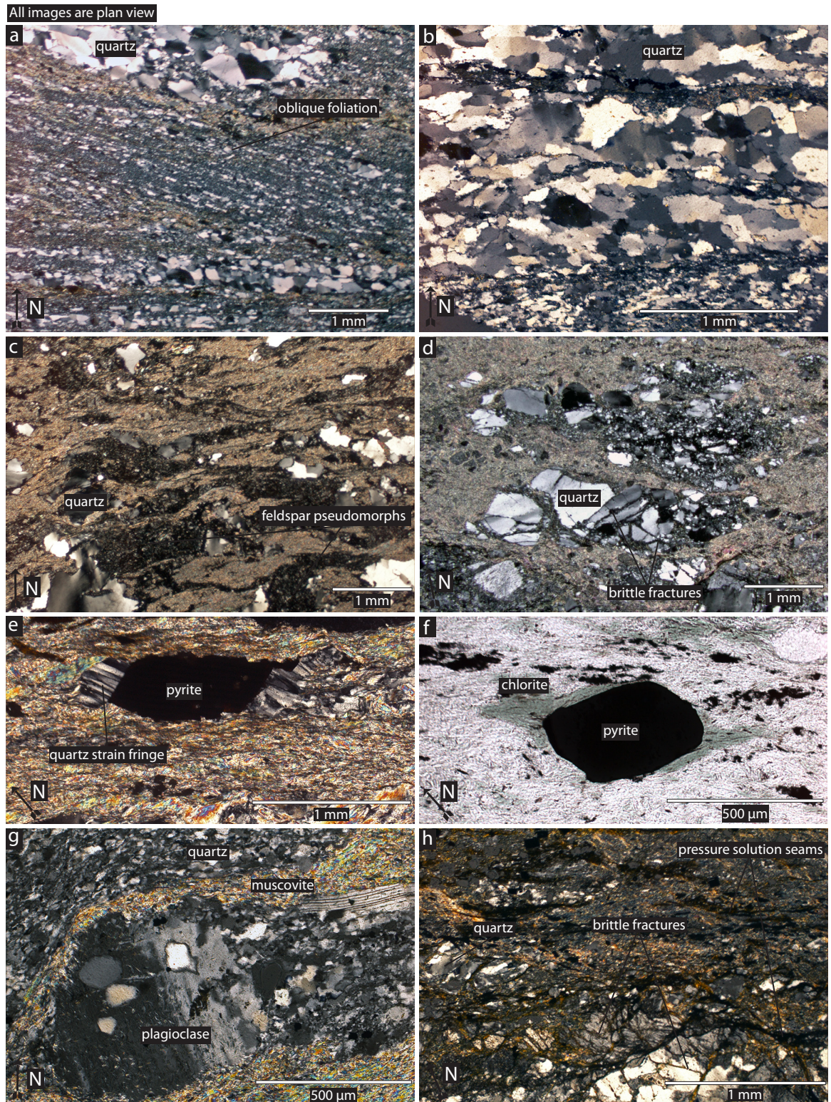
Figure 5.8 – Plan view photomicrographs: (a) crossed nicols photomicrograph of oblique foliation development in plan view (518905, 9079993); (b) crossed nicols photomicrograph showing undulatory extinction, dynamic recrystallization and sub-grain rotation in quartz (518905, 9079993); (c) crossed nicols photomicrograph of feldspar pseudomorphs and strained quartz (498933, 9073405); (d) crossed nicols photomicrograph of quartz ribbons, undulatory extinction and dynamic recrystallization in quartz (499282, 9073258); (e) crossed nicols photomicrograph of pyrite with quartz strain fringe (501850, 9074362); (f) plane polarized light photomicrograph of asymmetric pyrite porphyroblast (501850, 9074362); (g) crossed nicols photomicrograph of plagioclase porphyroclasts wrapped by mylonitic fabric. Note dynamic recrystallization of quartz and neocrystallization of feldspar at porphyroclasts margin (501137, 9072969); (h) crossed nicols photomicrograph of brittle fractured
