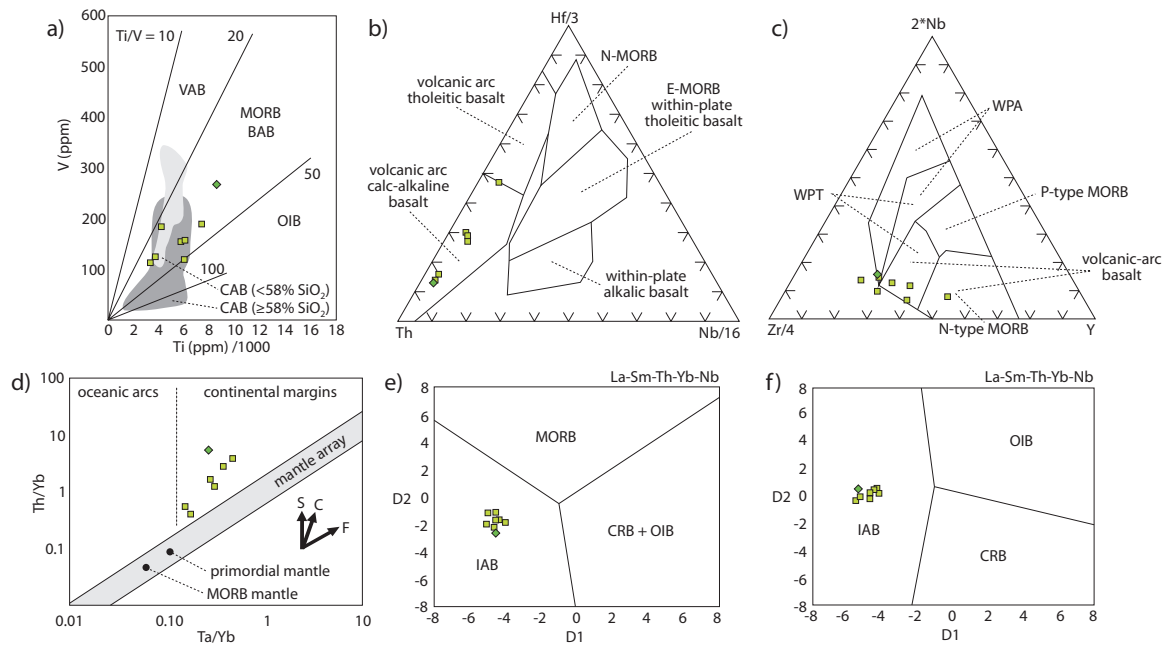
Figure 2.10 – Intermediate-mafic tectonic discrimination diagrams. (a) Basaltoid tectonic discrimination diagram modified from Shervais (1982). VAB = volcanic arc basalt, MORB = mid-ocean ridge basalt, BAB = back-arc basin basalt, OIB = ocean island basalt, CAB = continental arc basalt; (b) basaltoid tectonic discrimination diagram modified from Wood (1980). N-MORB = normal-mid ocean ridge basalt; (c) basaltoid tectonic discrimination diagram modified from Meschede (1986). WPT = within-plate tholeiitic basalt, WPA = within-plate alkalic basalt, P-type MORB = primitive mid-ocean ridge basalt, N-type MORB = normal-type mid-ocean ridge basalt; (d) basaltoid tectonic discrimination diagram modified from Pearce (1983). S = subduction zone enrichment trend, C = crustal contamination trend, F = fractional crystallization trend ( F = 0.5 ); (e) log-transformed basaltoid discrimination diagram modified from Agrawal et al. (2008). DF1 = 0.3518 \log(La/Th) + 0.6013 \log(Sm/Th) - 1.3450 \log(Yb/Th) + 2.1056 \log(Nb/Th) - 5.4763 ; and DF2 = -0.3050 \log(La/Th) - 1.1801 \log(Sm/Th) + 1.6189 \log(Yb/Th) + 1.2260 \log(Nb/Th) - 0.9944 . MORB = mid-ocean ridge basalts, IAB = island arc basalt, CRB = continental rift basalt, OIB = ocean island basalt; (f) log-transformed basaltoid discrimination diagrams modified from Agrawal et al. (2008). DF1 = 0.5533 \log(La/Th) + 0.2173 \log(Sm/Th) - 0.0969 \log(Yb/Th) + 2.0454 \log(Nb/Th) - 5.6305 and DF2 = -2.4498 \log(La/Th) + 4.8562 \log(Sm/Th) - 2.1240 \log(Yb/Th) - 0.1567 \log(Nb/Th) + 0.94 . IAB = island arc basalt, OIB = ocean island basalt, CRB = continental rift basalt. Lithology symbols are the same as Fig. 2.6.
