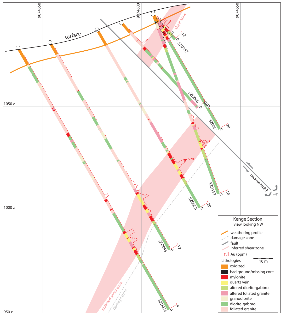
Figure 5.13 – Cross section of Kenge with lithology logs parallel to diamond drill hole traces. Note inferred reverse fault offsetting the interpreted mylonitic shear zone.
