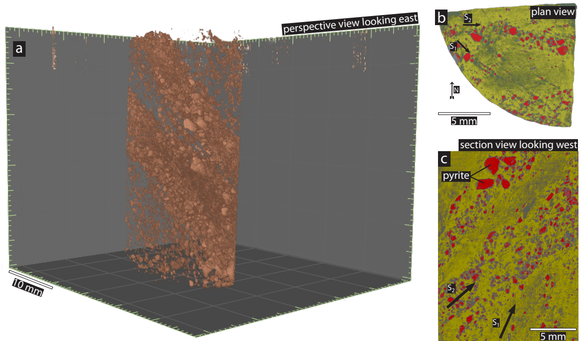
Figure 5.17 – (a) Perspective view of a 3-D X-ray CT model of a Au-bearing mylonite ¼ core sample from Mbenge. Pyrite is isolated based on density and shows the distribution closely follows the mylonitic foliation and associated shear band cleavage; (b) plan view of the same CT model with colors based on relative mineral density (yellow and grey are low density minerals and correspond to muscovite, chlorite, quartz and calcite; whereas red represents high density phases and corresponds to pyrite ± Au); (c) section view of the same CT model with colors based on relative density (same as previous).
