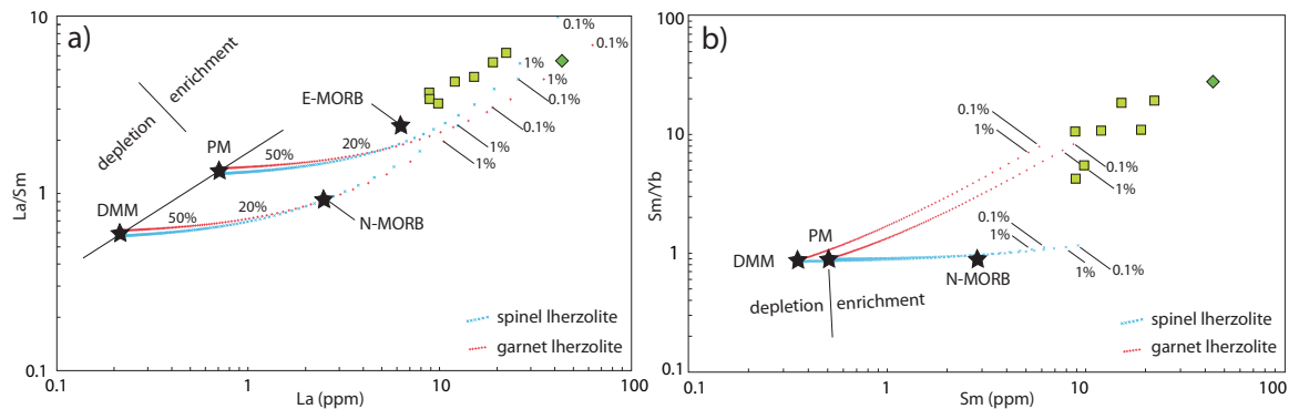
Figure 2.9 – (a) La vs. La/Sm plot of diorite-gabbro suite. (b) Sm vs. Sm/Yb plot of diorite gabbro suite. Melting curves are from the non-modal batch melting equations of Shaw (1970). The modelling used spinel lherzolite (with mode = olivine 53 + orthopyroxene 27 + clinopyroxene 17 + spinel 3 ; melt mode = olivine 6 + orthopyroxene 28 + clinopyroxene 67 + spinel 11 ; Kinzler, 1997) and garnet lherzolite (with mode = olivine 60 + orthopyroxene 20 + clinopyroxene 10 + garnet 10 ; melt mode = olivine 3 + orthopyroxene 16 + clinopyroxene 88 + garnet 9 ; Walter, 1998) sources with depleted mantle (DMM; McKenzie and O’Nions, 1991) and primitive mantle (PM; Sun and McDonough, 1989) compositions. Mineral/matrix partition coefficients are from McKenzie and O’Nions (1991). N-MORB and E-MORB compositions were taken from Sun and McDonough (1989). The solid line represents the mantle array and is defined using the DMM and PM compositions. Lithology sample symbols are the same as Fig. 2.6.
