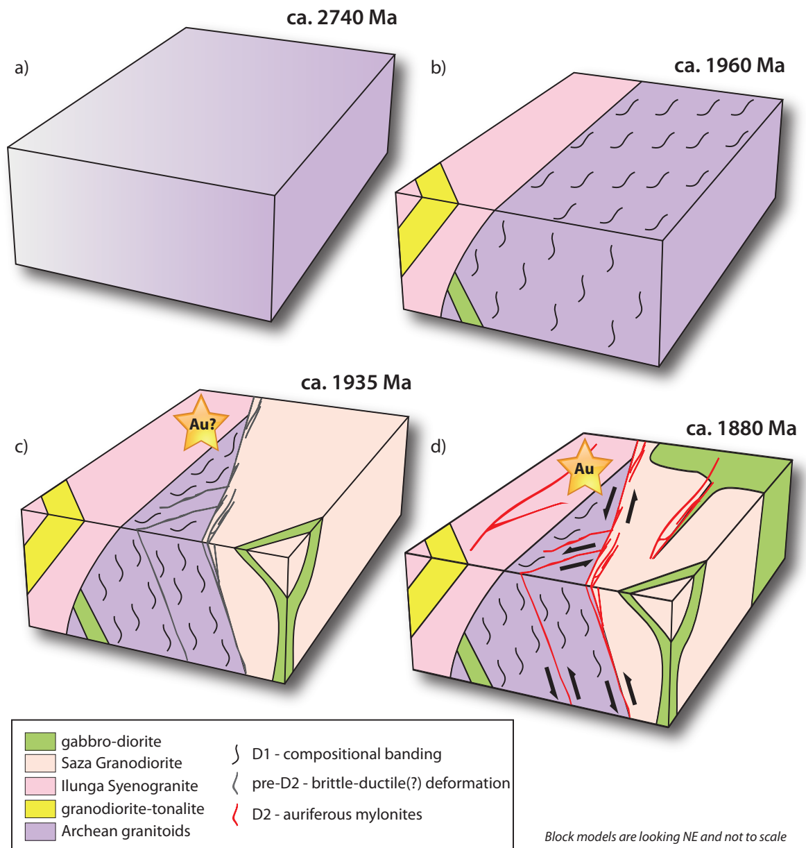
Figure 7.3 – Schematic block models showing the geologic evolution of the Lupa goldfield from the Archean to the Paleoproterozoic (based on U-Pb and Re-Os ages presented in Chapters Two, Four and Six). The geologic history of the Lupa extends beyond the Paleoproterozoic (e.g., Meso- and Neoproterozoic Re-Os ages, Neoproterozoic and Paleozoic U-Pb lower intercept ages, faulting cross cutting ca. 1880 Ma shear zones, etc.), however the timing and characteristics of these events remain poorly understood. See text for more details.
