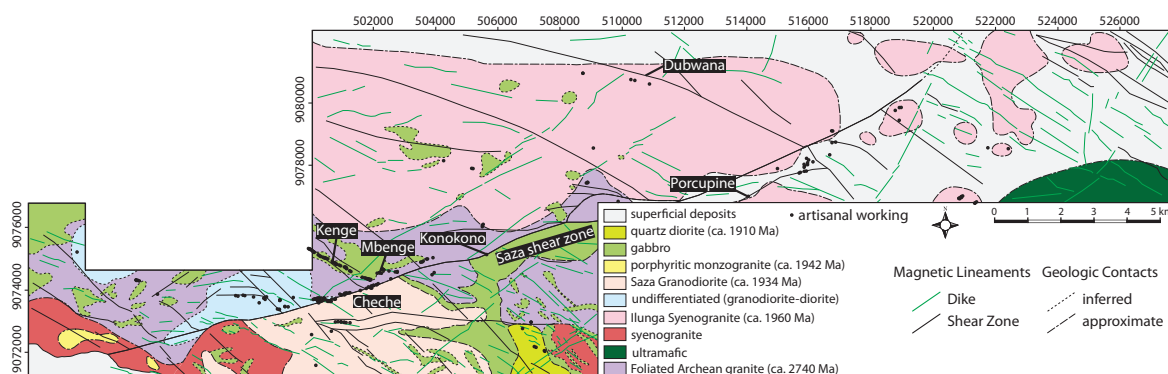
Figure 4.2 – Simplified local geology map showing the location of Kenge, Mbenge, Konokono, Porcupine and Dubwana exploration targets. Artisanal workings visited during field seasons in 2010 and 2011 are also shown (closed circles) and do not include alluvial workings, which are present in the majority of rivers in the field area. Eastings and northings are reported as UTM coordinates (WGS84, Zone 36S). Approximate lithologic contacts are based on a series of river traverses by the first author. Inferred lithologic contacts are based on unpublished aeromagnetic and radiometric surveys acquired from Helio Resource Corp. Shear zone locations are based, in part, on mapping and correspond to negative magnetic anomalies, whereas dikes are buried and interpreted from linear magnetic highs.
