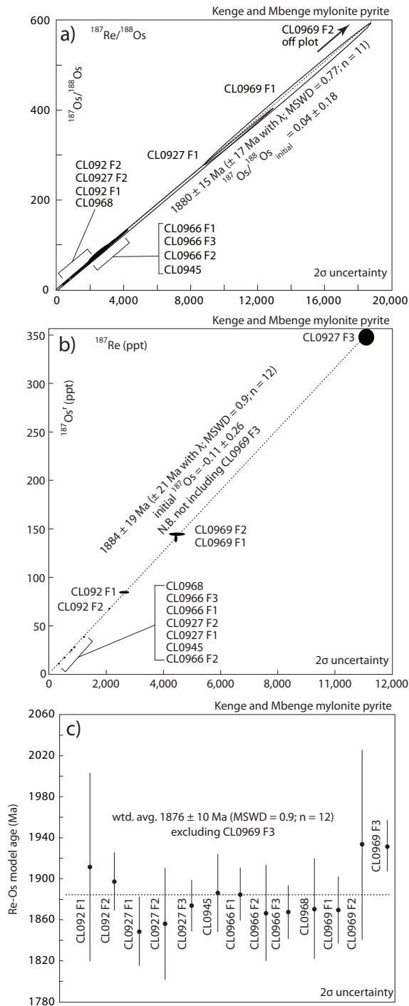
Figure 4.5 – (a) Model 1 York regression ^{187}\text{Re}/^{188}\text{Os} vs. ^{187}\text{Os}/^{188}\text{Os} isochron of pyrite samples from mylonitic shear zones at Kenge (CL0945, CL0927, CL0966, CL0968 and CL0969) and Mbenge (CL092). Analyses with exceptionally high ^{187}\text{Re}/^{188}\text{Os} ratios possess large correlated uncertainties and are typical of LLHR samples; (b) Model 2 York regression ^{187}\text{Re} vs. ^{187}\text{Os}^* isochron of pyrite samples from mylonitic shear zones at Kenge; (c) Re-Os pyrite model ages for samples from mylonitic shear zones at Kenge with weighted average Re-Os pyrite model age.
