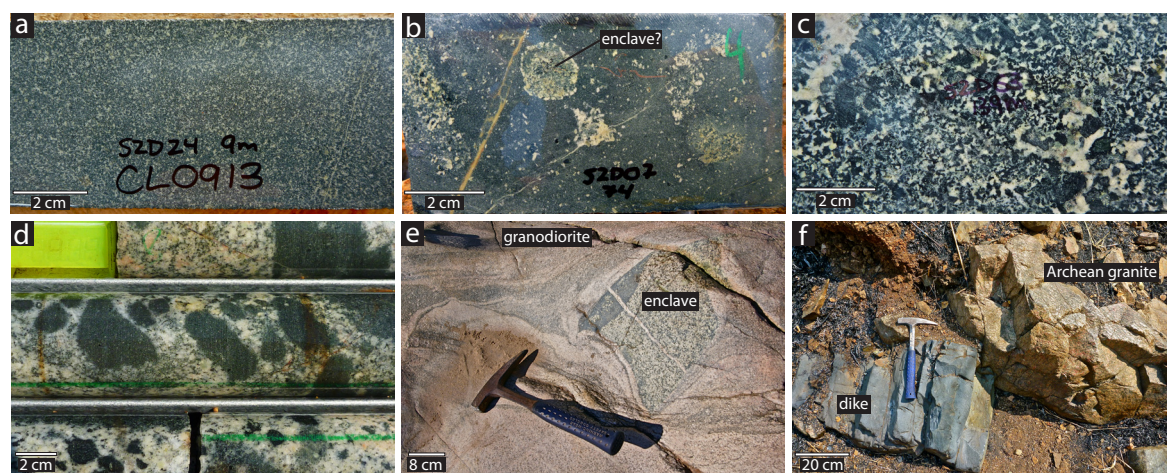
Figure 2.5 – (a) Typical example of the diorite-gabbro suite in core; (b) finer grained example of diorite-gabbro suite with more felsic enclaves; (c) plagioclase-amphibole intergrowths in diorite; (d) core photo of an example of the undifferentiated diorite-gabbro-granodiorite unit (Fig. 2.2) showing variable grain-size and modal mineralogy at hand sample scale; (e) complex and poly-phase mafic enclave hosted by granodiorite. Note ductile flow evidence around the enclave; (f) late fine-grained and alkaline dike (CL0956) cross cutting foliated Archean granitoid.
