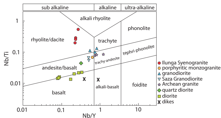
Figure 2.7 – Trace element rock classification diagram (modified from Pearce, 1996a). See text for discussion.
