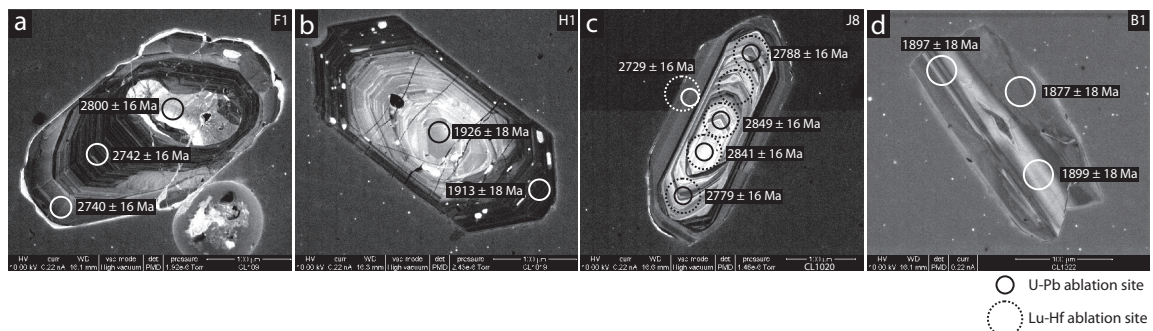
Figure 2.12 – (a) Cathodoluminescence image of zircon F1 from CL109 showing ablation spots and concordant ^{207}\text{Pb}/^{206}\text{Pb} ages; (b) cathodoluminescence image of zircon H1 from CL109 showing ablation spots and concordant ^{207}\text{Pb}/^{206}\text{Pb} ages; (c) cathodoluminescence image of zircon J8 from CL1020 showing U-Pb and Lu-Hf ablation spots and concordant ^{207}\text{Pb}/^{206}\text{Pb} ages; (e) cathodoluminescence image of zircon B1 from CL1022 showing ablation spots and concordant ^{207}\text{Pb}/^{206}\text{Pb} ages.
