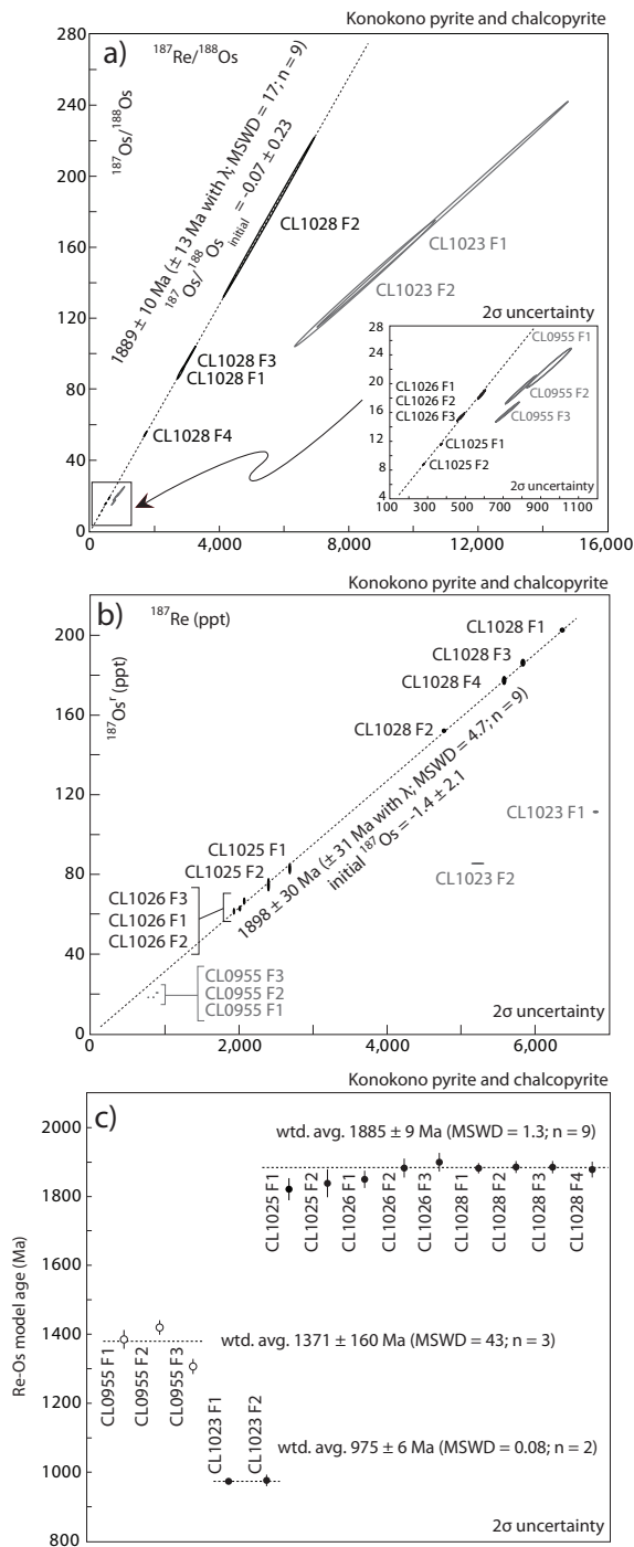
Figure 4.7 – (a) Model-3 York regression ^{187}\text{Re}/^{188}\text{Os} vs. ^{187}\text{Os}/^{188}\text{Os} isochron of pyrite samples (CL1023, CL1025, CL1026 and CL1028) and one chalcopyrite sample from Konokono. Two samples (CL1023 and CL0955) plot significantly off the regression defined by the other analyses and are not included in the isochron regression calculation (plotted in grey); (b) Model-2 York regression ^{187}\text{Re} vs. ^{187}\text{Os}^r isochron of pyrite and chalcopyrite samples from Konokono. Two samples (CL1023 and CL0955) plot significantly off the regression defined by the other analyses and are not included in the isochron regression calculation (plotted in grey); (c) Re-Os pyrite and chalcopyrite model ages for samples from Konokono. Weighted average Re-Os model ages are calculated for each of the interpreted sample sets.
