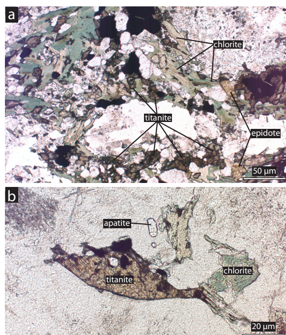
Figure 6.2 – Plane polarized light photomicrographs: (a) photomicrograph of titanite associated with greenschist facies metamorphic mineral assemblage and tectonic fabric (SZD23 at 32m); (b) euhedral titanite crystal from CL0975 (500237 / 9071994).
