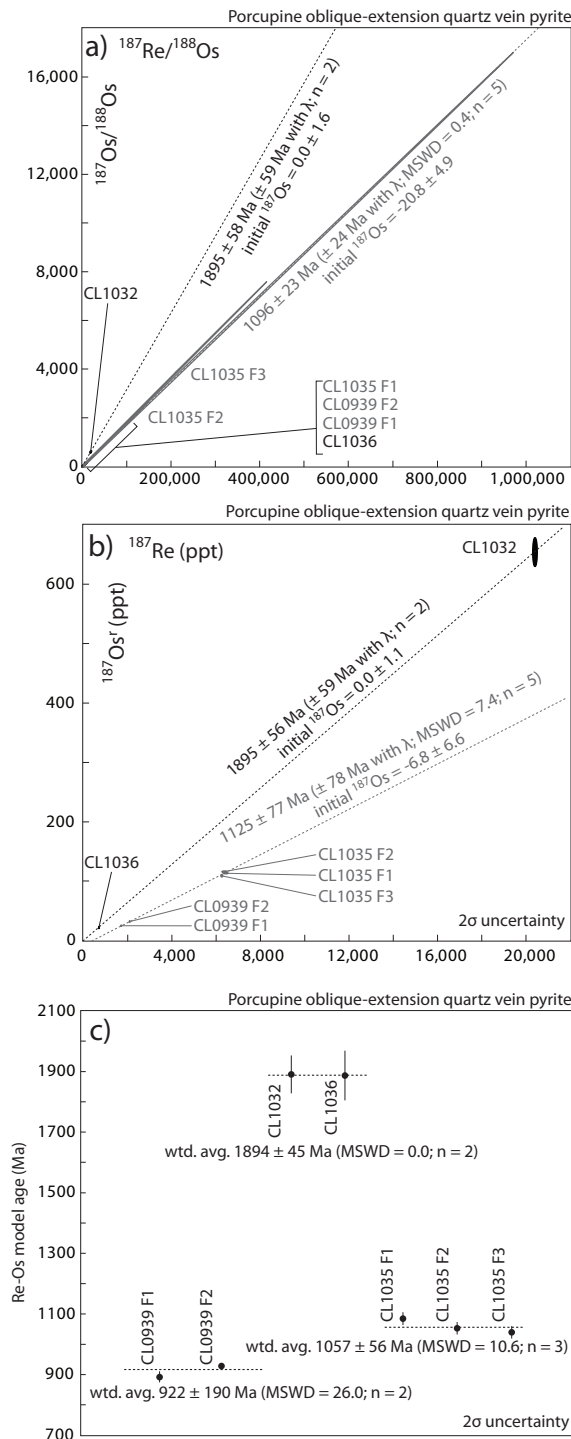
Figure 4.8 – (a) Model 1 York regression ^{187}\text{Re}/^{188}\text{Os} vs. ^{187}\text{Os}/^{188}\text{Os} isochron plot of pyrite samples from oblique-extension veins at Porcupine. Two samples (CL1032 and CL1036) yield an isochron age that is in good agreement with ages reported for Kenge, Mbenge and Konokono, whereas two samples (CL0939 and CL1035) plot significantly below the regression defined by the other two samples and yield a younger isochron age (plotted in grey); (b) Model-2 York regression ^{187}\text{Re} vs. ^{187}\text{Os}^r isochron plot of pyrite from oblique-extension veins at Porcupine. Two samples define a Mesoproterozoic isochron age (CL0939 and CL1035; plotted in grey) that contrast with the Paleoproterozoic age of the other two samples (CL1032 and CL1036); (c) Re-Os pyrite model ages hosted by oblique-extension veins at Porcupine. Weighted average Re-Os pyrite model ages are calculated for each of the interpreted sample sets.
