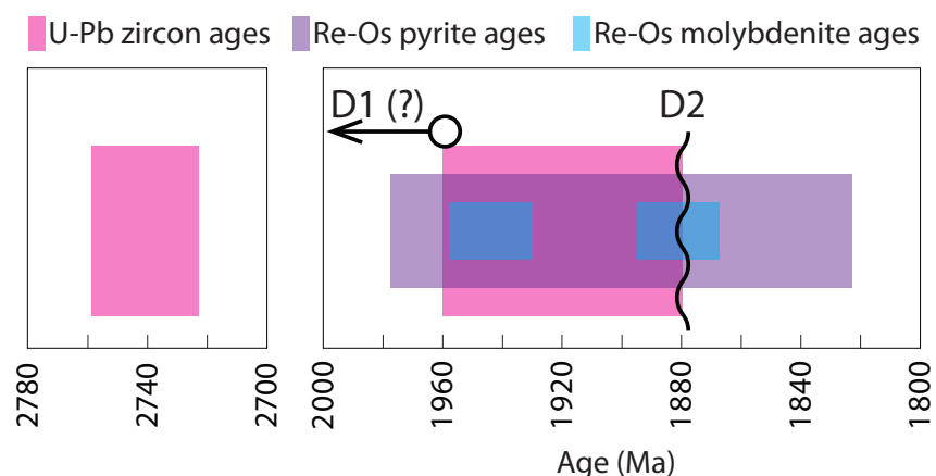
Figure 7.2 – Diagram summarizing the U-Pb and Re-Os age ranges reported in Chapters Two and Four. Note the broad temporal overlap between magmatism and mineralization.
