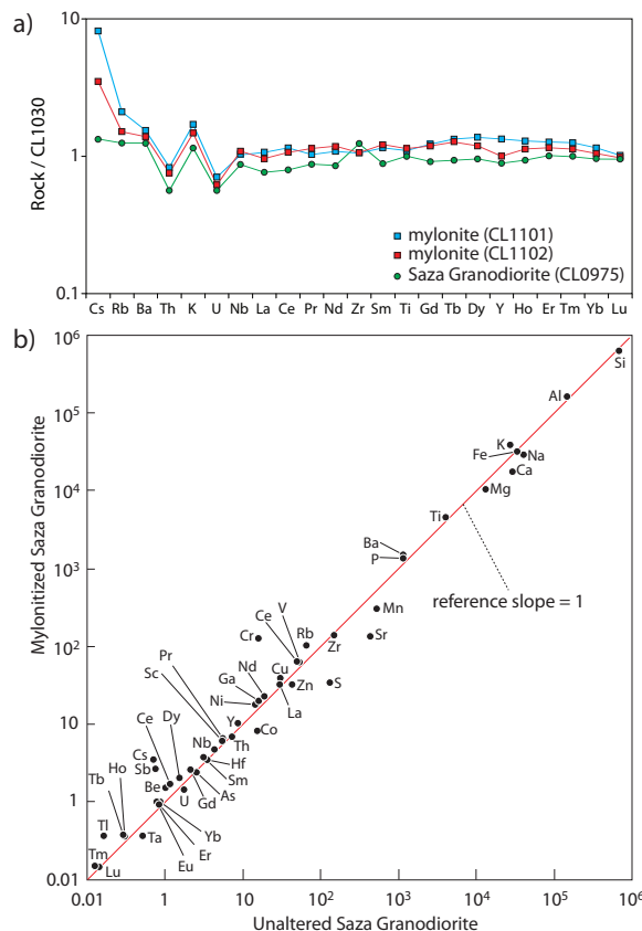
Figure 5.10 – (a) Trace element plot normalized to unaltered Saza Granodiorite sample CL1030. Note trace element homogeneity between all 4 samples except for large ion lithophile elements (e.g., Cs, Rb, Ba); (b) Diagram comparing the concentrations of elements in mylonitized Saza granodiorite and unaltered Saza Granodiorite. Elements concentrations are average values based on 2 samples of mylonitized and unaltered Saza Granodiorite. Major element oxide analyses were converted to elemental parts per million. Solid line represents the unit slope (slope = 1) and defines constant composition.
