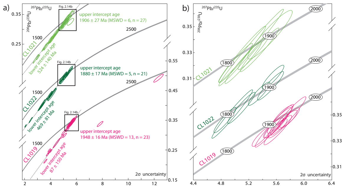
Figure 2.14 – (a–b) Concordia plots of all Proterozoic LA-MC-ICP-MS zircon analyses and concordant ( >95\% concordance) analyses, respectively. See text for discussion.
