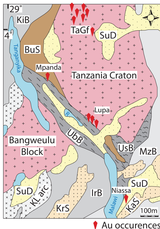
Figure 6.1 – Simplified regional geology map showing the location of goldfields in East Africa relative to Archean Cratons and Proterozoic mobile Belts (modified from CCGM/CGMW, 2002; UbB = Ubendian Belt; UsB = Usagaran Belt; KiB = Kibaran Belt; IrB = Irumide Belt; MzB = Mozambique Belt; KL arc = Katangan-Lufilian Arc; KaS = Karoo sedimentary rocks; BuS = Bukoban sedimentary rocks; SuD = surficial deposits; R = Lake Rukwa).
