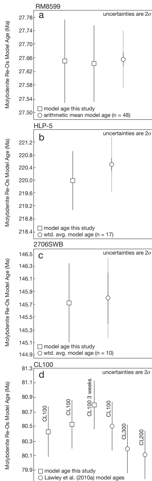
FIG. 2. (a) Molybdenite Re-Os model ages of RM8599 after exposure to HF and accepted age from Markey et al. (2007). Dotted error bars on arithmetic mean model age represent the typical uncertainty for an individual analysis. (b) Molybdenite Re-Os model age of HLP-5 after exposure to HF and accepted age from Selby and Creaser (2004). Dotted error bars on the weighted average model age represent the typical uncertainty for an individual analysis. (c) Molybdenite Re-Os model age of 2706SWB after exposure to HF and accepted age from Selby and Creaser (2004). Dotted error bars on the weighted average model age represent the typical uncertainty for an individual analysis. (d) Molybdenite Re-Os model ages of CL100 after exposure to HF and previously reported ages from Lawley et al. (2010a).
