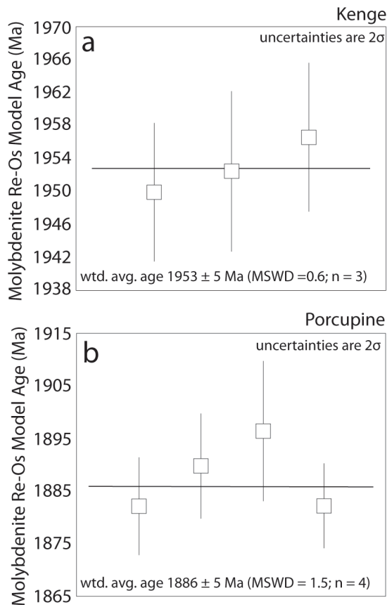
Figure 3.3 – (a) Molybdenite Re-Os model ages of ultra-fine molybdenite samples from the Kenge deposit. All three analyses provide a weighted average molybdenite Re-Os model age of 1953 \pm 5 Ma (MSWD = 0.6; n = 3); and (b) molybdenite Re-Os model ages of ultra-fine molybdenite samples from the Porcupine deposit. All four analyses provide a weighted average molybdenite Re-Os model age of 1886 \pm 5 Ma (MSWD = 1.5; n = 4).
