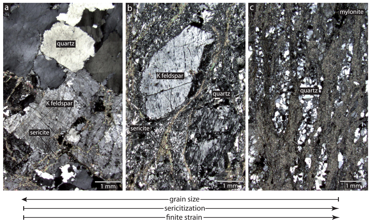
Figure 5.18 – (a–c) Crossed nicols photomicrographs of three Ilunga Syenogranite samples exhibiting various degrees of hydrothermal alteration and finite strain. Our proposed model for shear zone development would place these three samples into a progressive sequence from left to right. (a) Coarse grained, non-foliated and relatively unaltered granite becomes hydrothermally altered, potentially due to pre-D2 brittle fracturing, and results in the replacement of feldspars with intrinsically weaker phyllosilicates (GPD44 at 251m); (b) continued hydrothermal promotes strain localization within the altered granite and leads to increasing finite strain and mylonitization (505500, 9081129); (c) complete replacement of feldspars with further grain size reduction producing a quartz-phyllosilicate mylonite (508512, 9080975)
