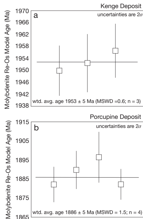
FIG. 3. (a) Molybdenite Re-Os model ages of ultrafine molybdenite samples from the Kenge deposit. (b) Molybdenite Re-Os model ages of ultrafine molybdenite samples from the Porcupine deposit.
