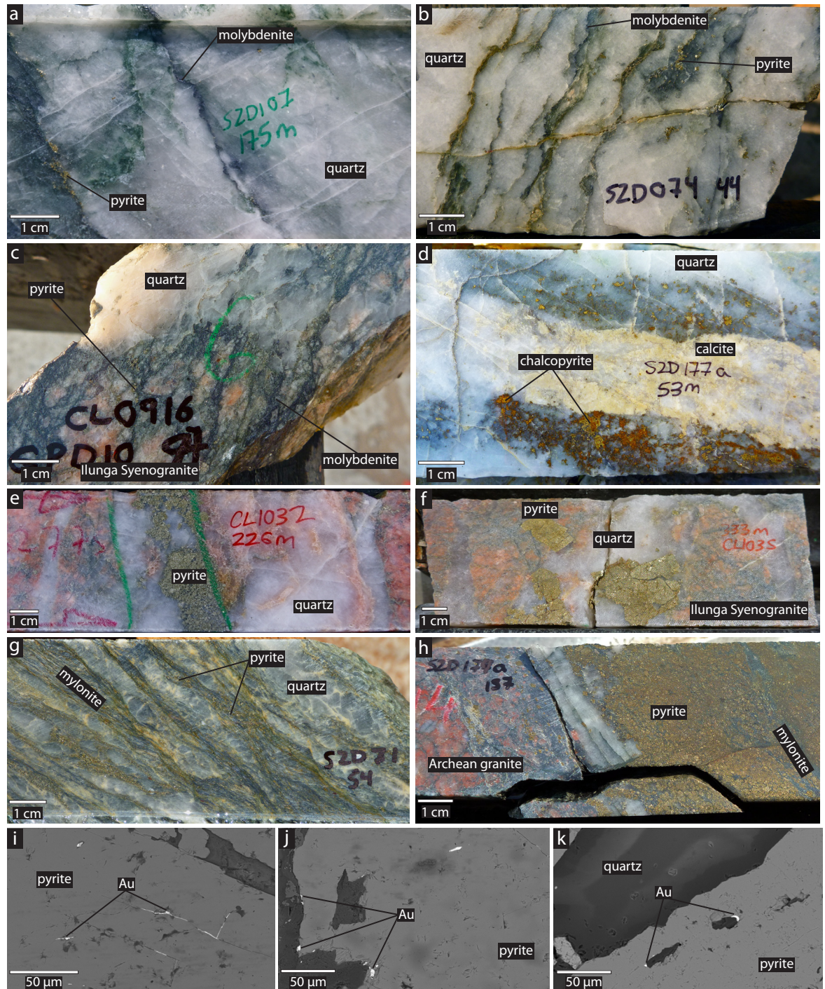
Figure 4.3 – (a) molybdenite stylolite-like vein hosted by fault-fill vein at Mbenge; (b) pyrite and molybdenite stylolite-like veins within fault-fill veins at Mbenge; (c) molybdenite hosted by sheared Ilunga Syenogranite at Porcupine; (d) complex vein relationships at Konokono showing chalcopyrite-bearing quartz vein (with vein margins not shown) cross cut by unmineralized quartz-calcite vein. Narrow quartz-calcite veins are observed extending from the wider quartz-calcite vein at high-angles; (e) pyrite hosted by quartz veins in hydrothermally altered Ilunga Syenogranite at Porcupine; (f) pyrite hosted by quartz vein in hydrothermally altered Ilunga Syenogranite that is paragenetically similar to Fig. 4.2e, but records anomalously younger ages; (g) pyrite hosted by sulfidized mylonitic shear zone at Kenge; (h) pyrite hosted by sulfidized mylonitic shear zone, quartz vein, and Archean granite wall rock at Konokono; (i) scanning electron microscope (SEM) images of Au observed as pyrite inclusions and fracture fills (SZD23 at 107 m); (j) scanning electron microscope (SEM) images of Au observed on the margins and as inclusions within pyrite (SZD23 at 107 m); (k) scanning electron microscope (SEM) images of Au observed as pyrite inclusions (SZD71 at 53 m).
