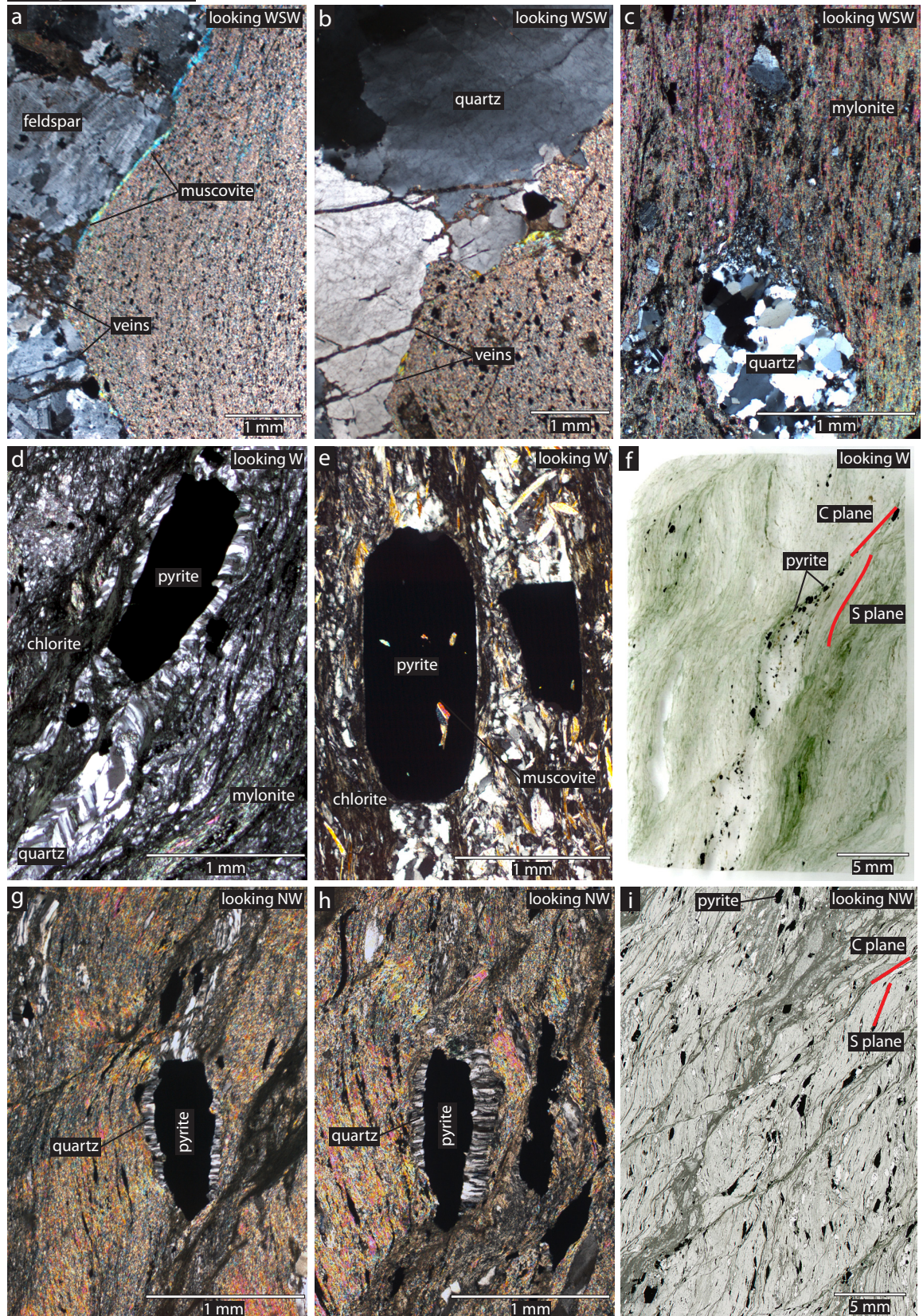
Figure 5.7 – Section view photomicrographs of Porcupine (a–c), Mbenge (d–f), and Kenge (g–i): (a) crossed nicols photomicrograph of sharp and undulating mylonite-granite contact cross cutting muscovite \pm calcite \pm chlorite veins (GPD44 at 211m); (b) crossed nicols photomicrographs of sharp and undulating fault-fill vein-mylonite contact cross cutting muscovite \pm calcite \pm chlorite veins (GPD44 at 212m); (c) crossed nicols photomicrograph of quartz porphyroclasts (GPD44 211 m); (d) pyrite with quartz strain fringes (SZD74 at 58m); (e) crossed nicols photomicrograph of muscovite included within a pyrite crystal that is concordant with mylonitic foliation
