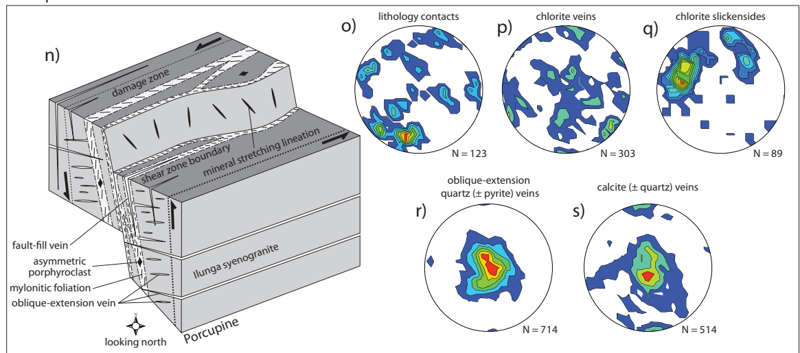
Figure 5.16 – (a) Schematic block model of Kenge summarizing structural fabrics; (b–g) lower hemisphere equal area contoured stereonet plots of planar and linear fabrics measured from oriented core at Kenge SE; (h–m) lower hemisphere equal area contoured stereonet plots of planar and linear fabrics measured from oriented core at the Mbenge; (n) schematic block model of Porcupine summarizing structural fabrics; (o–s) lower hemisphere equal area contoured stereonet plots of planar and linear fabrics measured from oriented core at Porcupine. All contours are plotted following the 1% area method using OSX Stereonet (v 1.4; contour intervals set at 1).
