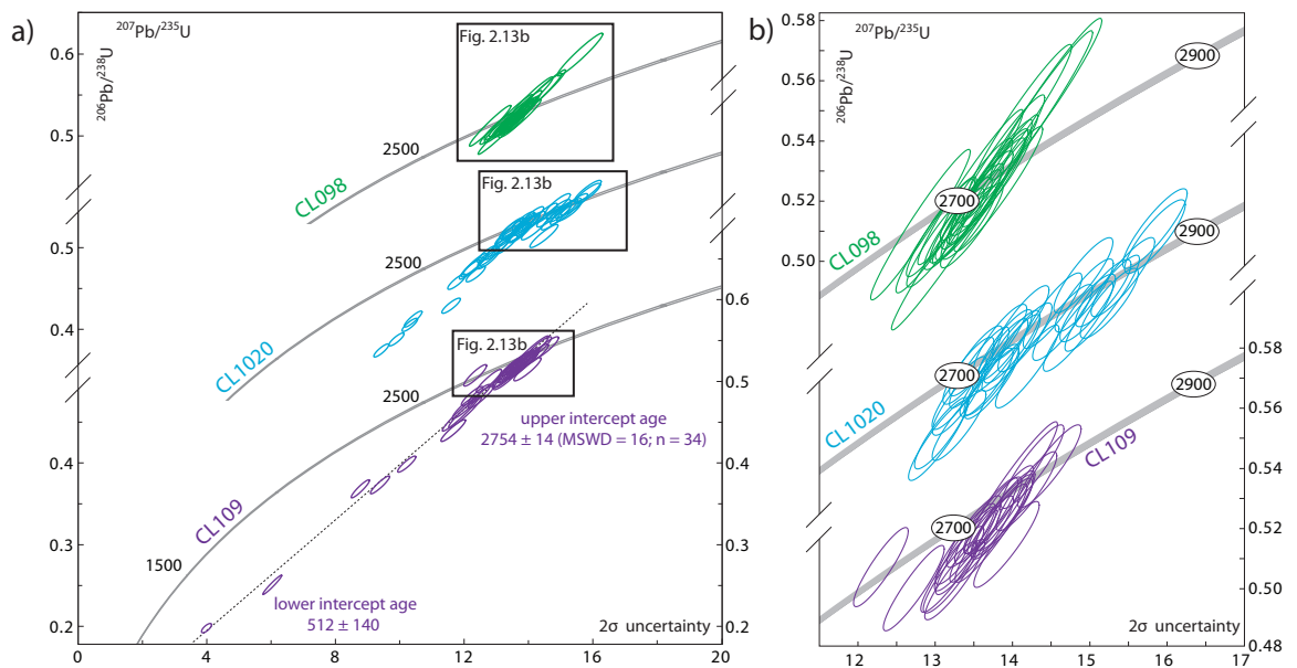
Figure 2.13 – (a,b) Concordia plots of all Archean LA-MC-ICP-MS zircon analyses and concordant (>95% concordance) analyses, respectively. See text for discussion.
