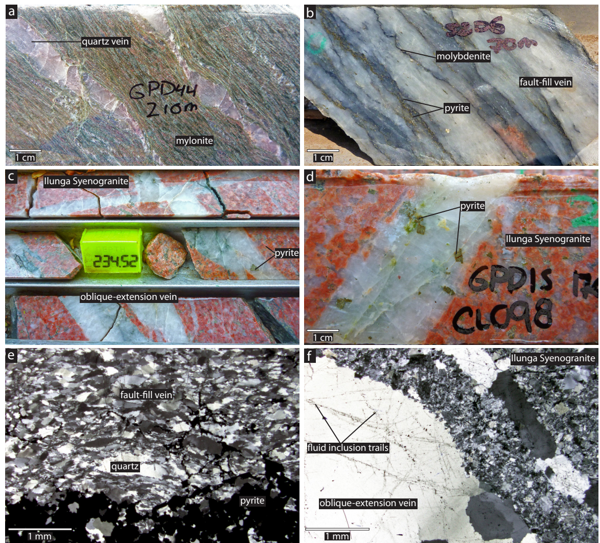
Figure 5.12 – Quartz vein photos from non-oriented core: (a) boudinaged and potentially transposed quartz veins hosted by mylonitic shear zone at Porcupine; (b) fault-fill vein at Saza shear zone showing stylolite-like sulfide stringer veins; (c) oblique-extension veins at Porcupine; (d) oblique-extension vein at Porcupine; (e) crossed nicols photomicrograph of fault-fill quartz vein. Note flattening and sub-grain rotation (SZD23 at 107m); (f) oblique extension vein at Porcupine. Not less deformed nature of quartz compared to fault-fill veins (GPD1 at 54m).
