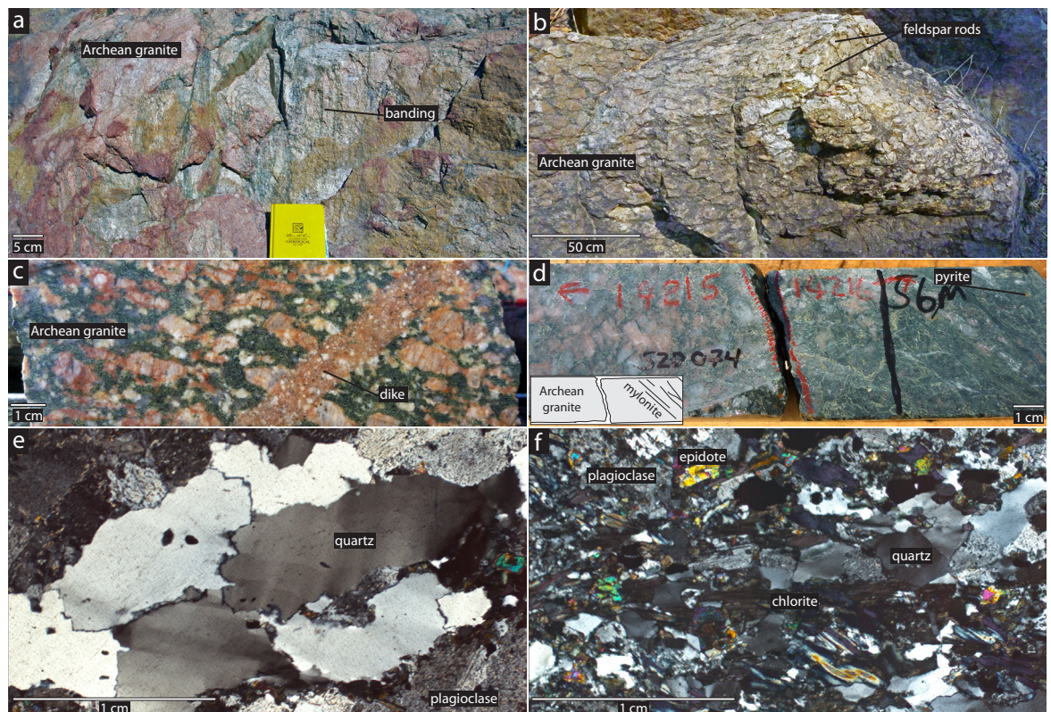
Figure 5.4 – (a–b) field photos of Archean granite highlighting the variability in structure and grain size of the lithologic unit; (c–d) core photos of the Archean granite cross cut by a non-foliated porphyritic dikes and mylonitic fault rocks (D2) cross cutting pre-existing foliation (D1); (e) crossed nicols photomicrograph of Archean granite showing undulatory extinction and cusate-lobate quartz crystal boundaries; (f) crossed nicols photomicrograph of Archean granite showing alignment of chlorite and undulatory extinction in quartz. The alignment of quartz, K feldspar, and chlorite gives the rock a banded appearance in the field.
