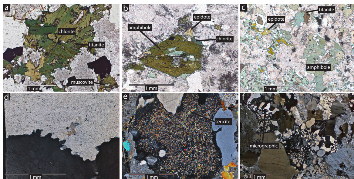
Figure 2.6 – (a) Transmitted light photomicrograph of primary Fe-Mg minerals in foliated Archean granite that have been replaced by chlorite, titanite, epidote and opaques (SZD23 at 32 m); (b) transmitted light photomicrograph of rare relict amphibole in a granodiorite dike that has been overprinted by chlorite and epidote (SZD24 at 27 m); (c) transmitted light photomicrograph of diorite dike showing characteristic mineral assemblage of amphibole, plagioclase, quartz, titanite and epidote (504690, 9075531); (d) crossed nicols transmitted light photomicrograph of recrystallized quartz grain boundaries in foliated Archean granitoid. Quartz crystals also locally possess undulatory extinction and subgrain development (SZD23 at 32 m); (e) crossed nicols transmitted light photomicrograph of sericitized plagioclase (SZD71 at 10 m); (f) crossed nicols transmitted light photomicrograph of micrographic texture in Ilunga Syenogranite. Locally, Ilunga Syenogranite samples possess gradational contacts with aplite dikes and are characterized by abundant feldspar intergrowth textures (GPD15 at 105 m).
