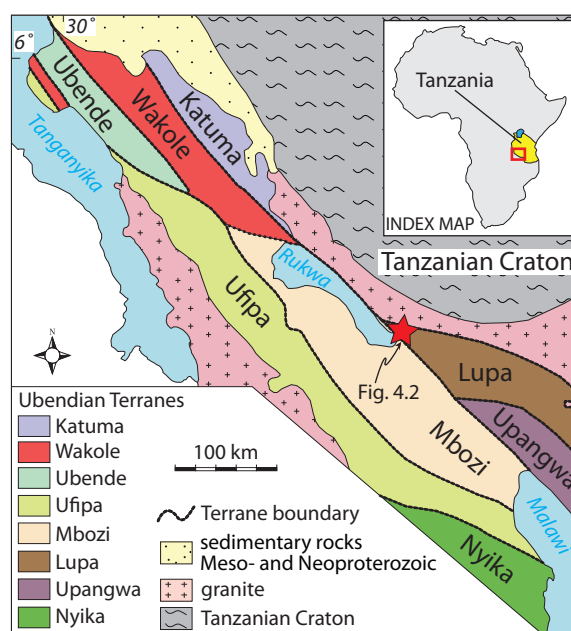
Figure 4.1 – Regional geology map of SW Tanzania showing Ubendian Terranes and the field area for the current study (modified from Daly, 1988).
