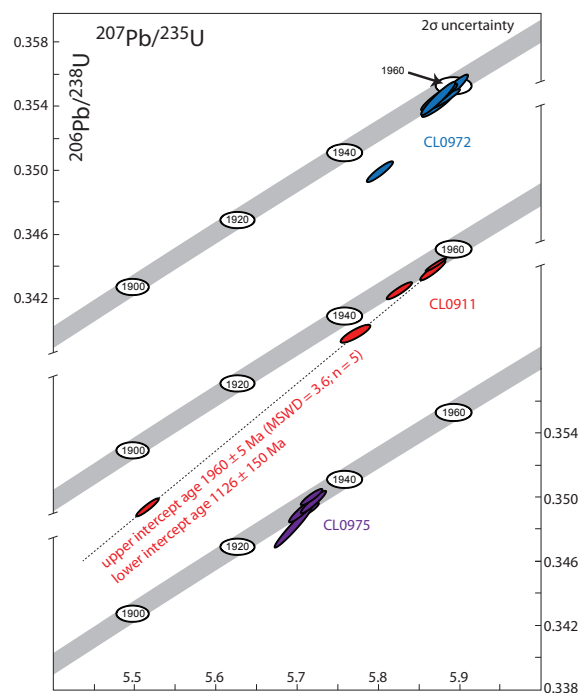
Figure 2.11 – Concordia plots for CL0911, CL0972 and CL0975, respectively. See text for discussion.
