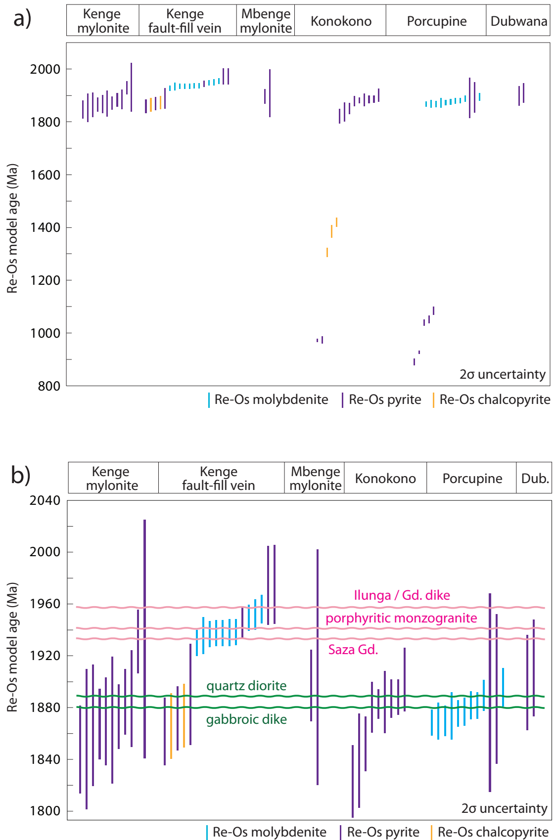
Figure 7.1 – (a) All Re-Os molybdenite (blue), pyrite (purple) and chalcopyrite (yellow) model ages reported in Chapter Four. Uncertainties are reported at 2\sigma ; (b) Paleoproterozoic Re-Os molybdenite (blue), pyrite (purple) and chalcopyrite (yellow) model ages reported in Chapter Four. Uncertainties are reported at 2\sigma . With interpreted U-Pb zircon ages, minus their associated analytical uncertainties, reported in Chapter Two (Gd. = granodiorite; Ilunga = Ilunga Syenogranite)
