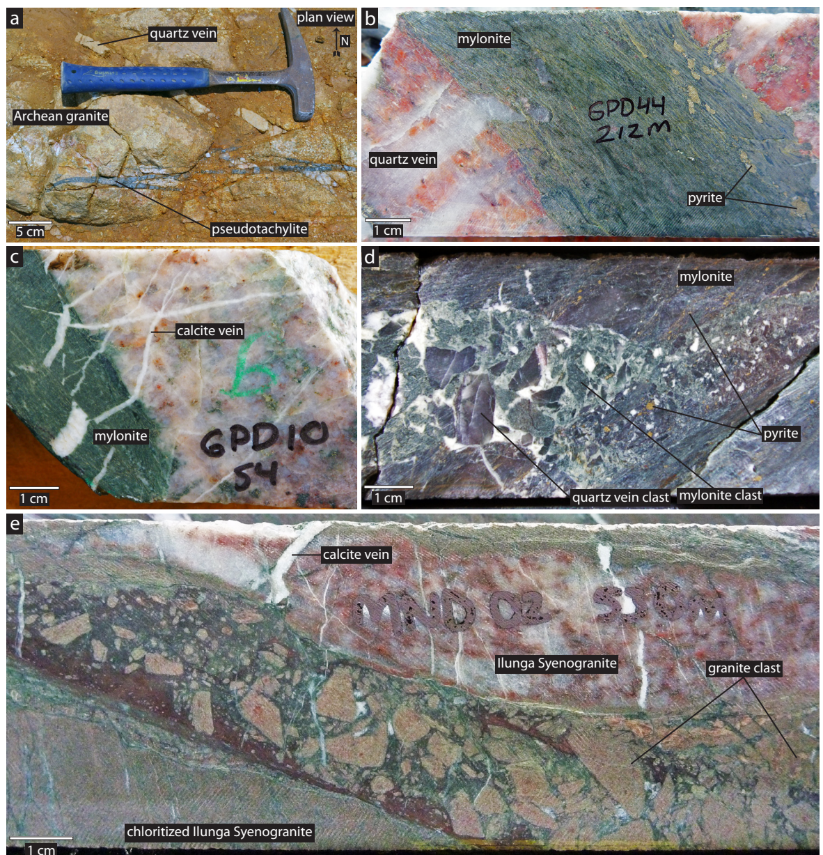
Figure 5.9 – (a) Plan view photo of suspected pseudotachylite fault rock offsetting quartz veins and cross cutting Archean foliated granite; (b) quartz veins cross cutting Ilunga syenogranite and becoming transposed sub-parallel to the mylonitic foliation; (c) calcite veins cross cutting Ilunga Syenogranite and mylonite. Calcite veins are in turn offset by later movement parallel to mylonitic foliation; (d) cataclasites cross cutting mineralized mylonite; (e) cataclasites cross cutting and containing angular to sub-rounded clasts of Ilunga Syenogranite. Note complex calcite veining.
