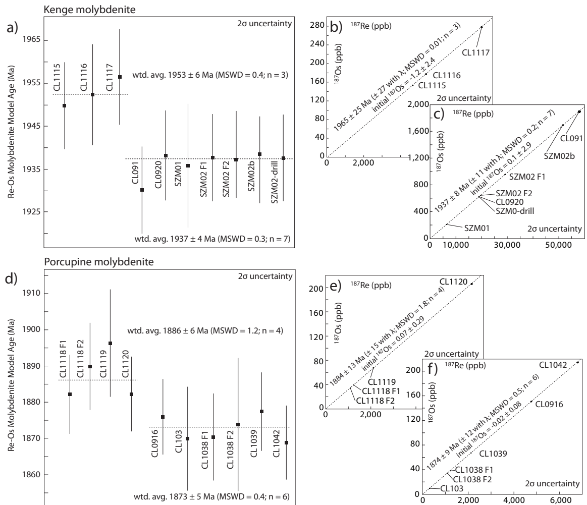
Figure 4.4 – (a) Re-Os molybdenite model age from ultrafine molybdenite samples (Chapter Three) and molybdenite from stylolite-like veins at Kenge. Weighted average (wtd. avg.) Re-Os molybdenite model age are reported for both sample sets; (b) Model 1 York regression ^{187}\text{Re} vs. ^{187}\text{Os} isochron from ultrafine molybdenite samples at Kenge; (c) Model 1 York regression ^{187}\text{Re} vs. ^{187}\text{Os} isochron of molybdenite from stylolite like veins at Kenge; (d) Re-Os molybdenite model age from ultrafine molybdenite samples (Chapter Three) and molybdenite from sheared granite samples at Porcupine. Weighted average (wtd. avg.) Re-Os molybdenite model age are reported for both sample sets; (e) Model 1 York regression ^{187}\text{Re} vs. ^{187}\text{Os} isochron of molybdenite from ultrafine molybdenite samples at Porcupine; (f) Model 1 York regression ^{187}\text{Re} vs. ^{187}\text{Os} isochron of molybdenite from sheared granite samples at Porcupine.
