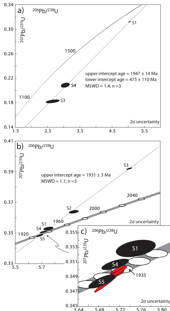
Figure 6.3 – (a) Concordia plot showing U-Pb titanite analyses and upper/lower intercept ages for sample CL109; (b) Concordia plots showing U-Pb titanite analyses (black ellipses) and upper intercept age for sample CL0975. Inset diagram shows concordant U-Pb titanite analyses and U-Pb zircon analyses (red ellipses) for CL0975 (Chapter Two).
