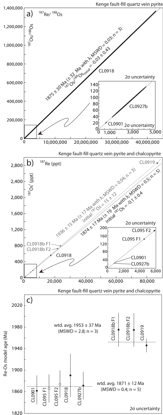
Figure 4.6 – (a) Model 1 York regression ^{187}\text{Re}/^{188}\text{Os} vs. ^{187}\text{Os}/^{188}\text{Os} isochron of pyrite samples from fault-fill veins at Kenge; (b) Model 2 York regression ^{187}\text{Re} vs. ^{187}\text{Os}^r isochron of pyrite and chalcopyrite samples from fault-fill veins at Kenge; (c) Re-Os pyrite (CL0918a, CL0918b, CL0919, CL0966b; closed circles) and chalcopyrite (CL095; open circles) model ages hosted by fault-fill veins at Kenge.
