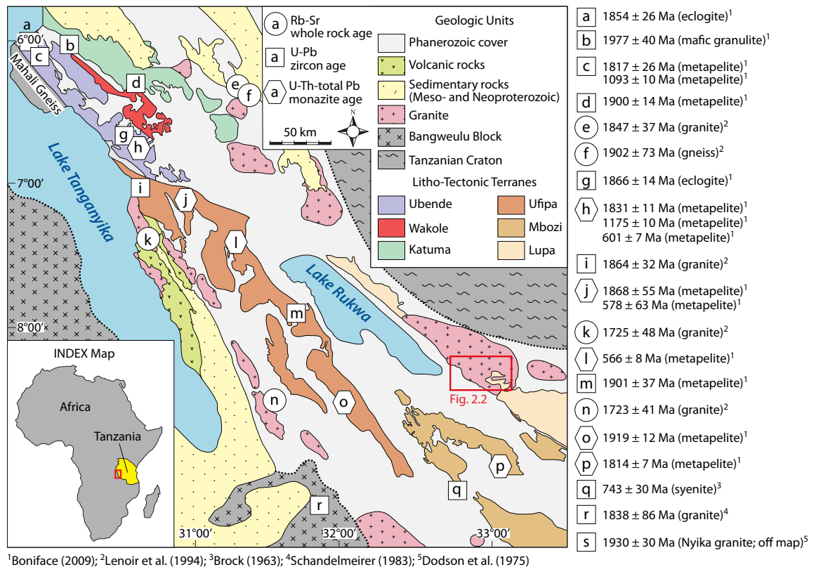
Figure 2.1 – Regional geologic map showing Ubendian Terranes and previously reported geochronology sample locations (modified from Smirnov et al., 1973).
