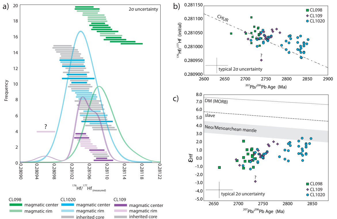
Figure 2.15 – (a) Measured ^{176}\text{Hf}/^{177}\text{Hf} ratios from CL098, CL109 and CL1020. Overlying individual analyses are the probability distributions for each sample. Samples CL098 and CL1020 possess approximately normal ^{176}\text{Hf}/^{177}\text{Hf} ratios distributions, whereas CL109 possesses a weakly bi-modal distribution. (b) Calculated ^{176}\text{Hf}/^{177}\text{Hf}_{\text{initial}} ratios for sample CL098, CL109 and CL1020 plotted against each analyses corresponding ^{207}\text{Pb}/^{206}\text{Pb} age. The CHUR evolution line and typical 2σ uncertainty for an individual analysis are also shown. (c) Calculated \epsilon\text{Hf} for samples CL098, CL109 and CL1020 plotted against the corresponding ^{207}\text{Pb}/^{206}\text{Pb} age for each analysis. DM (MORB source depleted mantle, Griffin et al., 2000), Slave Craton mantle (Pietranik et al., 2008) and Neo-Mesoarchean mantle (Shirey et al., 2008) are also plotted. The typical 2σ uncertainty on individual ^{207}\text{Pb}/^{206}\text{Pb} ages and \epsilon\text{Hf} values are also shown.
