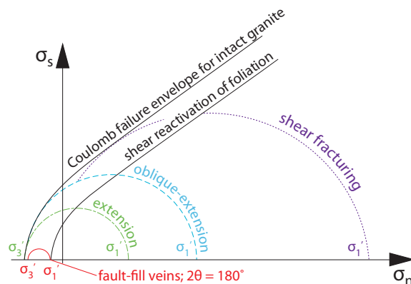
Figure 5.19 – Schematic Mohr diagram showing the geomechanics of the three main vein types at orogenic Au deposits (modified after Vearncombe, 1998). Fault-fill veins that form parallel to the mylonitic foliation requires negative effective \sigma'_1 and \sigma'_3 , low differential stress and high fluid pressure ( \sigma_n = normal stress; \sigma_s = shear stress; \sigma'_1 = maximum effective compressive stress; \sigma'_3 = minimum effective compressive stress).
