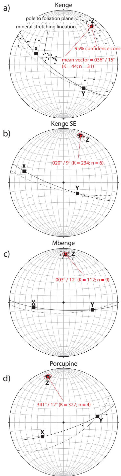
Figure 5.15 – (a–d) Lower-hemisphere equal-area stereonets of the Kenge, Kenge SE, Mbenge and Porcupine ore body geometry, respectively. The orientations of the finite strain ellipsoid axes ( X^3 Y^3 Z ; closed squares) are based on the finite strain approach (Robert and Poulsen, 2001) where the intersection of the average mylonitic foliation (black solid line) and the average shear zone boundary (black dotted line) represents the Y axis. The X axis of the finite strain ellipsoid is assumed to lie 90^\circ away from the Y axis and along the mylonitic foliation whereas the Z axis is fixed by the location of the other finite strain axes (see text for further discussion). Structural measurements are from surface exposures (closed circles = mineral stretching lineations; open circles = mylonitic foliation poles to planes; mean mylonitic foliation pole to plane = red diamond; 95% confidence interval of mean = red ellipse). K values are a measure of the tendency of linear data to fit a girdle or a cluster (K values approaching zero represent girdles, whereas K values approaching infinity represent clusters) following the approach of Woodcock and Naylor (1983).
