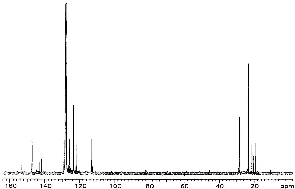
Appendix 5.8 ^{13}\text{C} -NMR spectrum of \text{Mo}(=\text{C}(\text{CH}_3)\text{-m-}
