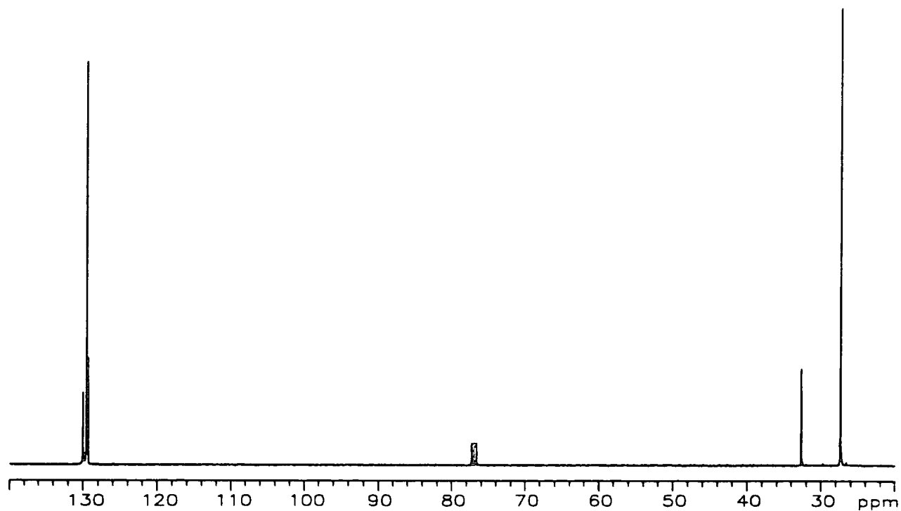
Appendix 2.2.a ^{13}\text{C} -NMR spectrum of poly(1-butenylene) initiated by \text{W}(\text{CH}^t\text{Bu})(\text{O}^t\text{Bu})_2(\text{NAr})
