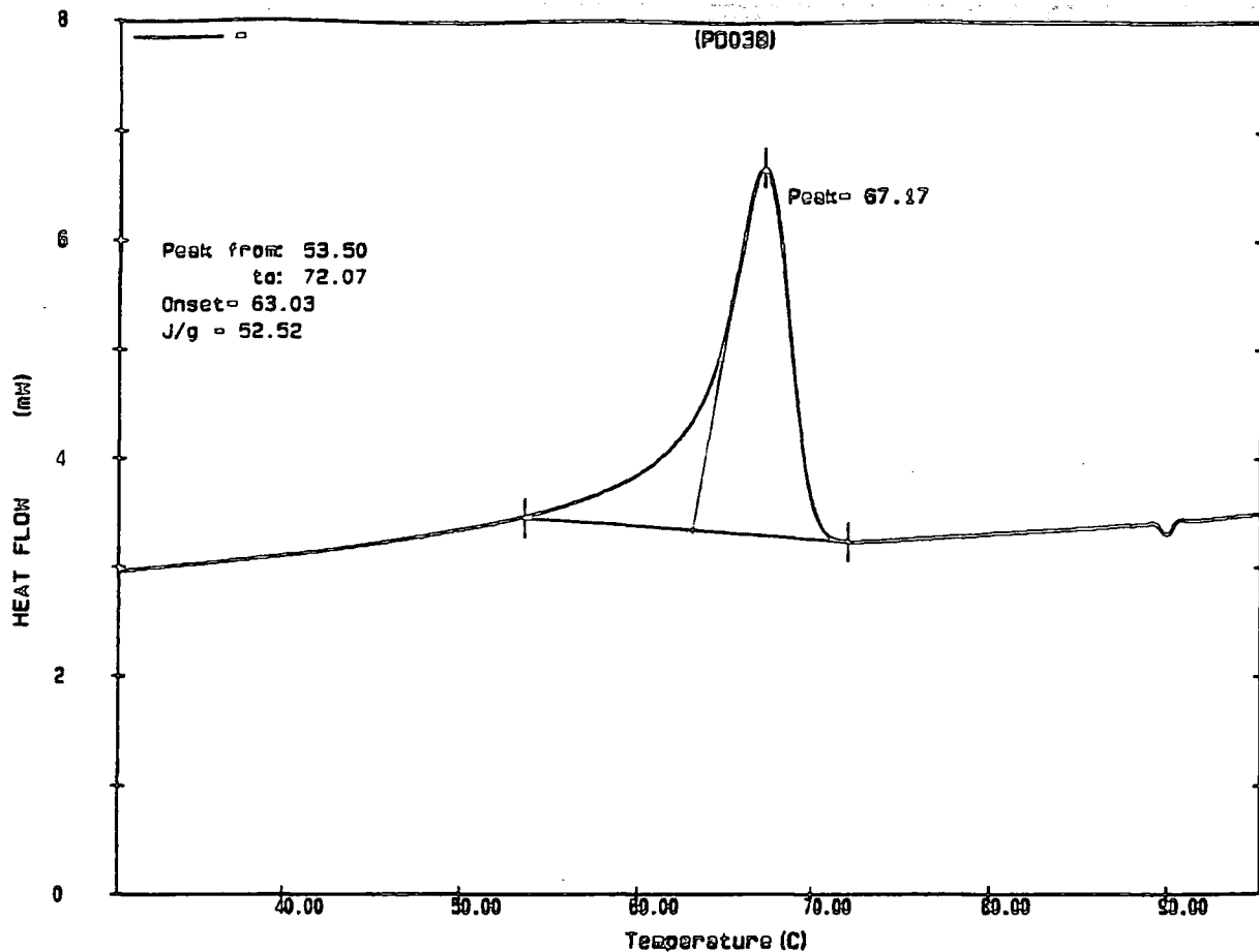
Appendix 2.27.a DSC trace of poly(1-dodecenylene) initiated with W(CH^tBu)(O^tBu)_2(NAr)
