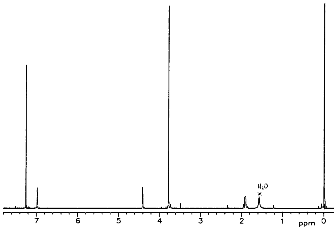
App.5.3 ^1\text{H-NMR} spectrum of compound (2)
