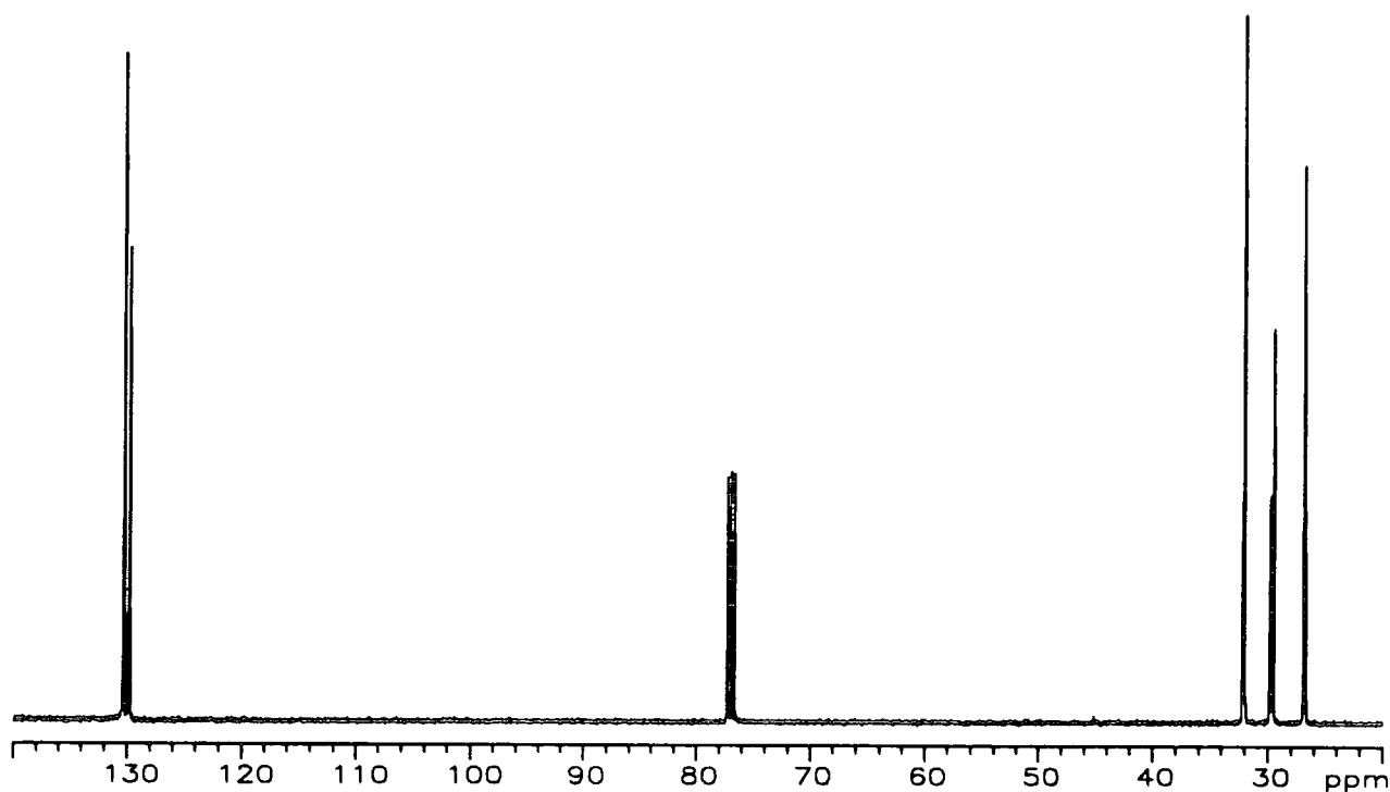
Appendix 2.8.c ^{13}\text{C} -NMR spectrum of poly(1-pentenylene) initiated by \text{Mo}(\text{CH}^t\text{Bu})(\text{OC}(\text{CH}_3)_2\text{CF}_3)_2(\text{NAr})
