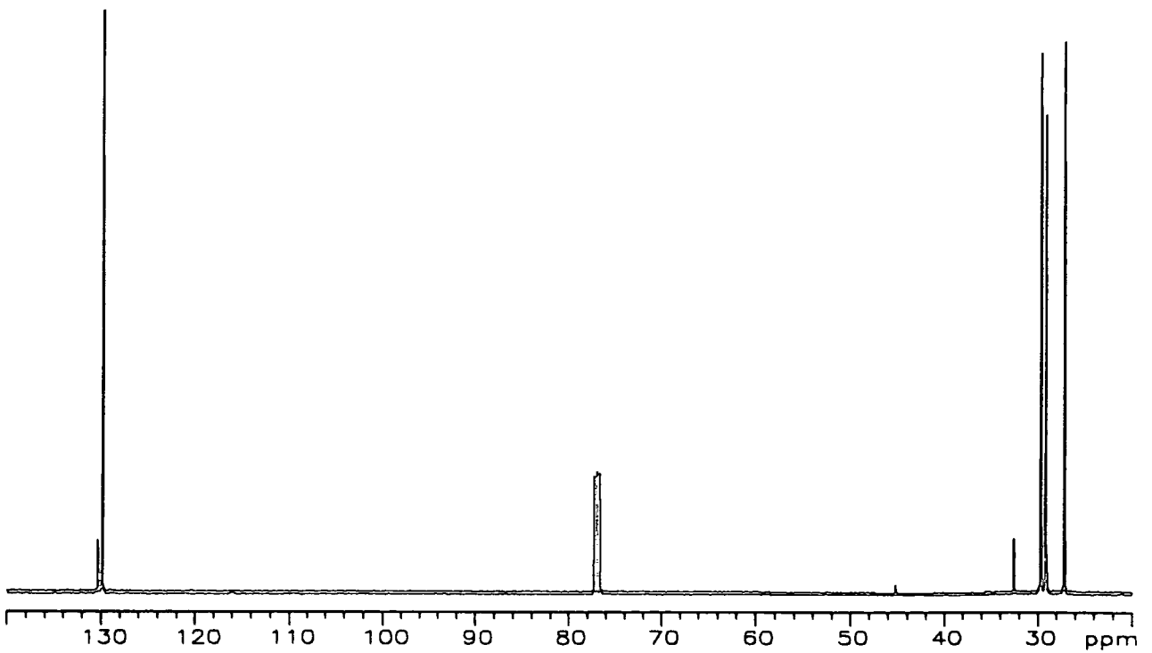
Appendix 2.16.a ^{13}\text{C} -NMR spectrum of poly(1-octenylene) initiated by \text{W}(\text{CH}^t\text{Bu})(\text{O}^t\text{Bu})_2(\text{NAr})
