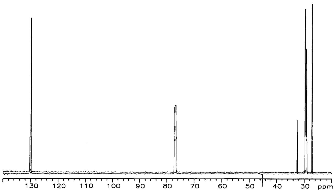
Appendix 2.16.b ^{13}\text{C} -NMR spectrum of poly(1-octenylene) initiated by \text{Mo}(\text{CH}^t\text{Bu})(\text{OC}(\text{CH}_3)_3)_2(\text{NAr})
