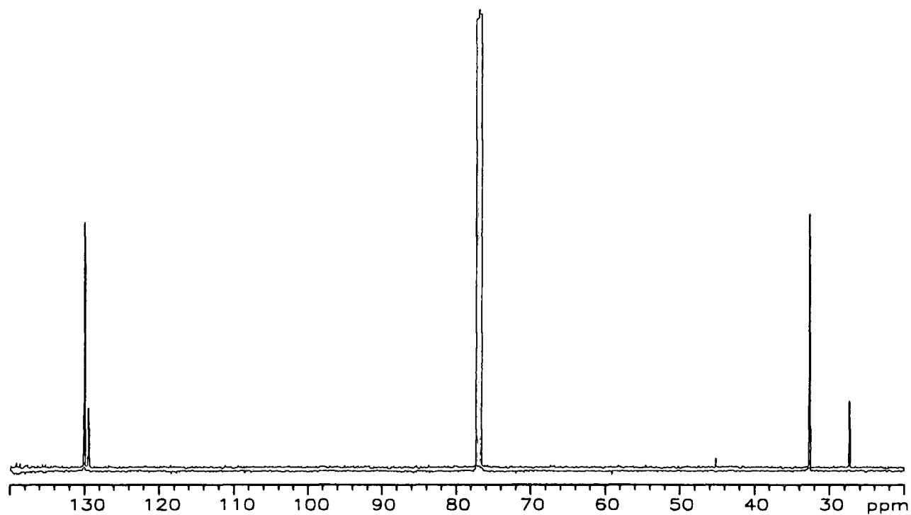
Appendix 2.2.d ^{13}\text{C} -NMR spectrum of poly(1-butenylene) initiated by \text{Mo}(\text{CH}^t\text{Bu})(\text{OC}(\text{CH}_3)(\text{CF}_3)_2)_2(\text{NAr})
