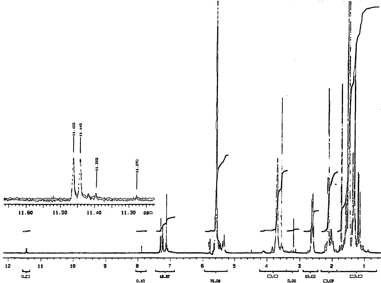
Appendix 3.1.c ^1\text{H-NMR} of the poly(bistrifluoromethylnorbornadiene)- block -poly(1-octenylene) polymerisation (3 days after addition of cyclooctene)
