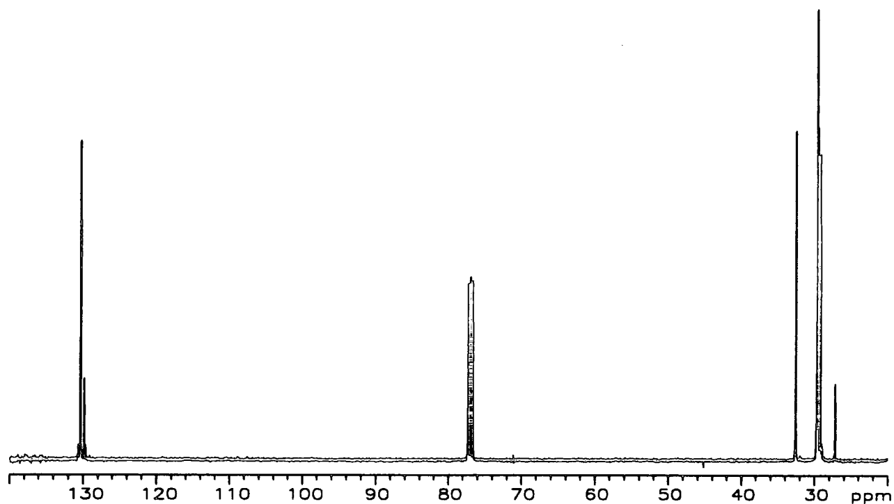
Appendix 2.25.b ^{13}\text{C} -NMR spectrum of poly(1-dodecylene) initiated by \text{Mo}(\text{CH}^t\text{Bu})(\text{OC}(\text{CH}_3)_3)_2(\text{NAr})
