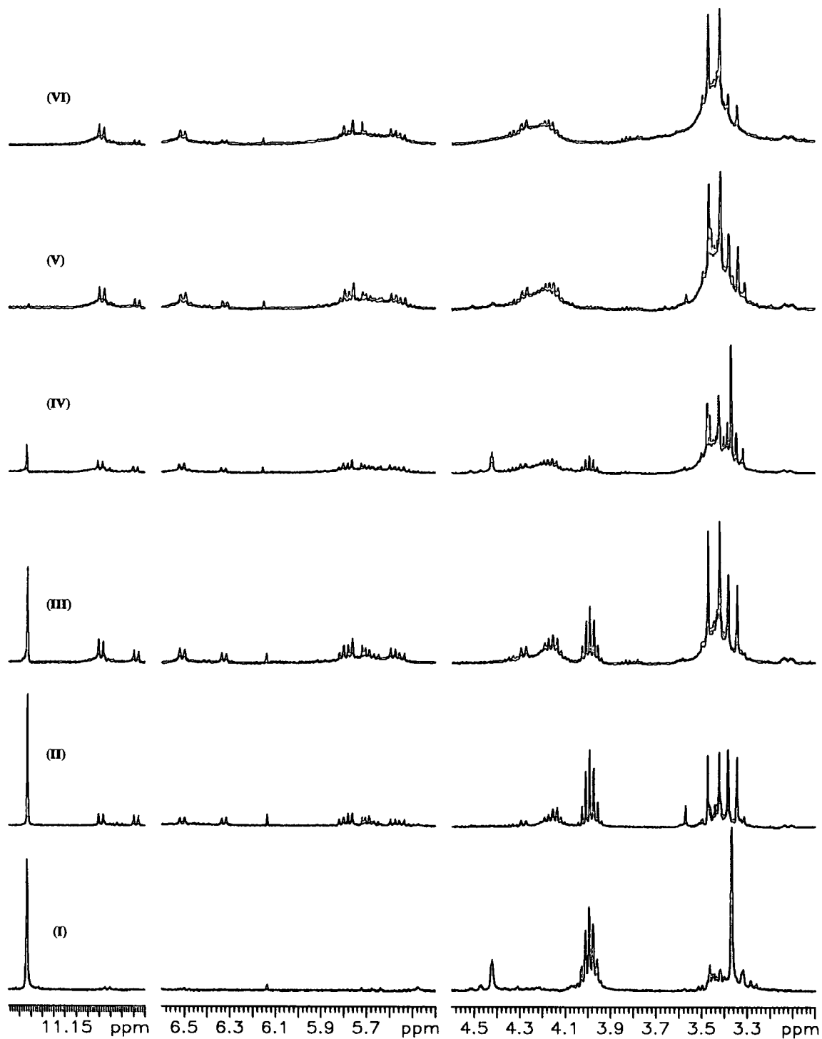
Figure 5.2.3.b ^1\text{H} NMR spectra of the ROMP reaction of (2)
