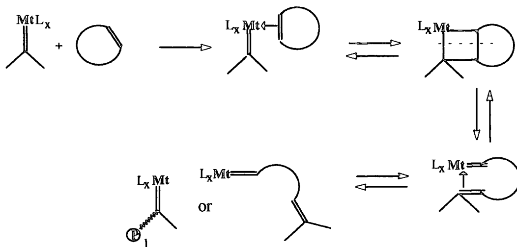
Figure 1.4.a Ring opening metathesis polymerisation initiation
