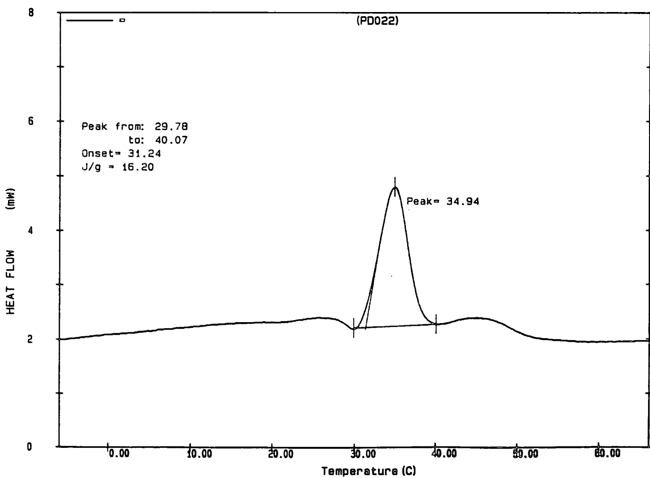
Appendix 2.4.c DSC trace of poly(1-butylene) initiated with \text{Mo}(\text{CH}^t\text{Bu})(\text{OC}(\text{CH}_3)_2\text{CF}_3)_2(\text{NAr})
