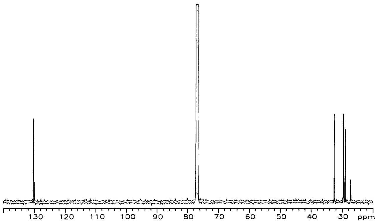
Appendix 2.16.c ^{13}\text{C} -NMR spectrum of poly(1-octenylene) initiated by \text{Mo}(\text{CH}^t\text{Bu})(\text{OC}(\text{CH}_3)_2\text{CF}_3)_2(\text{NAr})
