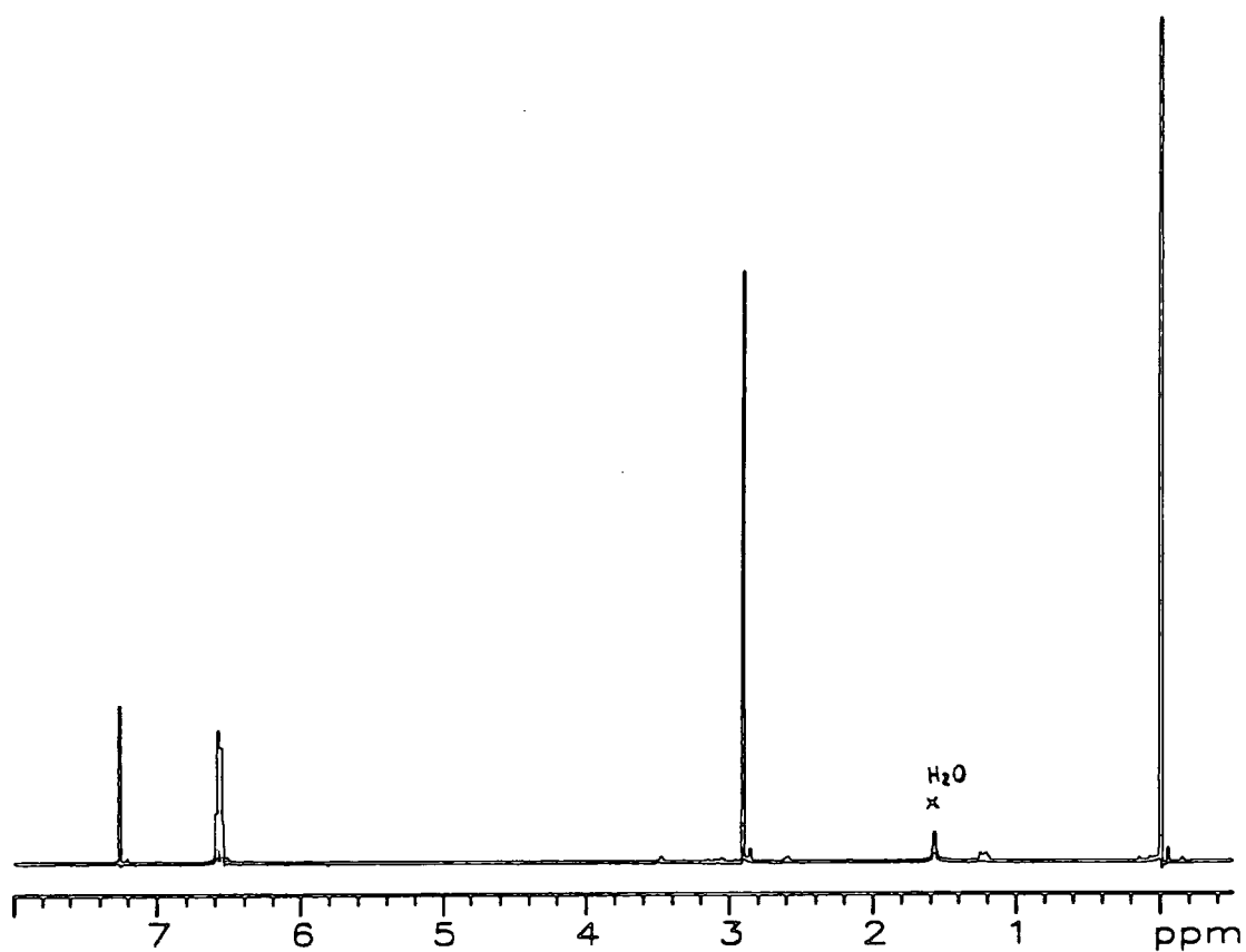
App.5.1 1 H-NMR spectrum of 1,4-cyclohexanedicyclopentadienylidene
