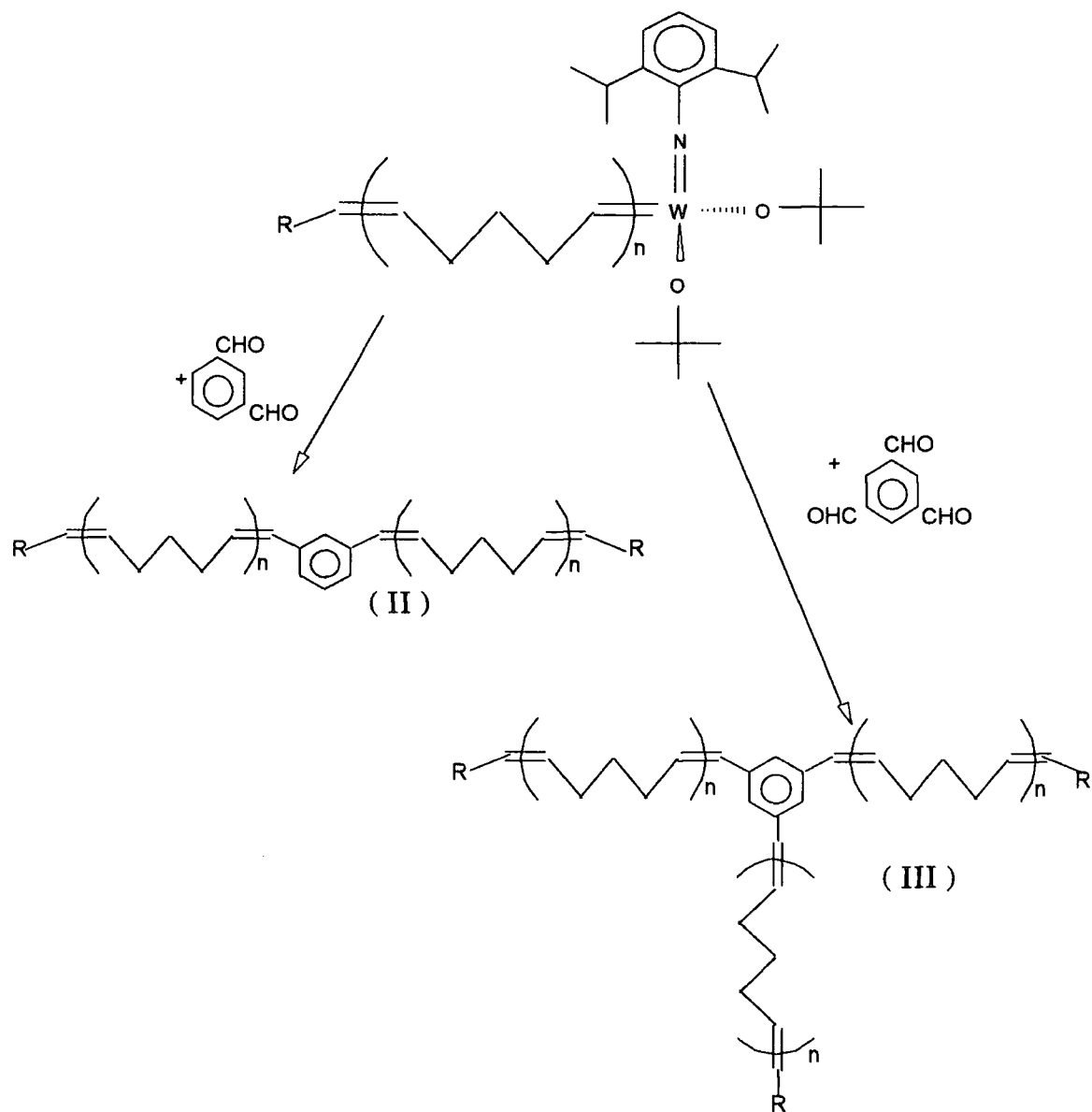
Figure 4.2.a Capping reaction between living poly(1-pentenylene) and multifunctional aromatic aldehydes
