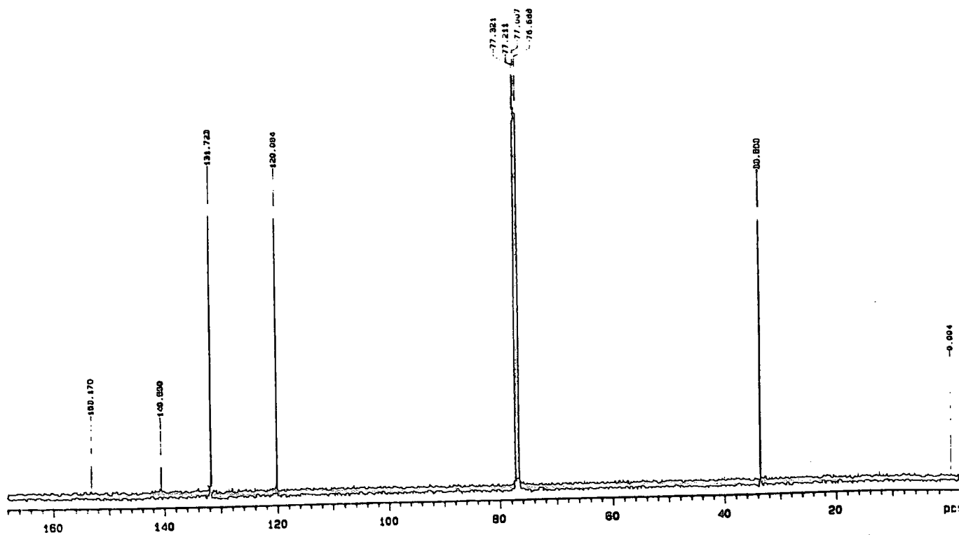
App.5.2 13 C-NMR spectrum of 1,4-cyclohexanedicyclopentadienylidene
