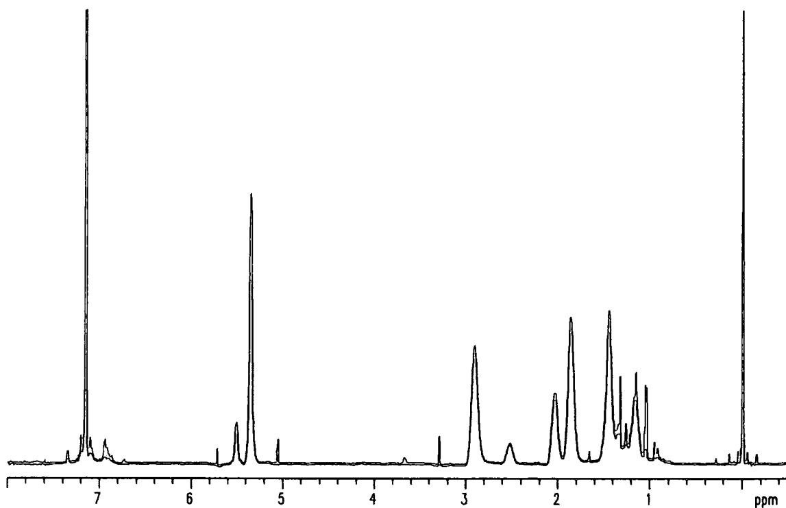
Appendix 5.11 ^1\text{H-NMR} of polynorbornene initiated by \text{Mo}(=\text{C}(\text{CH}_3)\text{Ph})(\text{NAr})(\text{OCCH}_3(\text{CF}_3)_2)_2
