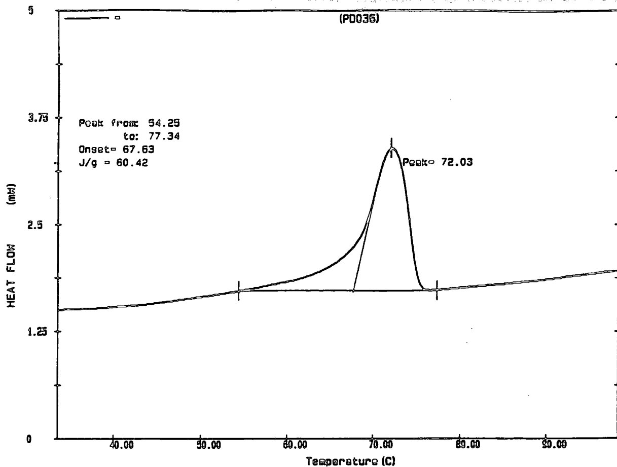
Appendix 2.27.c DSC trace of poly(1-dodecene) initiated with \text{Mo}(\text{CH}^t\text{Bu})(\text{OC}(\text{CH}_3)_2\text{CF}_3)_2(\text{NAr})
