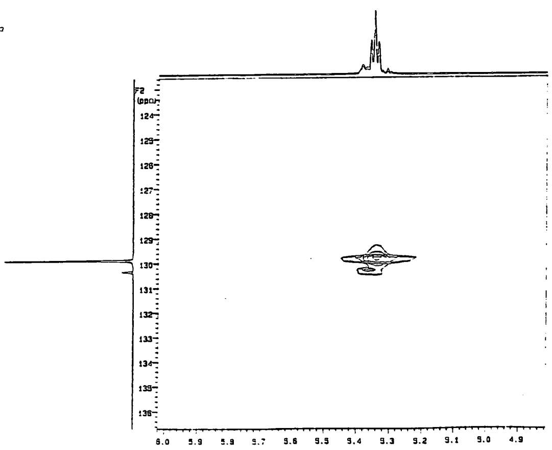
Appendix 2.17 HETCOR spectrum of poly(1-octenylene) initiated with W(CH^tBu)(O^tBu)_2(NAr)
