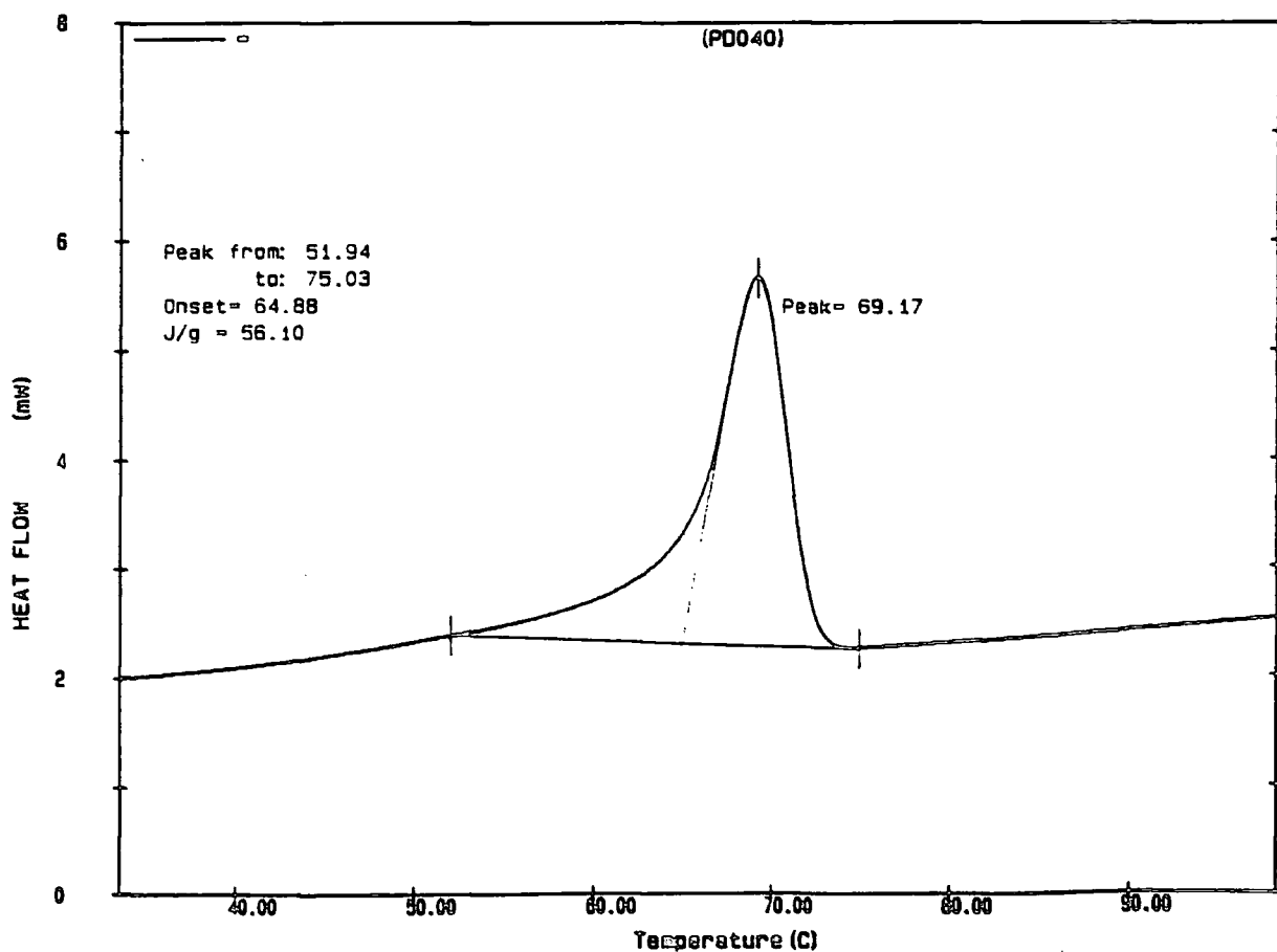
Appendix 2.27.b DSC trace of poly(1-dodecenylene) initiated with Mo(CH^tBu)(OC(CH_3)_3)_2(NAr)
