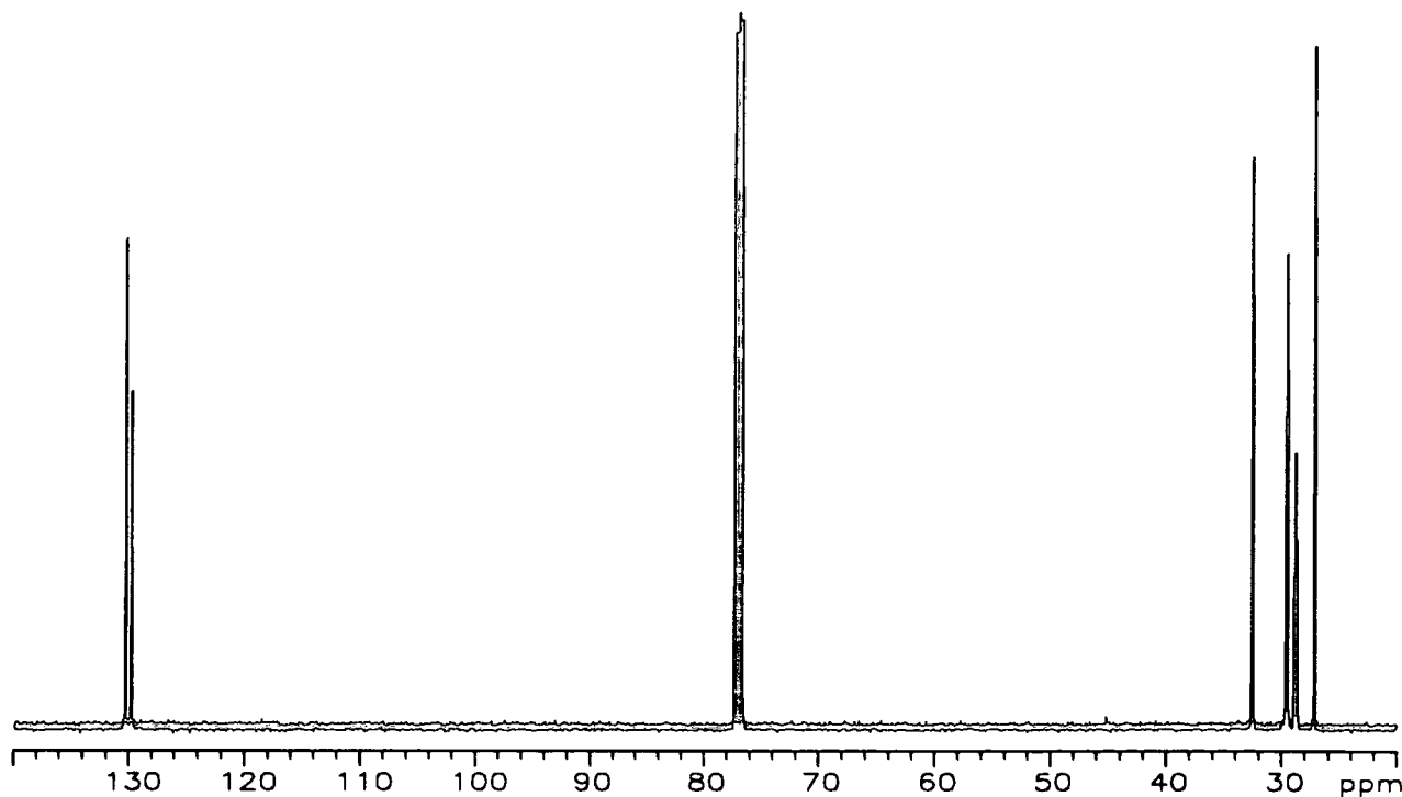
Appendix 2.12.a ^{13}\text{C-NMR} spectrum of poly(1-heptylene) initiated by \text{Mo}(\text{CH}^t\text{Bu})(\text{OC}(\text{CH}_3)_3)_2(\text{NAr})
