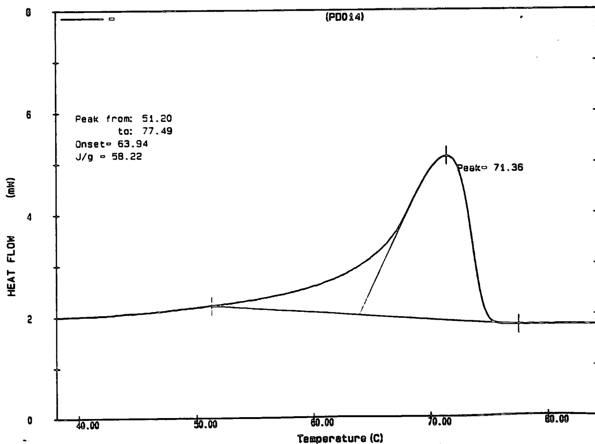
Appendix 2.27.d DSC trace of poly(1-dodecene) initiated with \text{Mo}(\text{CH}^t\text{Bu})(\text{OC}(\text{CH}_3)(\text{CF}_3)_2)_2(\text{NAr})
