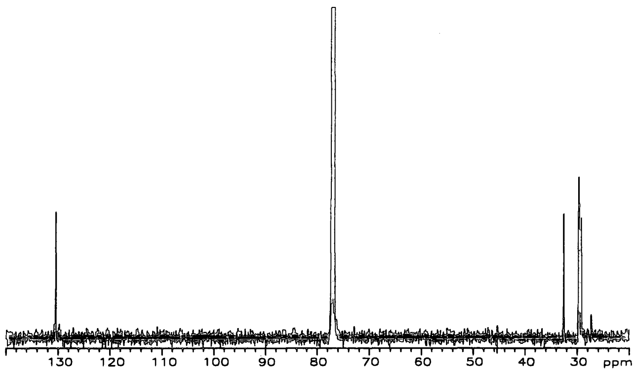
Appendix 2.25.d ^{13}\text{C} -NMR spectrum of poly(1-dodecenylyene) initiated by \text{Mo}(\text{CH}^t\text{Bu})(\text{OC}(\text{CH}_3)(\text{CF}_3)_2)_2(\text{NAr})
