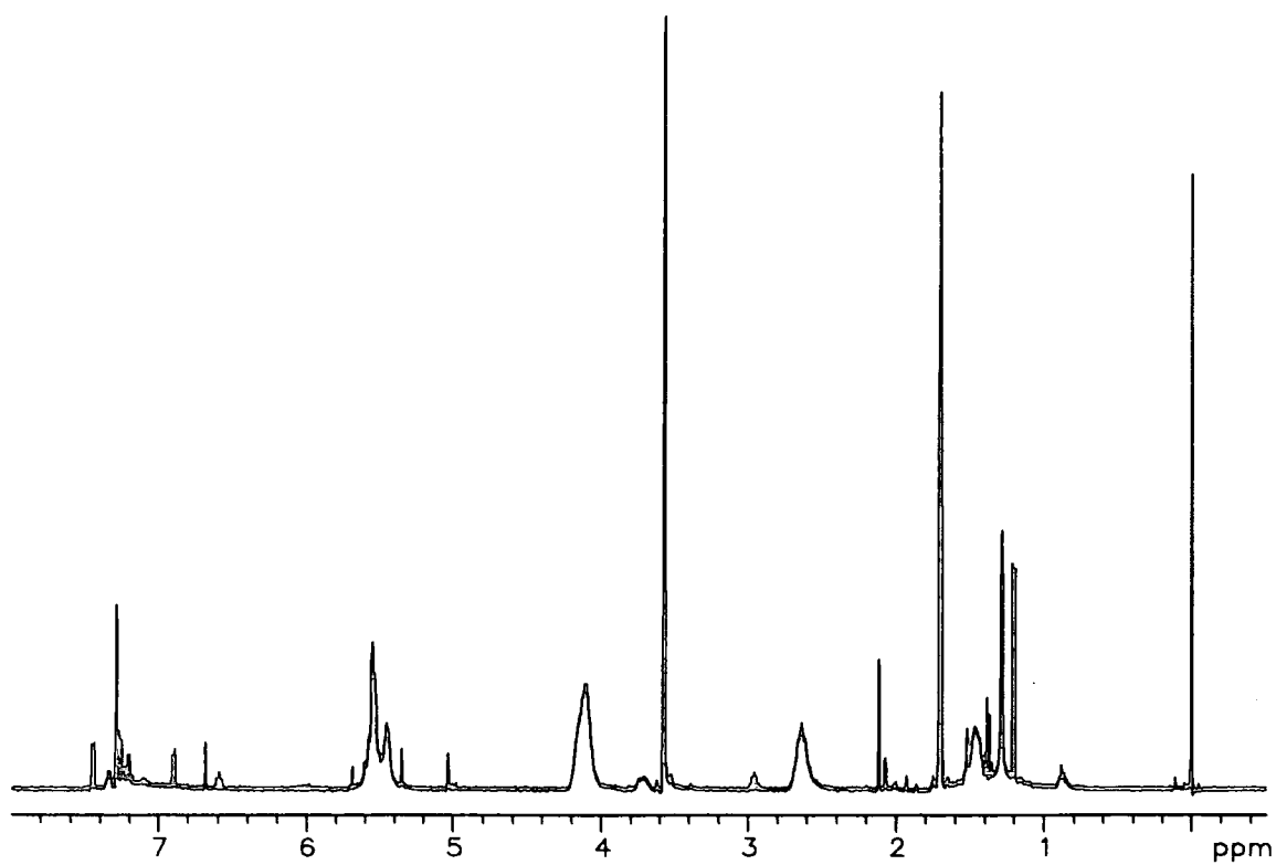
Appendix 5.12 ^1\text{H-NMR} of poly(bistrifluoromethylnorbornadiene) obtained via \text{Mo}(=\text{C}(\text{CH}_3)\text{Ph})(\text{NAr})(\text{OCCH}_3(\text{CF}_3)_2)_2 initiation
