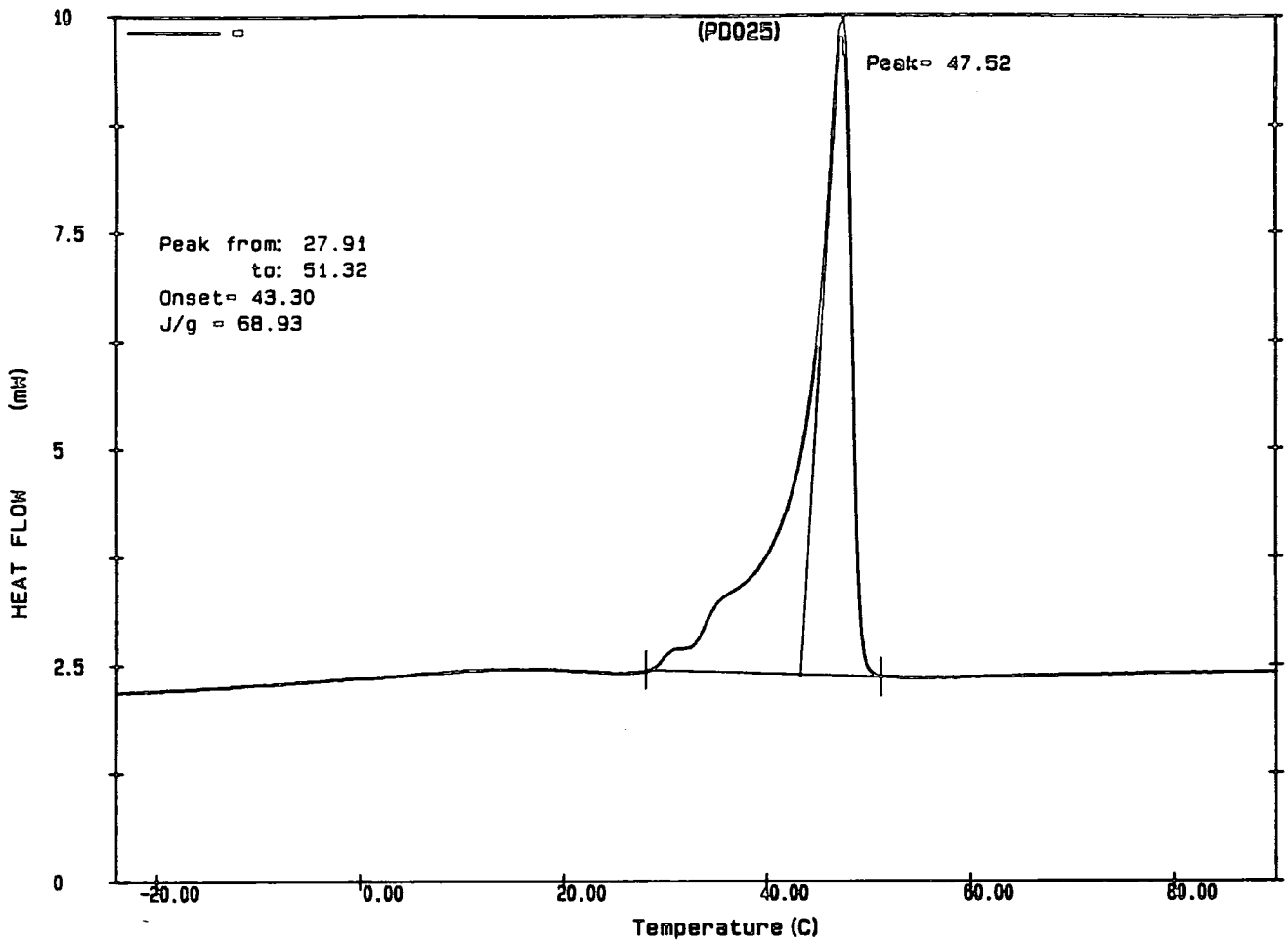
Appendix 2.14.c DSC trace of poly(1-heptenylene) initiated with \text{Mo}(\text{CH}^t\text{Bu})(\text{OC}(\text{CH}_3)(\text{CF}_3)_2)_2(\text{NAr})
