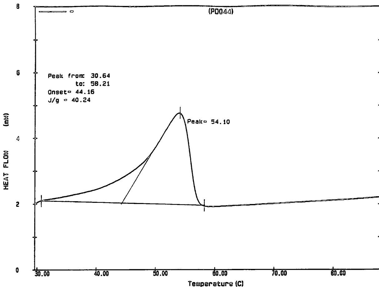
Appendix 2.19.c DSC trace of poly(1-octenylene) initiated with \text{Mo}(\text{CH}^t\text{Bu})(\text{OC}(\text{CH}_3)_2\text{CF}_3)_2(\text{NAr})
