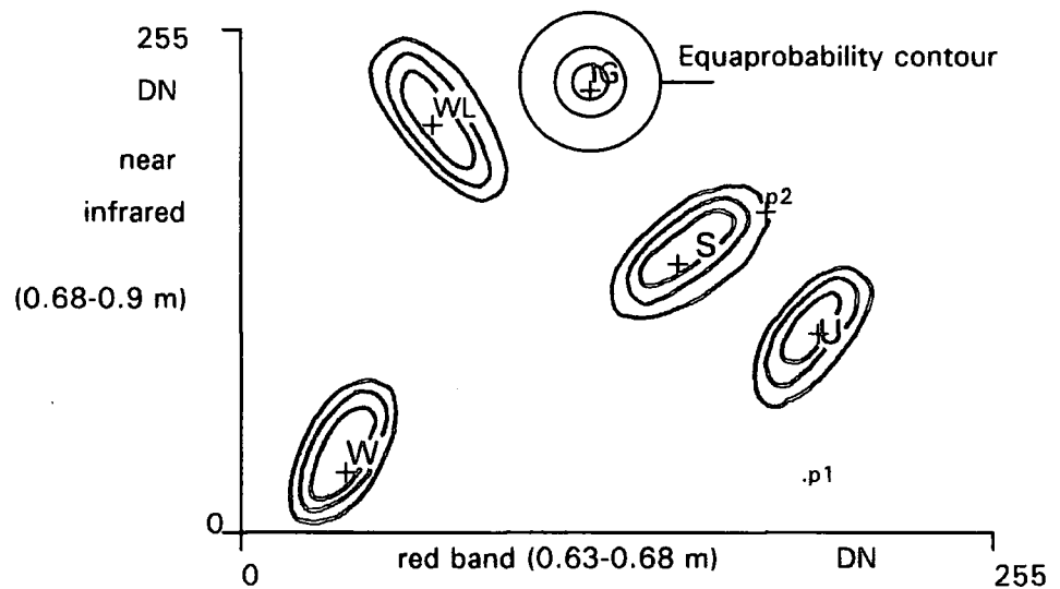
Figure (4:1): Principle of the Maximum Likelihood Classifier
