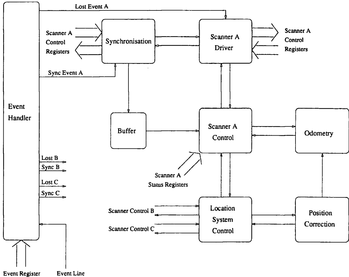
Figure 2.13: Location System Control Processes
