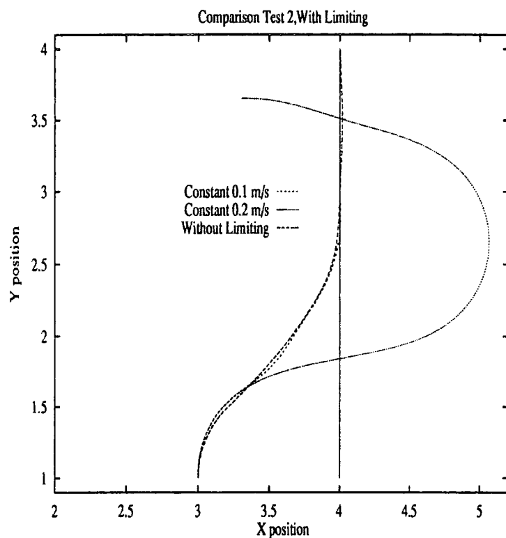
Figure 4.25: Path for Test 2, Showing Velocity Effects.
