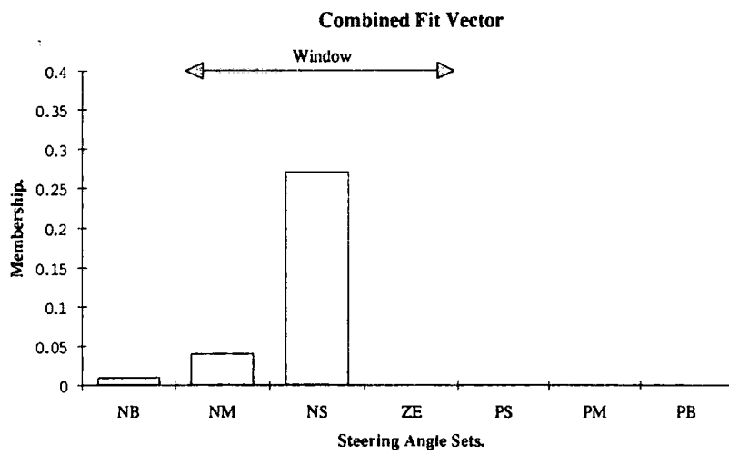
Figure 5.20: Fuzzy Fit and Mask Vectors for Position 3.
