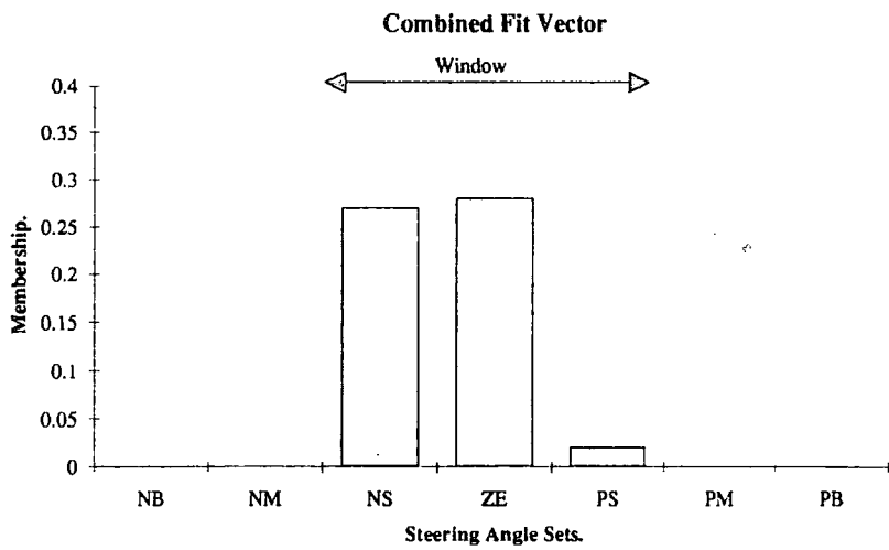
Figure 5.18: Fuzzy Fit and Mask Vectors for Position 1.
