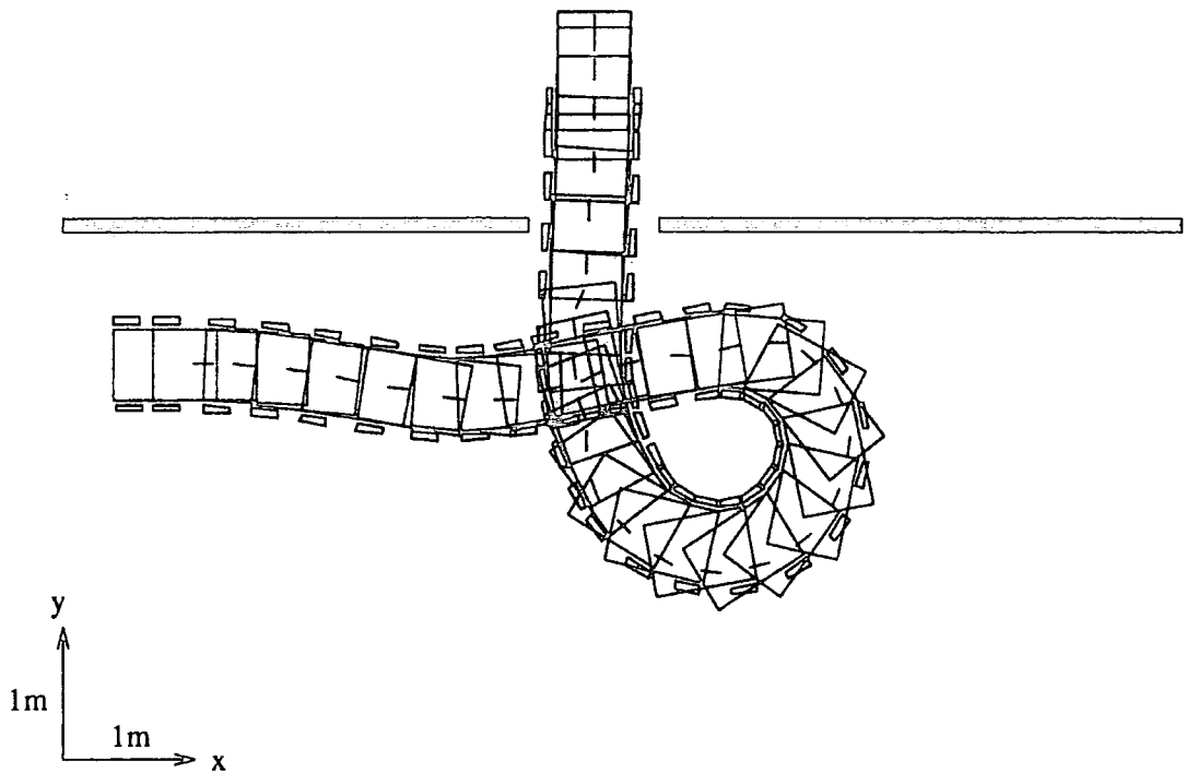
Figure 7.6: Vehicle Faced with a Narrow (1m) Gap, Goal Aligned With Gap.
