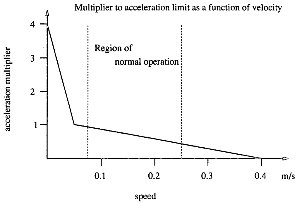
Figure 2.10: Limits Placed upon the Vehicle's Acceleration.
