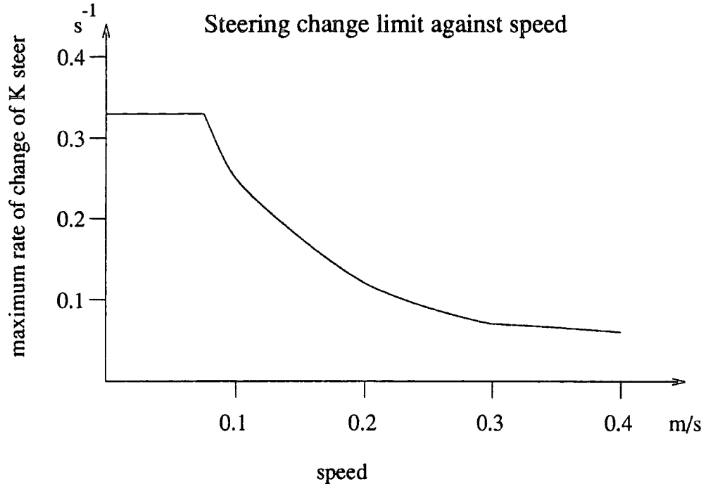
Figure 2.9: Maximum Rate of Change of Steering Constant Against Speed.
