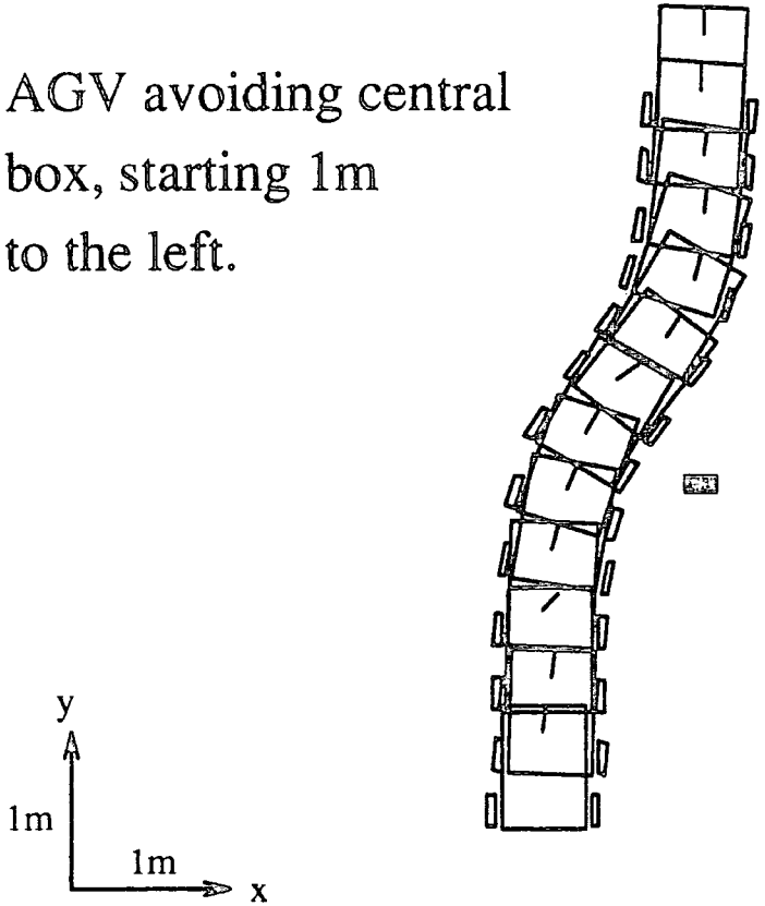
Figure 5.15: Vehicle in Laboratory Test Avoiding a Central Box, Starting 1m to Left.
