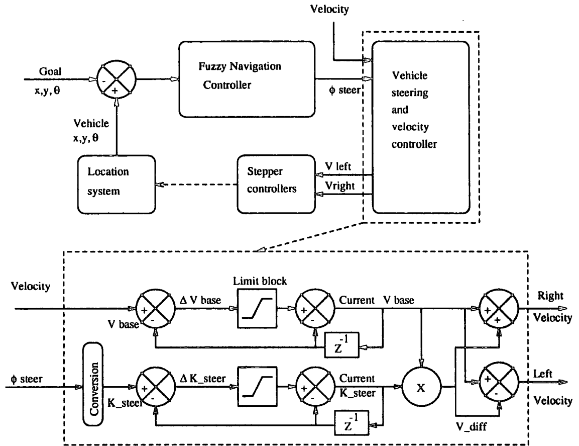
Figure 4.22: Vehicle Control Loop, Illustrating Rate Limiting Block.
