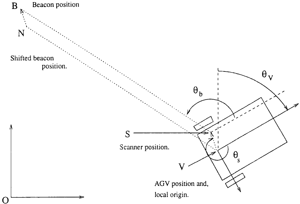
Figure B.5: Illustration of Correction Made for Scanner Position.
