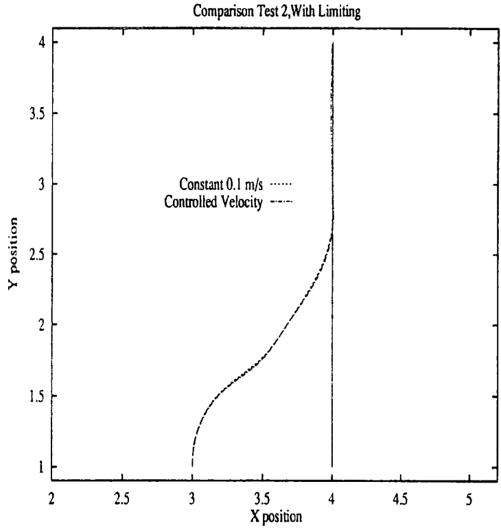
Figure 4.33: Path for Test 2, Using Velocity Control.
