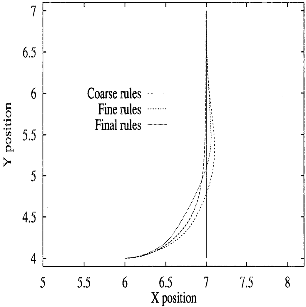
Figure 4.11: Path for Test 1, without Windowing and Rule Spreading.
