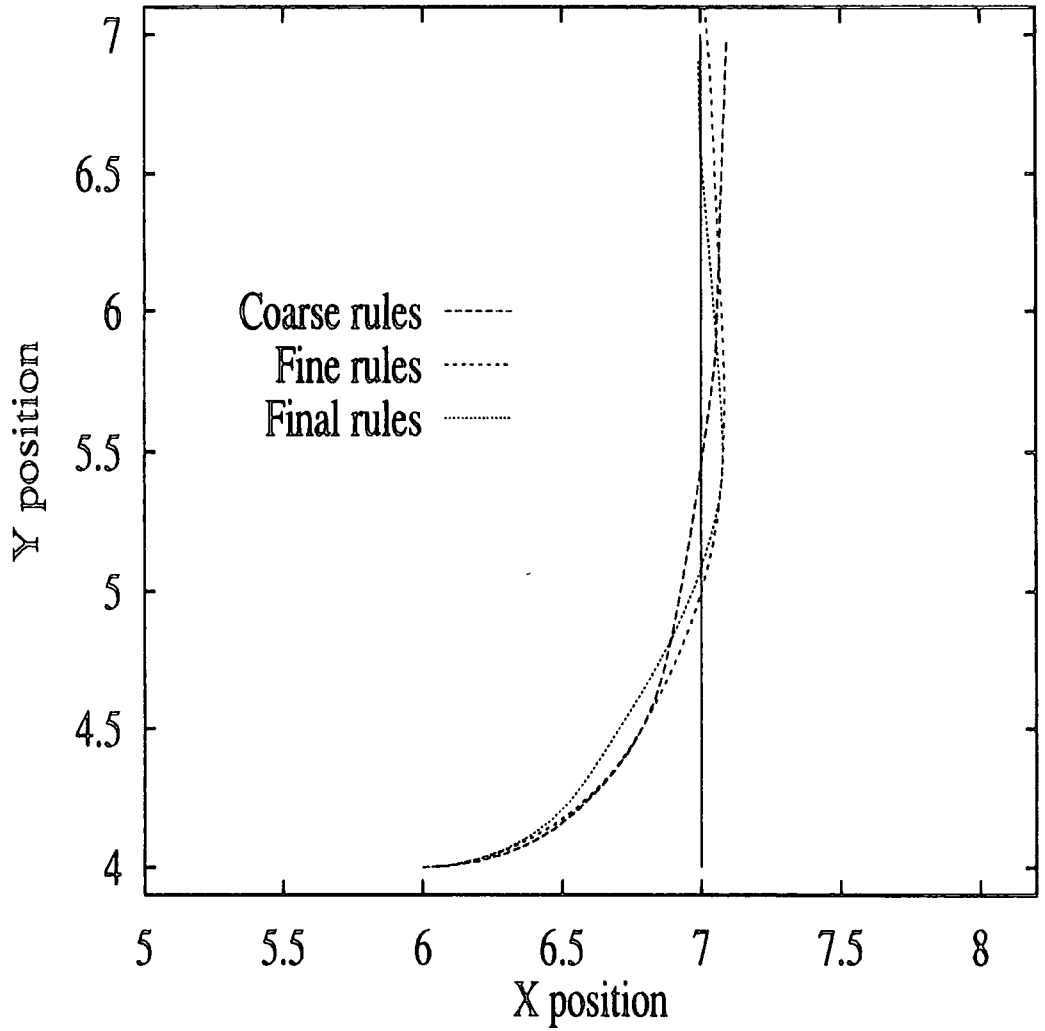
Figure 4.13: Path for Test 1, using Windowing and Rule Spreading.
