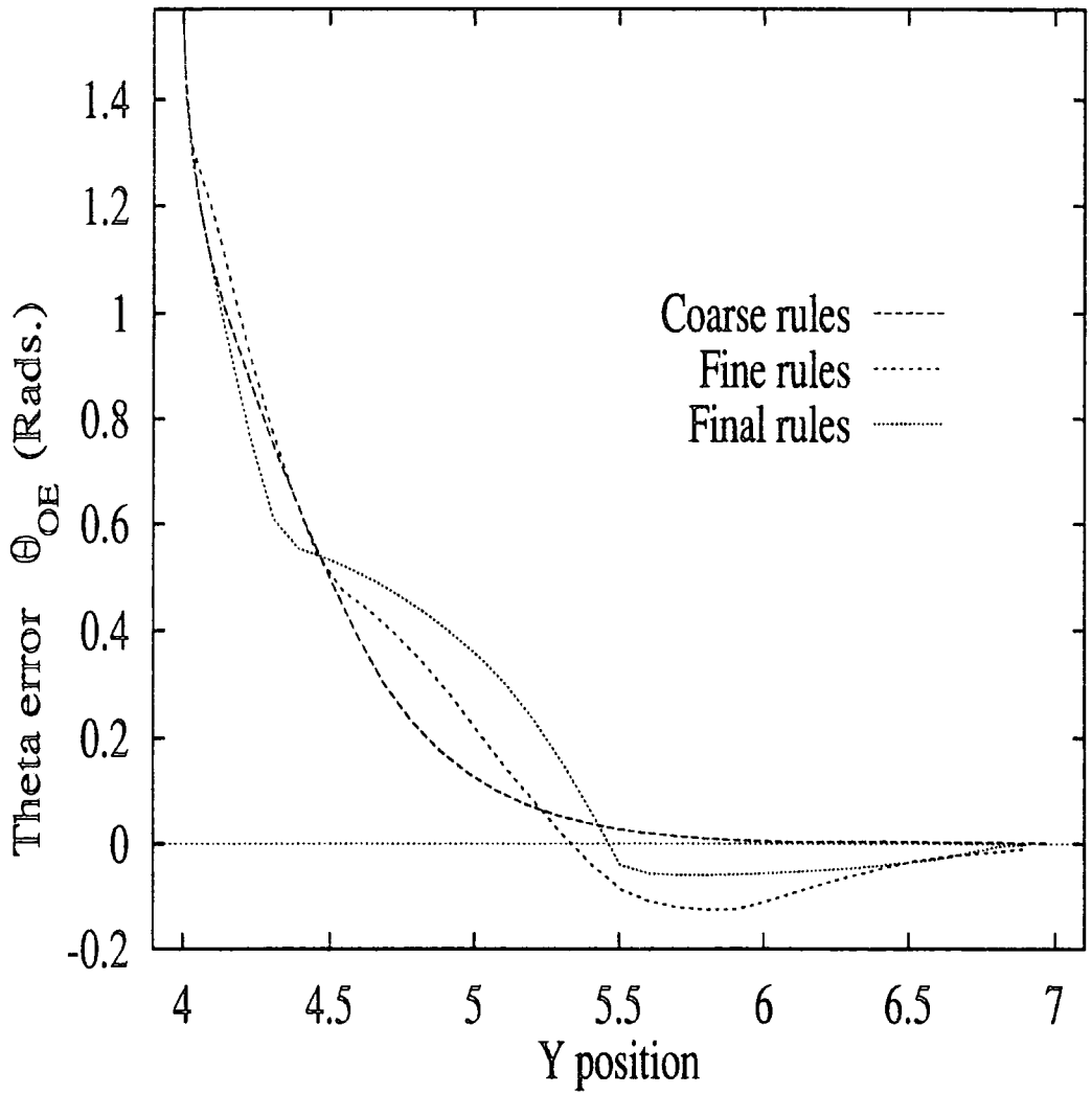
Figure 4.12: Angle Error During Test 1, without Windowing and Rule Spreading.
