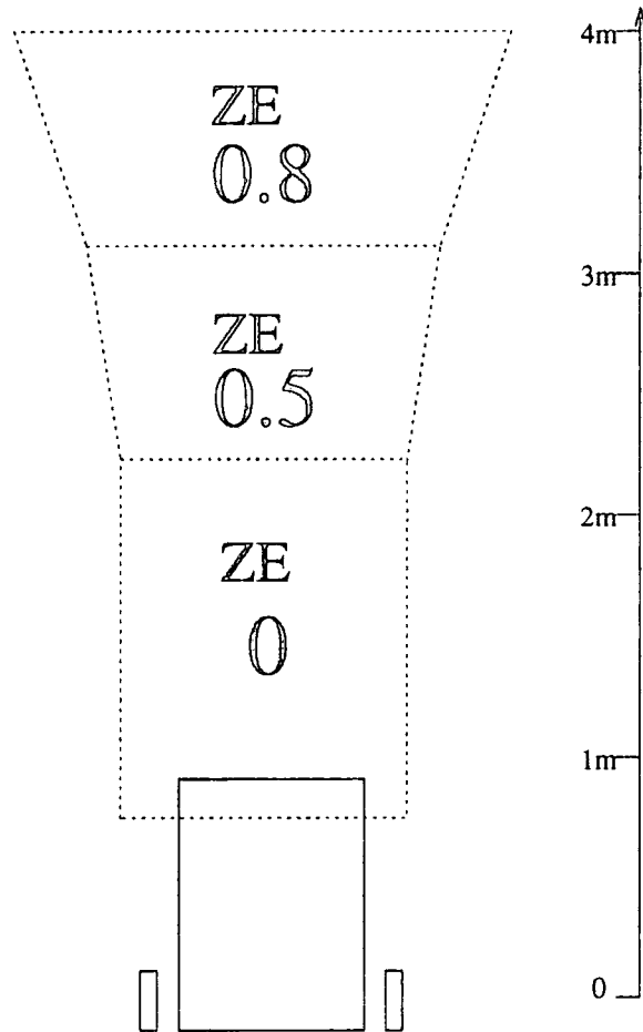
Figure 5.3: Avoidance Set Areas for 'Zero' Steering Angle.
