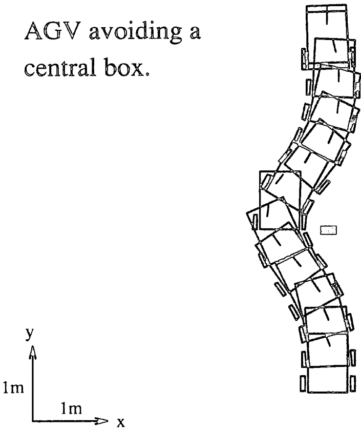
Figure 5.14: Vehicle in Laboratory Test Avoiding a Central Box.
