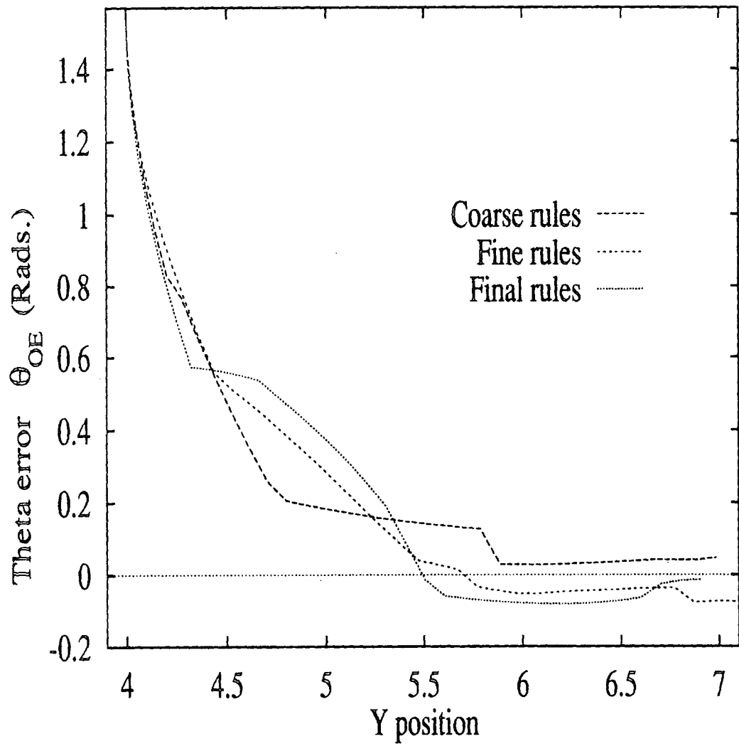
Figure 4.14: Angle Error During Test 1, using Windowing and Rule Spreading.
