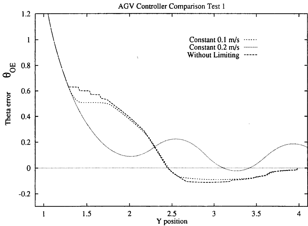
Figure 4.24: Angle Error During Test 1, Showing Velocity Effects.
