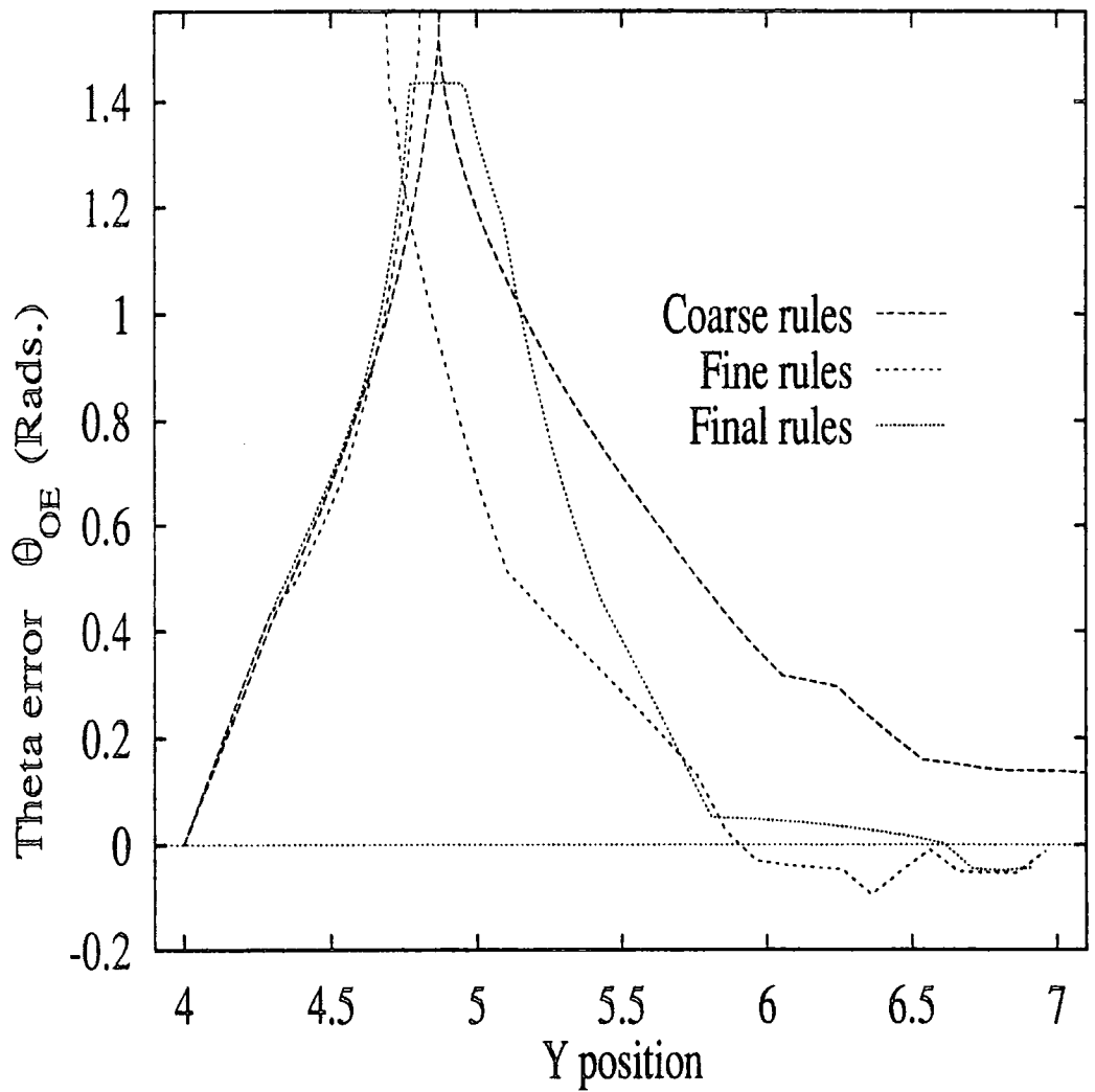
Figure 4.18: Angle Error During Test 3.
