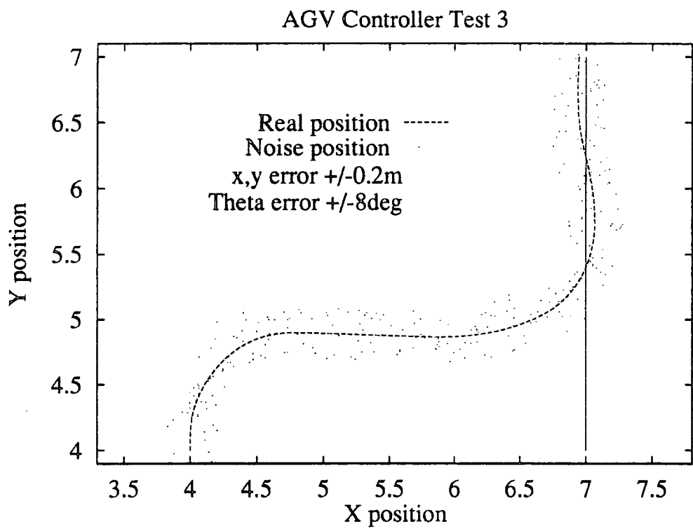
Figure 4.36: Path for Test 3, High Level Noise.
