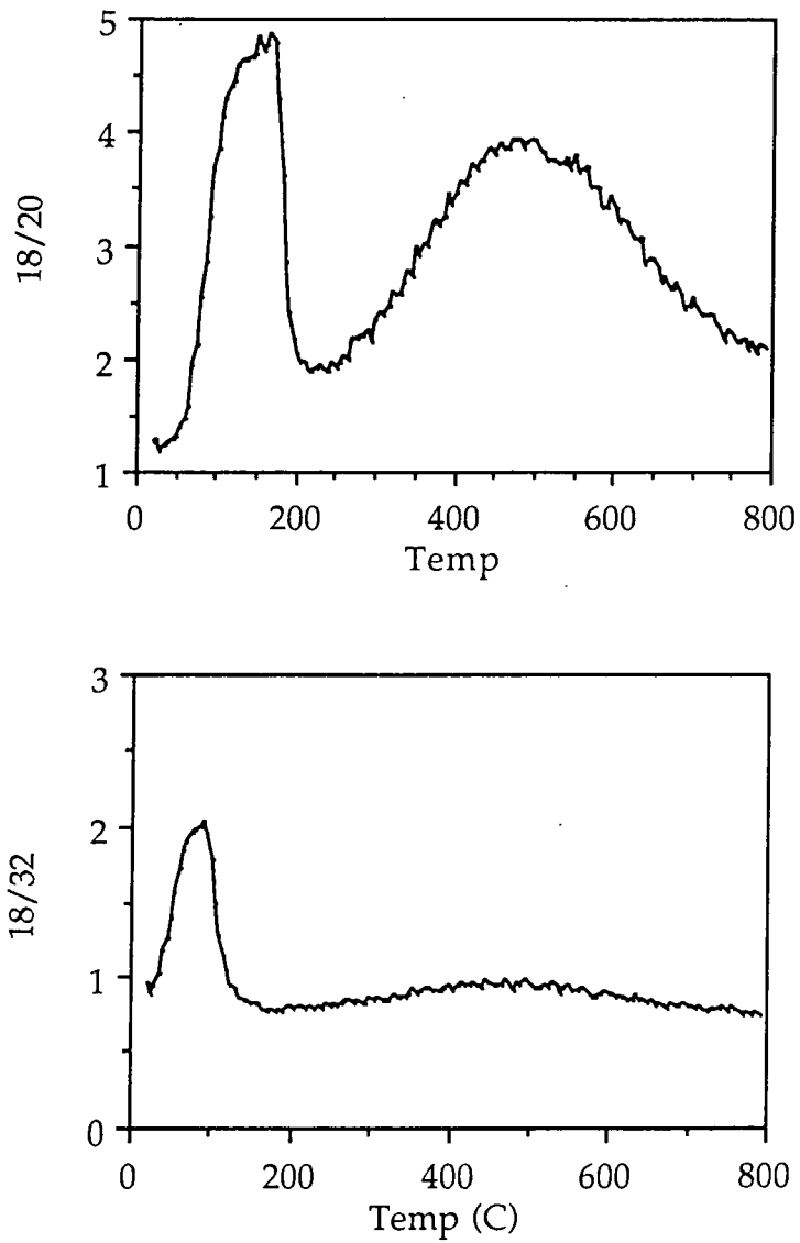
Figure 5.10 Comparison of the water loss profiles for silica. (Top: Under Ar, Bottom: Under O_2 ).
