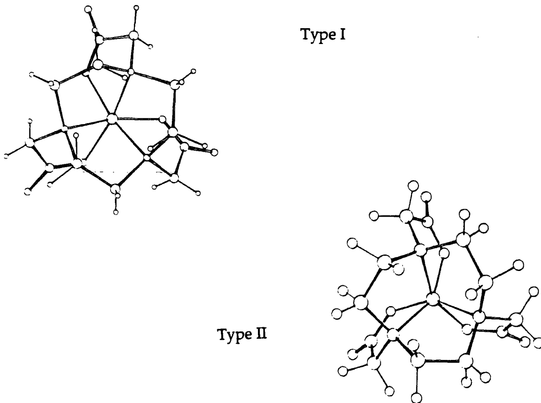
Figure 1.5 Structure of complexes with type I [Ni (II)] and II [Fe (III)] structures.
