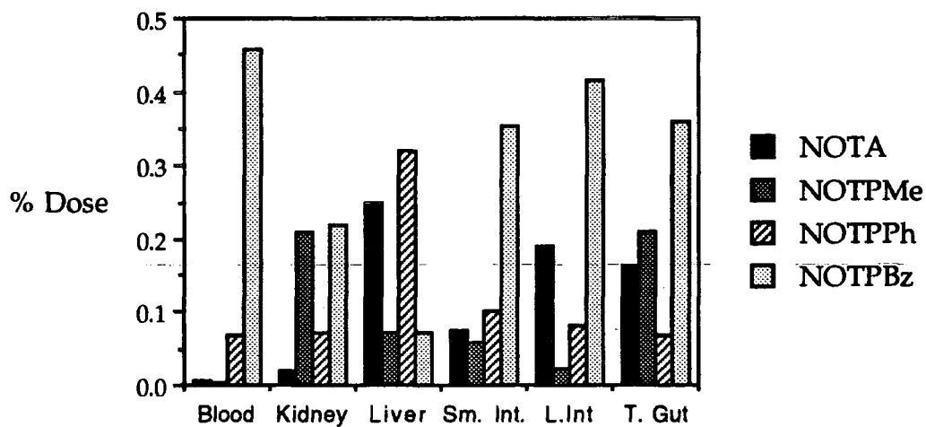
Figure 3.25 Plot of distribution of Ga complex after 1 hour.
