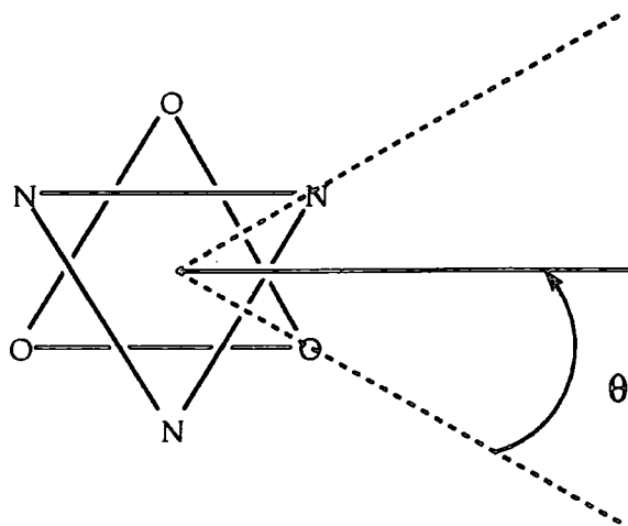
Figure 3.7 Defining the angle referred to as the twist angle.
