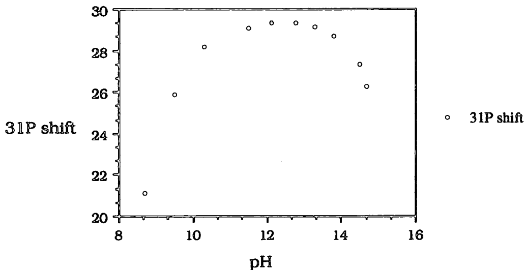
Figure 2.1 Plot of pH versus 31 P shift for DPP.
