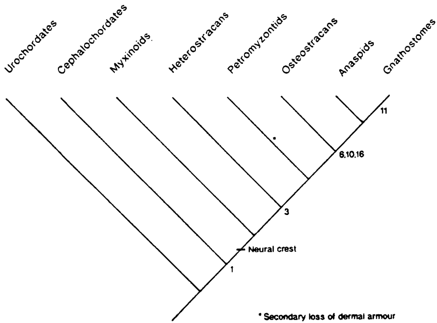
TEXT-FIG. 6.23. Cladogram showing the phylogenetic interrelationships of the chordates presented by Maisey (1988, figs 1-3). Numbers indicate the stated distribution of the character states utilised in this study (Text-fig. 6.17).
