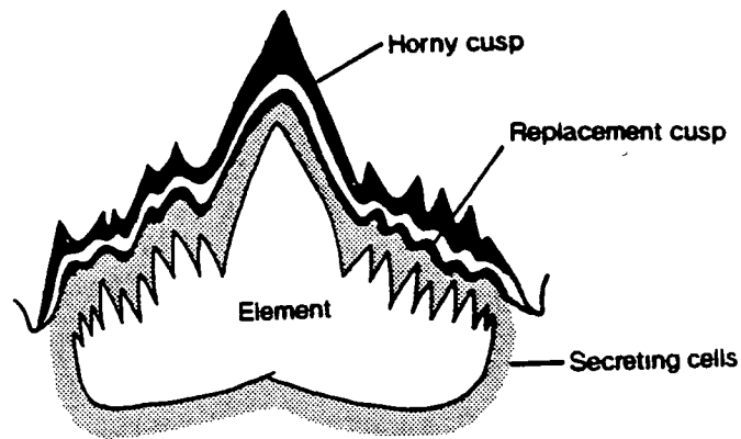
TEXT-FIG. 4.3. An ozarkodinid Pb element acting as an internal support for a 'horny' (presumably keratinous) cusp, presumably homologous with myxinoid lingual denticles (Modified from Priddle 1974, fig. 2).
