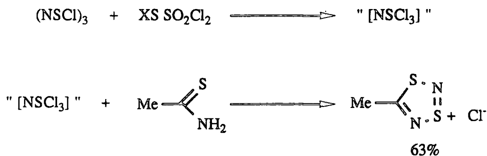
Scheme 1.2.7 Preparation of 1,3,2,4-Dithiadiazolium Chlorides from (NSCl) 3 , SO 2 Cl 2 and Thioamides
