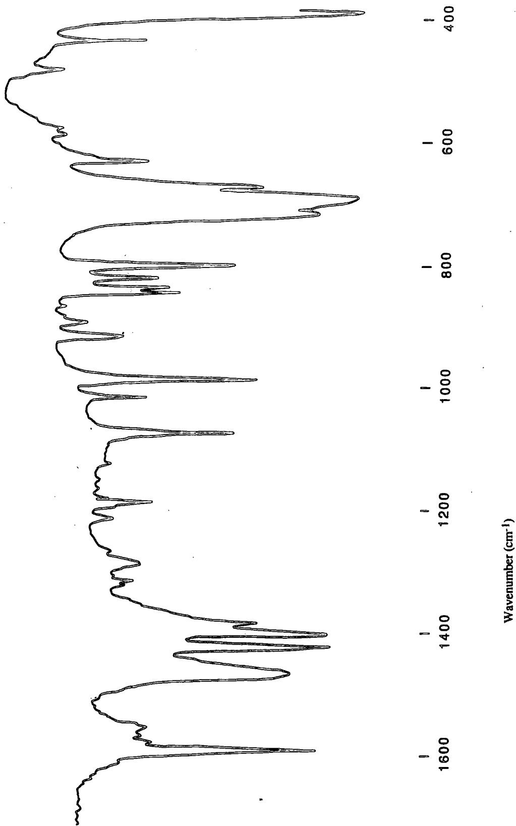
Fig. 3.2.4 IR spectrum (Nujol mull) of [p-Br-C 6 H 4 -CNSNS][AsF 6 ] 9
