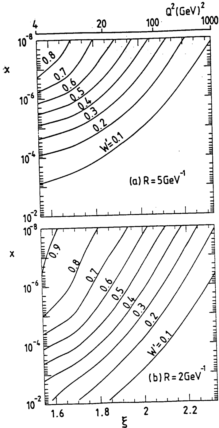
Figure 6.10. Contour plots of constant W' in the (y, \xi) plane, where y = \ln(1/x) and \xi = \ln(\ln(Q^2)) , obtained from solving the (exact) Lipatov equation with shadowing included with (a) R = 5 \text{ GeV}^{-1} and (b) R = 2 \text{ GeV}^{-1} , as described in the text. The leading-order shadowing approximation should be valid in the domain satisfying W' \lesssim \alpha_s(Q^2) .
