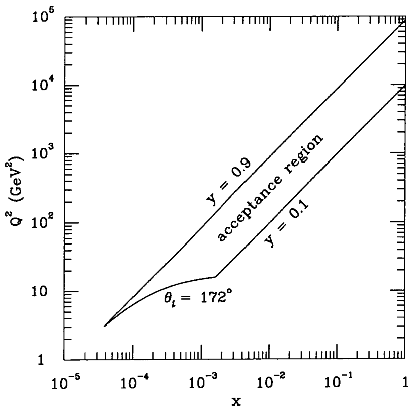
Figure 8.2. The accessible (x, Q^2) range at HERA in which accurate x and Q^2 reconstruction is possible from only lepton scattering measurements.
