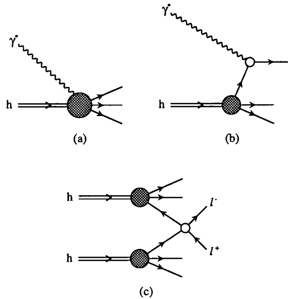
Figure 1.1. a) A diagrammatic representation of a virtual photon, \gamma^* , interacting with a hadron. b) In QCD the interaction ‘factorises’ into a hard scattering part (represented by the upper blob) and a soft part (shown shaded). The hard scattering process is independent of the hadron, h , in which the parton involved in the hard scattering, was travelling. Likewise, the soft part is independent of the hard scattering interaction. As a result, the soft part is the same for processes such as (c) the production of leptons via parton-parton annihilation.
