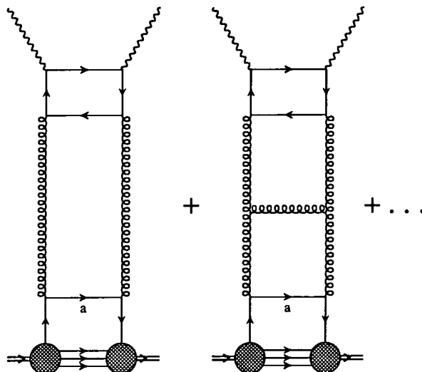
Figure 7.3. The leading \ln(x_j/x) approximation to the process shown in Fig. 7.2.
