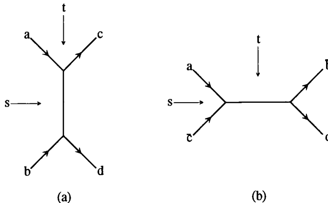
Figure 5.1. (a) The s -channel diagram relevant to the scattering ab \rightarrow cd via particle exchange in the t -channel. Each exchanged particle has q^2 < 0 and so can never come close to its mass shell condition q^2 = m^2 . Crossing s and t leads to the process a\bar{c} \rightarrow \bar{b}d , shown in (b), in which the exchange particles now exist in the s -channel with q^2 > 0 . We expect that the scattering amplitude for process (b) will contain poles when q^2 \simeq m^2 and we can therefore approximate the scattering amplitude by the sum of these poles. The relationship between the scattering amplitude for (b) and the scattering amplitude for (a) is given by Regge theory.
