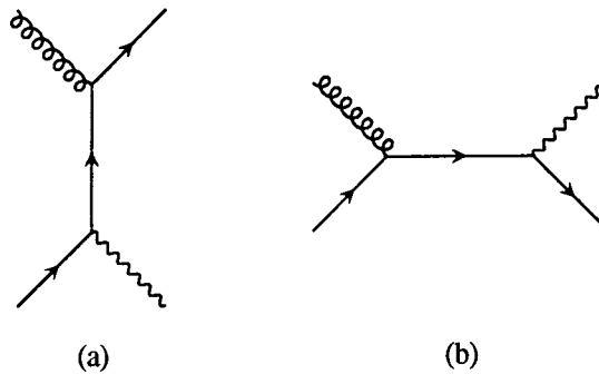
Figure 3.3. Compton graph contributions to the O(\alpha_s) corrections to the Drell-Yan process.
