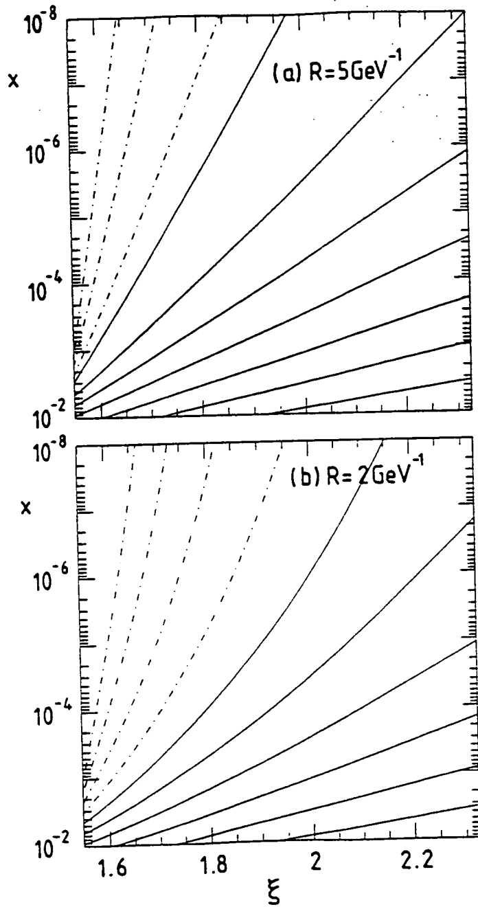
Figure 6.8. The characteristic curves, y(\xi) , obtained by solving the semi-classical equations 6.23 and 6.24-6.27 using the gluon distribution of Fig. 6.7 at Q^2 = 4 \text{ GeV}^2 as input, where \xi = \ln(\ln(Q^2)) and y = \ln(1/x) . We show the families of characteristics for (a) the conventional choice of the shadowing radius, R = 5 \text{ GeV}^{-1} , and (b) "hot-spot" shadowing with R = 2 \text{ GeV}^{-1} . The dot-dashed curves correspond to characteristics above the critical line.
