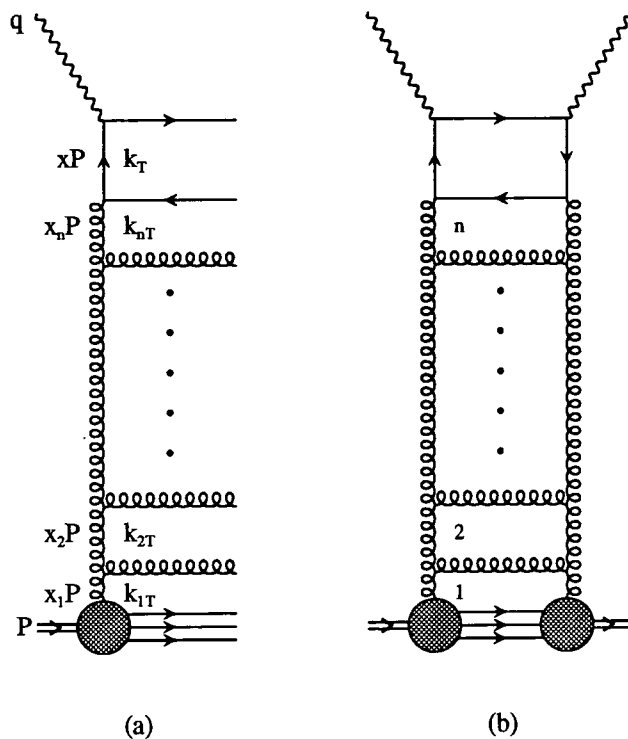
Figure 5.4. Diagrammatic representation for probing the gluon content of the proton at high Q^2 . In the DLLA the transverse ( k_{iT} ) and longitudinal ( x_i P ) are strongly ordered along the chain. On squaring the amplitude of Fig. (a) we generate the ladder diagram of Fig. (b).
