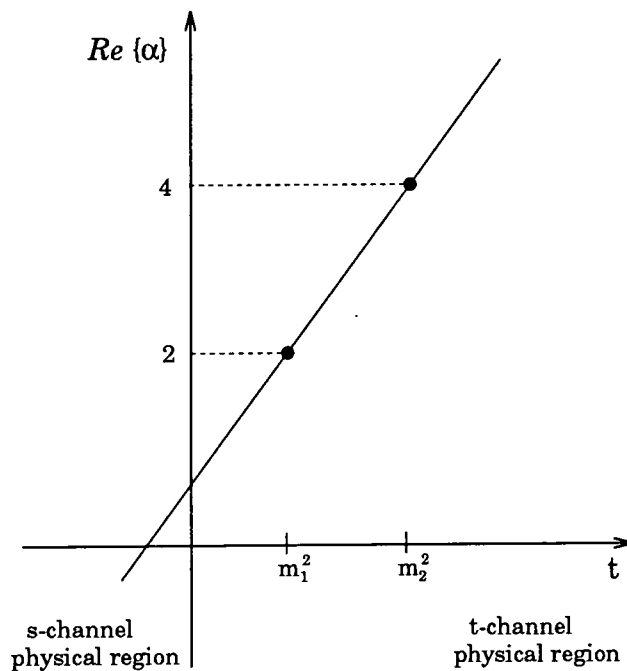
Figure 5.2. A typical Regge trajectory. This trajectory connects a particle of mass m_1^2 and spin 2 with a particle of mass m_2^2 and spin 4.
