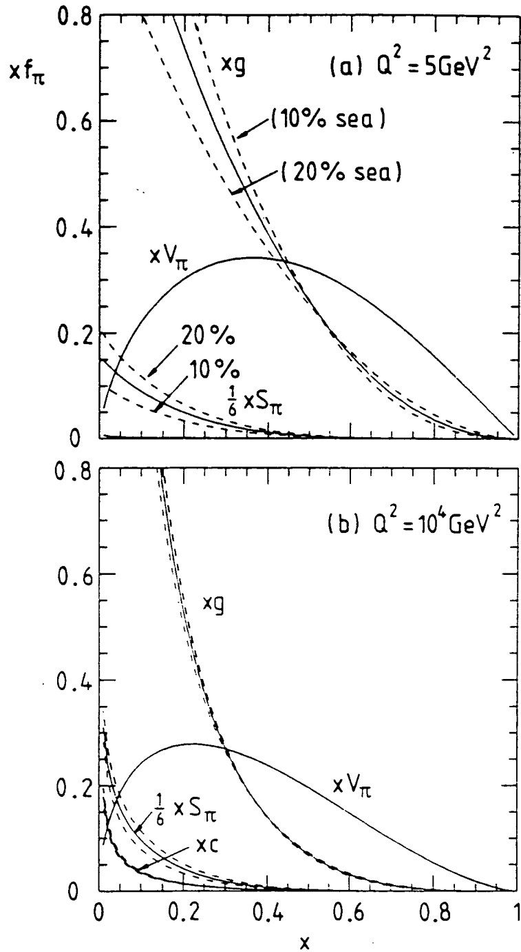
Figure 4.12. The parton distributions of Table 4.8 evolved to (a) Q^2 = 5 \text{ GeV}^2 and (b) Q^2 = 10^4 \text{ GeV}^2 . The set for which the sea quarks carry 15% of the pion's momentum at Q^2 = 4 \text{ GeV}^2 is shown as a solid line, and the remaining two sets, for which the sea quarks carry 10% and 20% of the momentum, as dashed lines. The sea quark distribution is defined as xS_{\pi} = 2x(u + \bar{d} + \bar{s}) ; also shown is the charm quark distribution, x_c = x\bar{c} .
