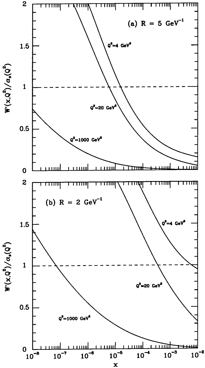
Figure 6.2. The values of W'(x, Q^2)/\alpha_s(Q^2) which correspond to the solutions of the Lipatov equation (6.1) with (a) “weak” ( R = 5 \text{ GeV}^{-1} ) and (b) “strong” ( R = 2 \text{ GeV}^{-1} ) shading. The solutions are only expected to be valid below the dashed line which represents W'(x, Q^2)/\alpha_s(Q^2) = 1 .
