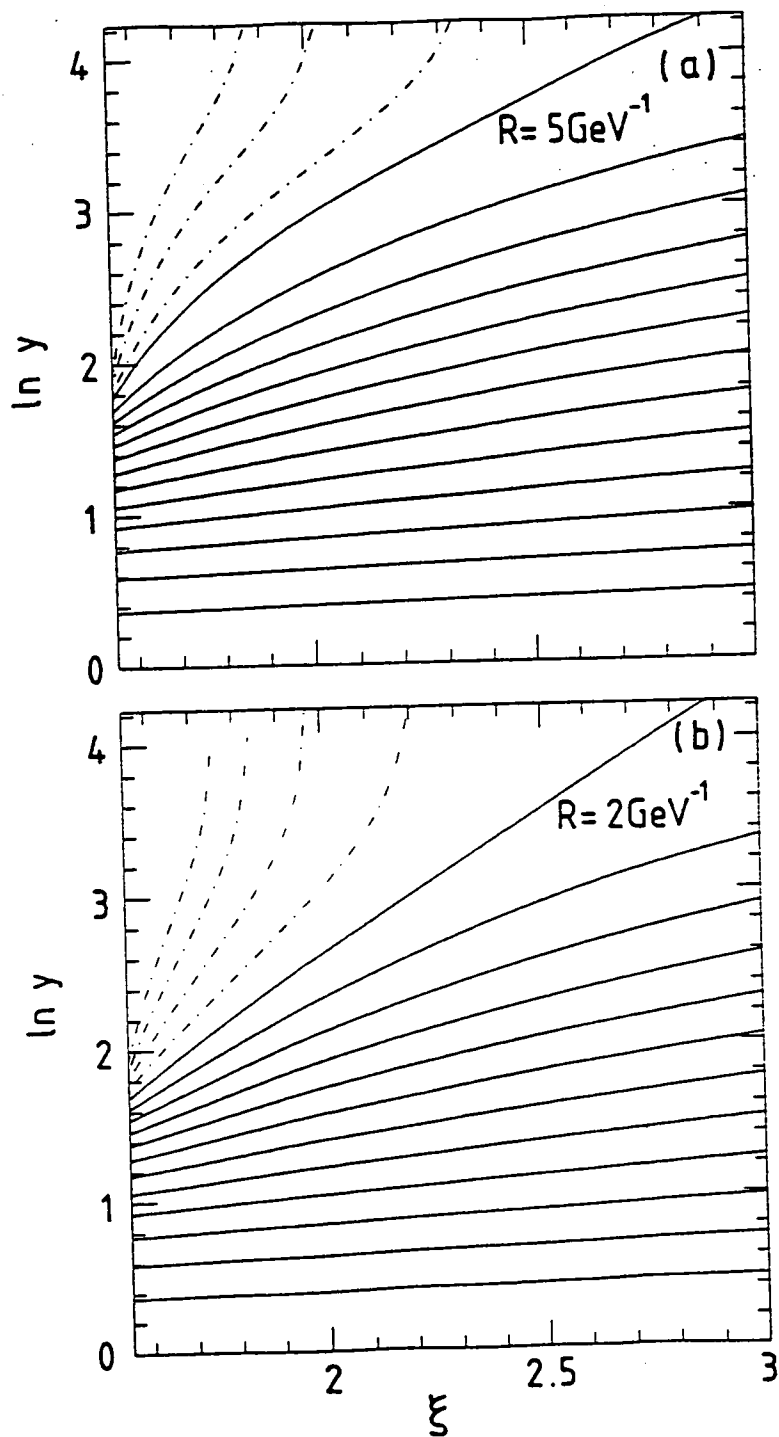
Figure 6.9. The characteristic curves of Fig. 6.8 redrawn on a (\ln y, \xi) plot. On this plot the critical curve behaves at large \xi as a straight line of slope 2, [see Eq. (6.31)]. The dot-dashed characteristic curves above the critical line are now very evident.
