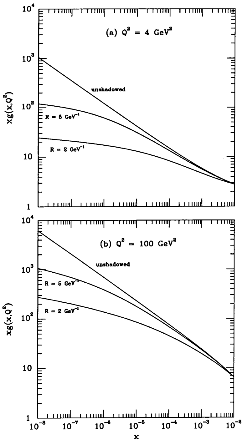
Figure 6.1. The values of xg(x, Q^2) at (a) Q^2 = 4 \text{ GeV}^2 and (b) Q^2 = 100 \text{ GeV}^2 calculated from the solution f(x, k^2) of the integro-differential Lipatov equations [Eqs. (6.1) and (6.3)] with the boundary conditions, f(x_0, k^2) , at x_0 = 10^{-2} fixed as described in the text. In each figure the three curves are, in descending order, the solution with shadowing neglected and the solutions with the shadowing term included with R = 5 \text{ GeV}^{-1} and R = 2 \text{ GeV}^{-1} . The validity of the leading-order shadowing approximation at ultra-small x is studied in Fig. 6.2
