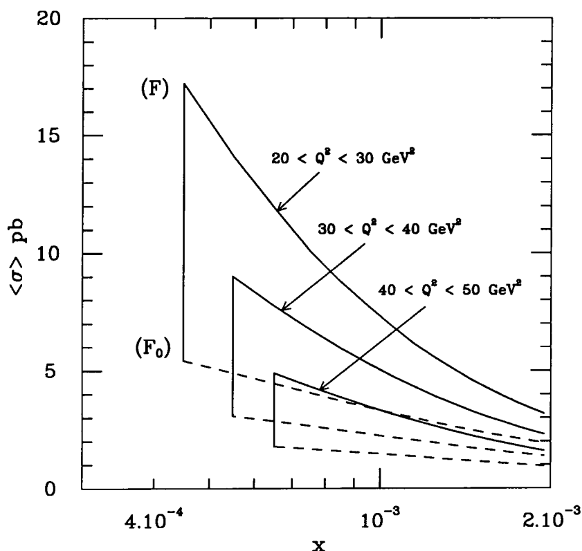
Figure 8.6. The cross section, \langle \sigma \rangle in pb, for deep-inelastic + jet events, integrated over \Delta x = 10^{-4} , \Delta Q^2 = 10 \text{ GeV}^2 bins which are accessible at HERA, and integrated over \theta_j > 5^\circ and x_j > 0.05 , but subject to the constraint \frac{1}{2}Q^2 < k_T^2 < 2Q^2 . The x dependence of \langle \sigma \rangle is shown for three different \Delta Q^2 bins, namely (20,30), (30,40) and (40,50) \text{GeV}^2 . The \langle \sigma \rangle values are plotted at the central x value in each \Delta x bin and joined by straight lines. The continuous curves show \langle \sigma \rangle calculated with the inclusion of the Lipatov soft gluon summation, that is to say with the full F(z, k^2, Q^2) . The corresponding \langle \sigma \rangle values calculated with just the quark box approximation F = F_0 are shown as dashed curves and, for clarity, each is joined with its associated solid curve by a vertical line. The parton distributions used are the B - set of KMRS [50].
