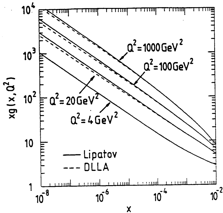
Figure 6.4. A comparison of the Q^2 evolution generated by the Lipatov equation (continuous curves) with that obtained in the DLLA of Eqs. (6.7) and (6.8) (dashed curves)
