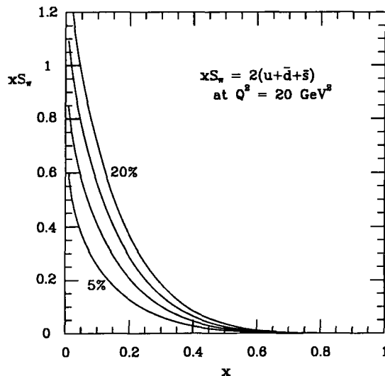
Figure 4.2. The range of sea distributions, xS_\pi = 2x(u + \bar{d} + \bar{s}) , at Q^2 = 20 \text{ GeV}^2 that we include in our fits to the NA10 and E615 Drell-Yan data. The distributions carry 5%, 10%, 15% and 20% of the pion’s momentum at Q^2 = Q_0^2 = 4 \text{ GeV}^2 .
