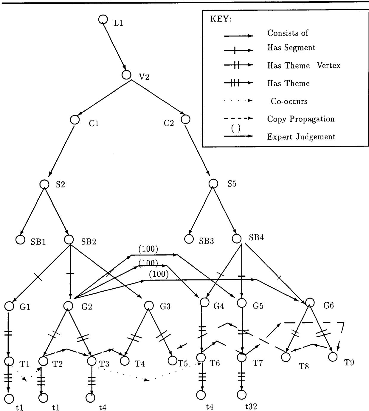
Figure 8.13: Example 2 \delta CIG(\mathcal{V}, \mathcal{E})
