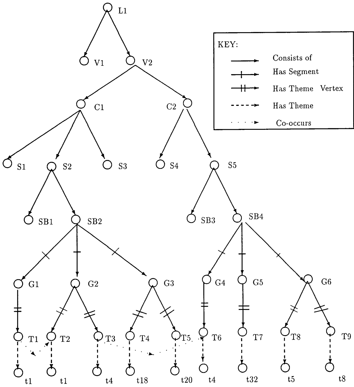
Figure 8.1: RPG(V, \mathcal{E}) Example 1
