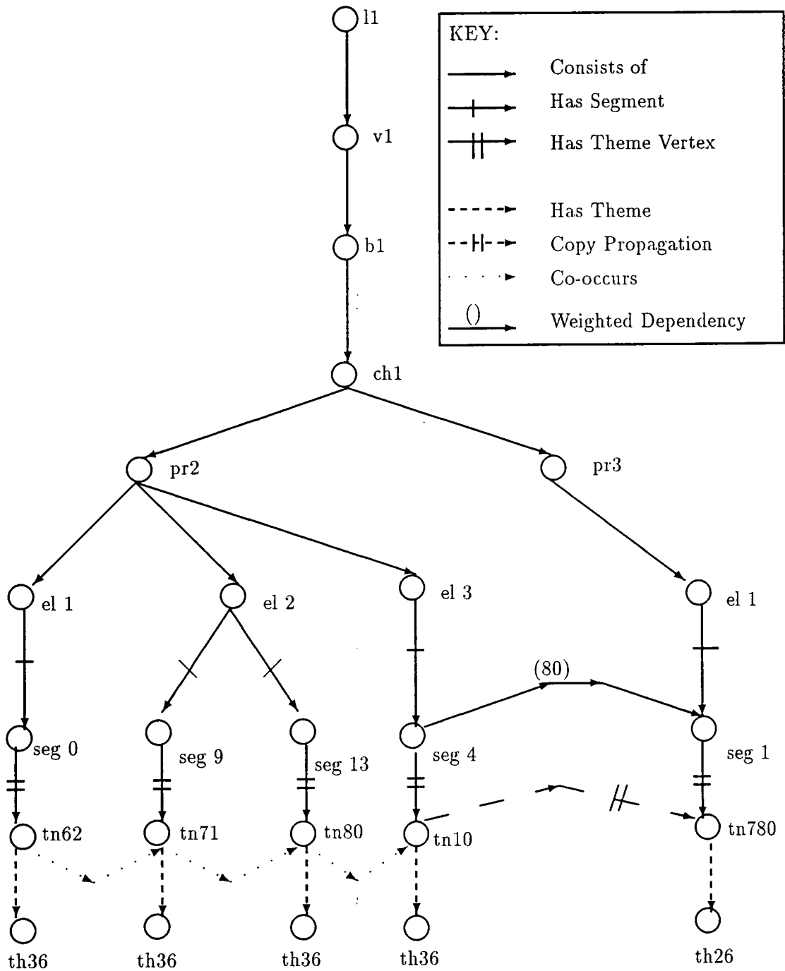
Figure 8.29: Case Study \gamma CIG(V, \mathcal{E})
