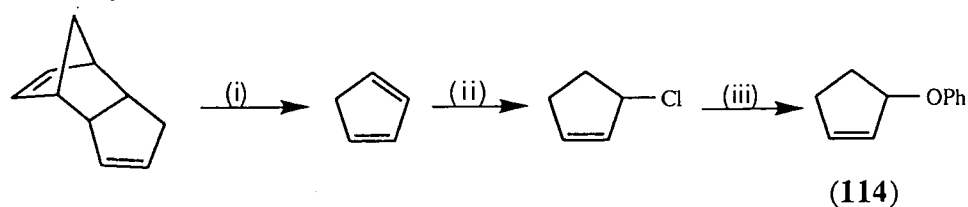
(i) 160°C; (ii) HCl(g), -69°C; (iii) PhOH, NaOH, DMF, H 2 O scheme 2.6
