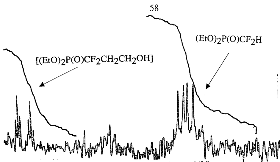
^{19}\text{F} NMR of the reaction between oxirane and (96) figure 2.8
