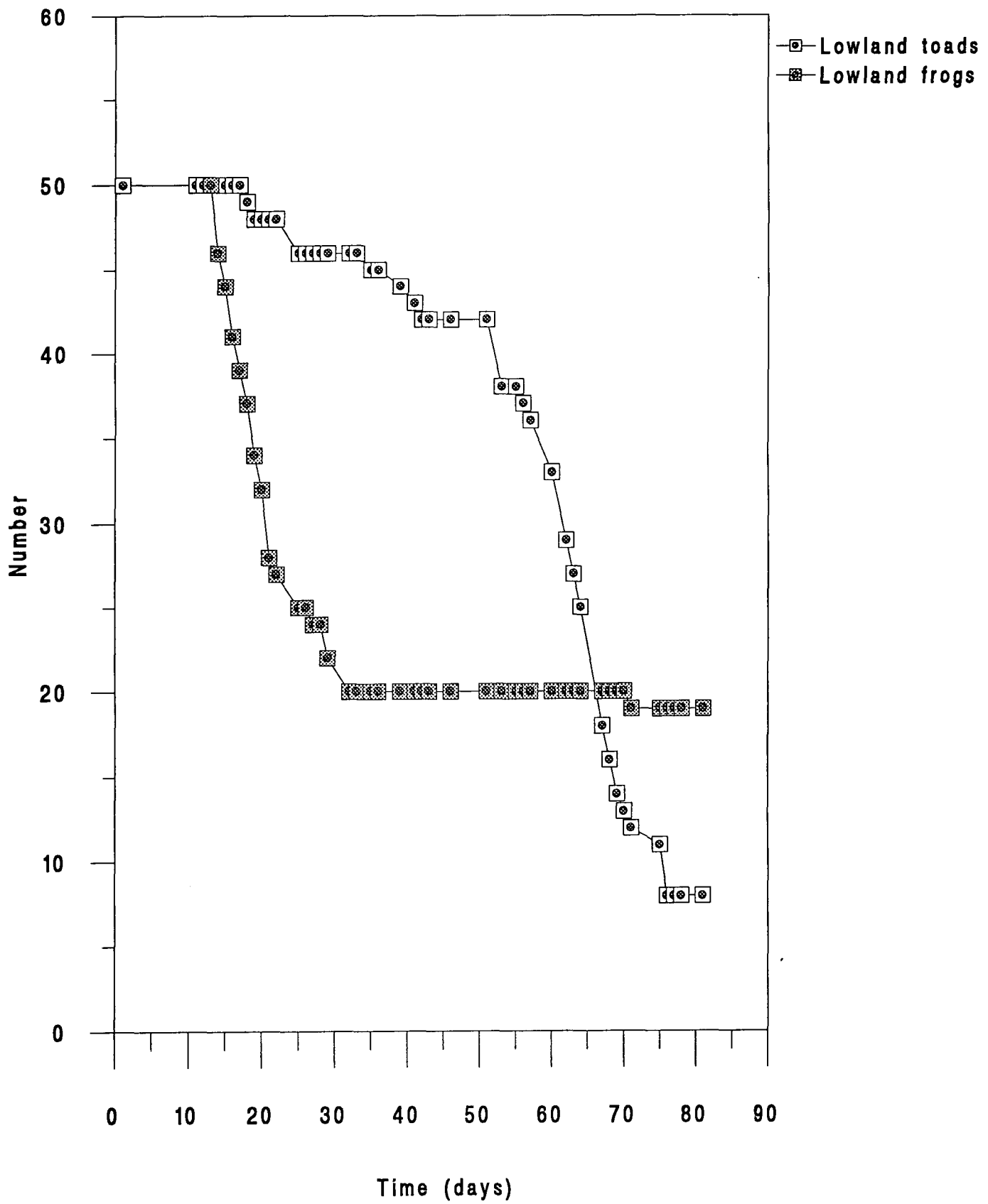
Figure 31. The Survival of Lowland Frogs and Toads at 10 °c With Time
